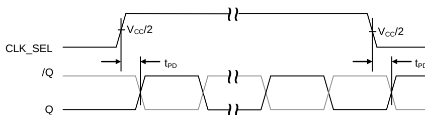
CLK_SEL-to-Differential Out
