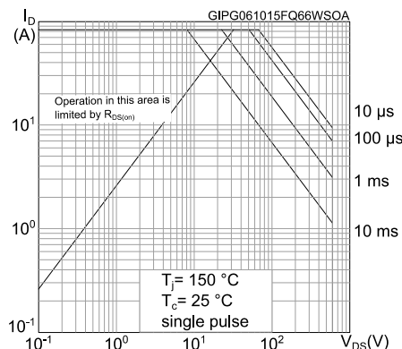
Figure 6: Safe operating area for TO-247
