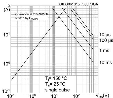
Figure 4: Safe operating area for TO-220
