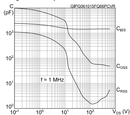
Figure 12: Capacitance variations
