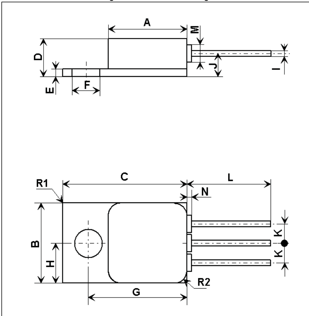
Figure 18. TO-254AA drawing
