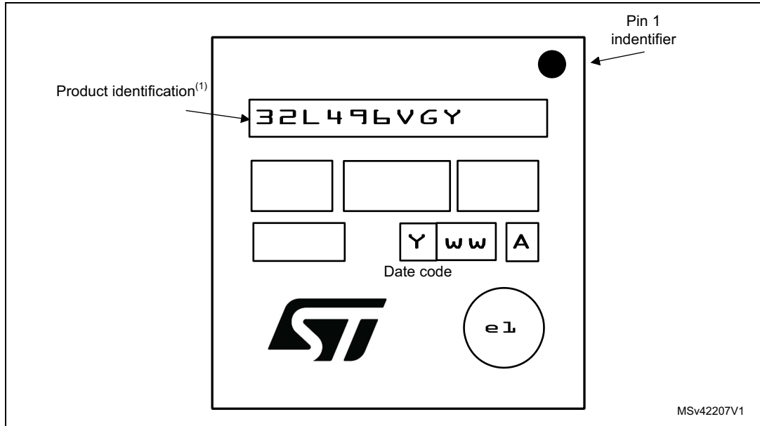
Figure 78. WLCSP100L marking (package top view)
