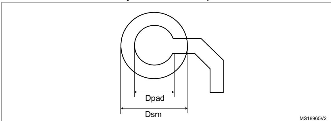
Figure 62. UFBGA169 - 169-ball, 7 x 7 mm, 0.50 mm pitch, ultra fine pitch ball grid array recommended footprint
