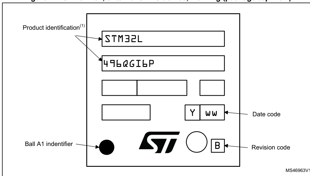
Figure 72. UFBGA132, external SMPS device, marking (package top view)
