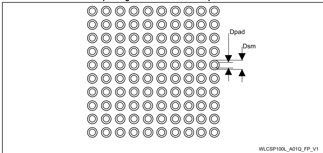
Figure 77. WLCSP100L – 100L, 4.166 x 4.628 mm 0.4 mm pitch wafer level chip scale package recommended footprint
