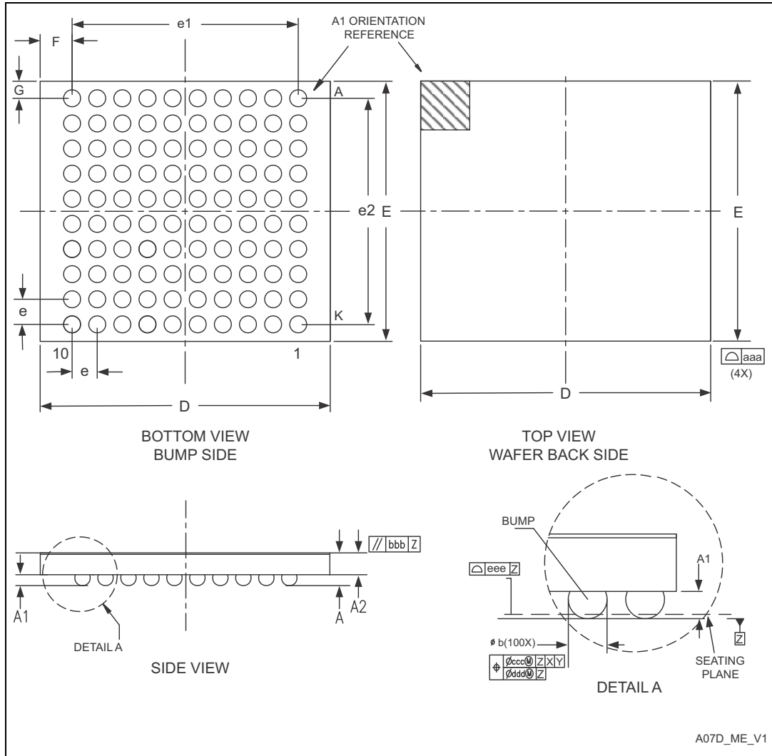
Figure 76.WLCSP100L – 4.618 x 4.142 mm, 0.4 mm pitch wafer level chip scale package outline
