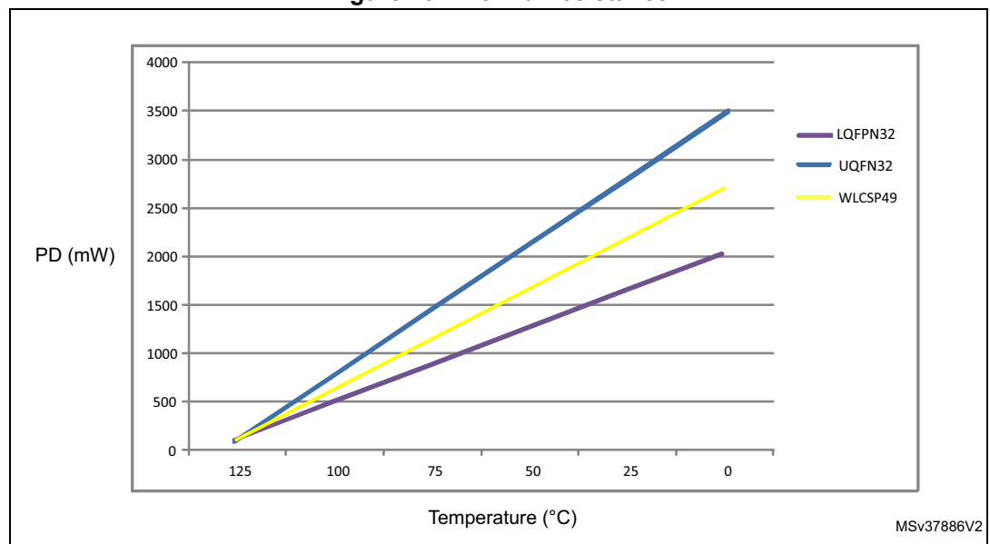
Figure 40. Thermal resistance
