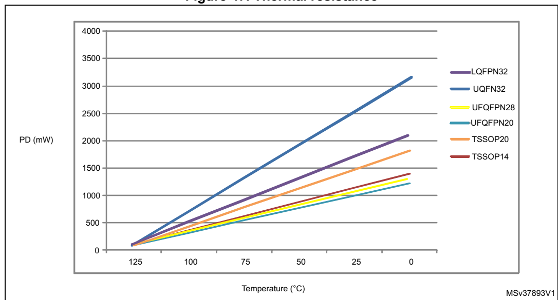
Figure 47. Thermal resistance
