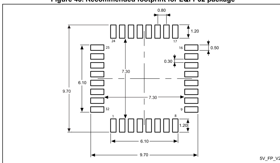
Figure 45. Recommended footprint for LQFP32 package
