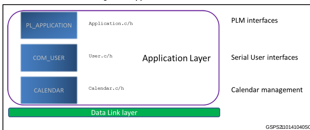
Figure 8: Application architectures
