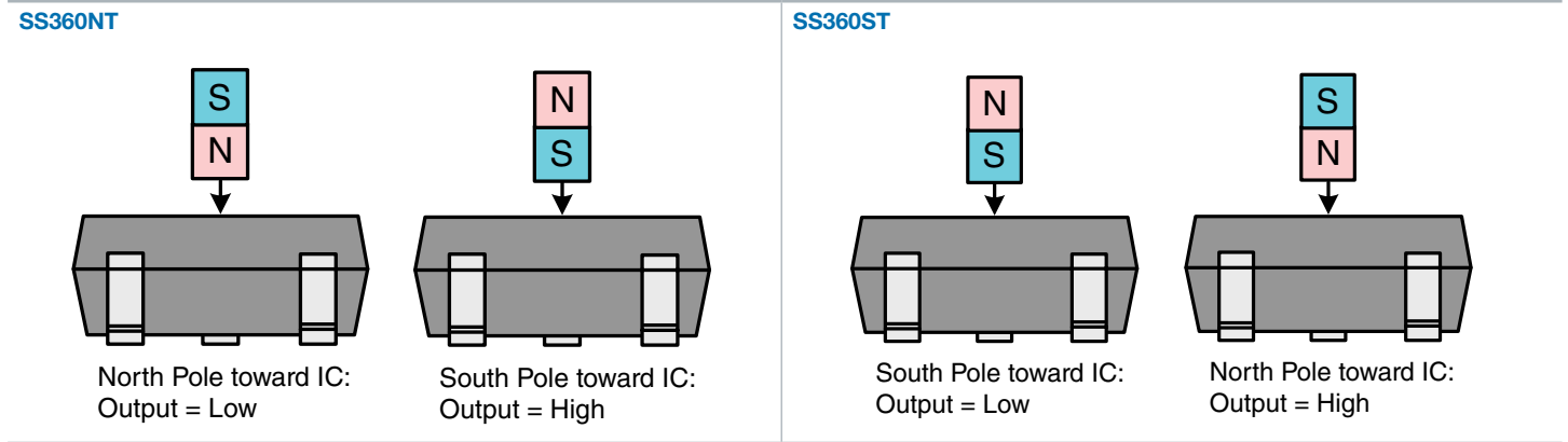
Figure 4. Magnetic Activation
