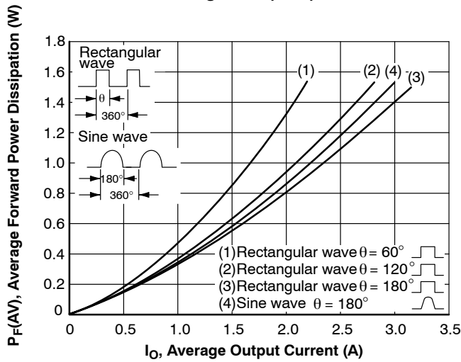
Figure 4. P_F(AV) - I_O
