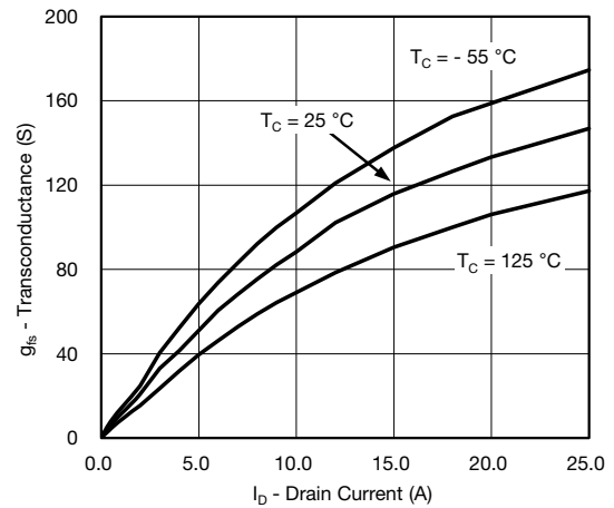
Transconductance
