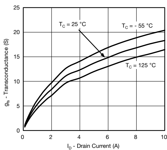
Transconductance
