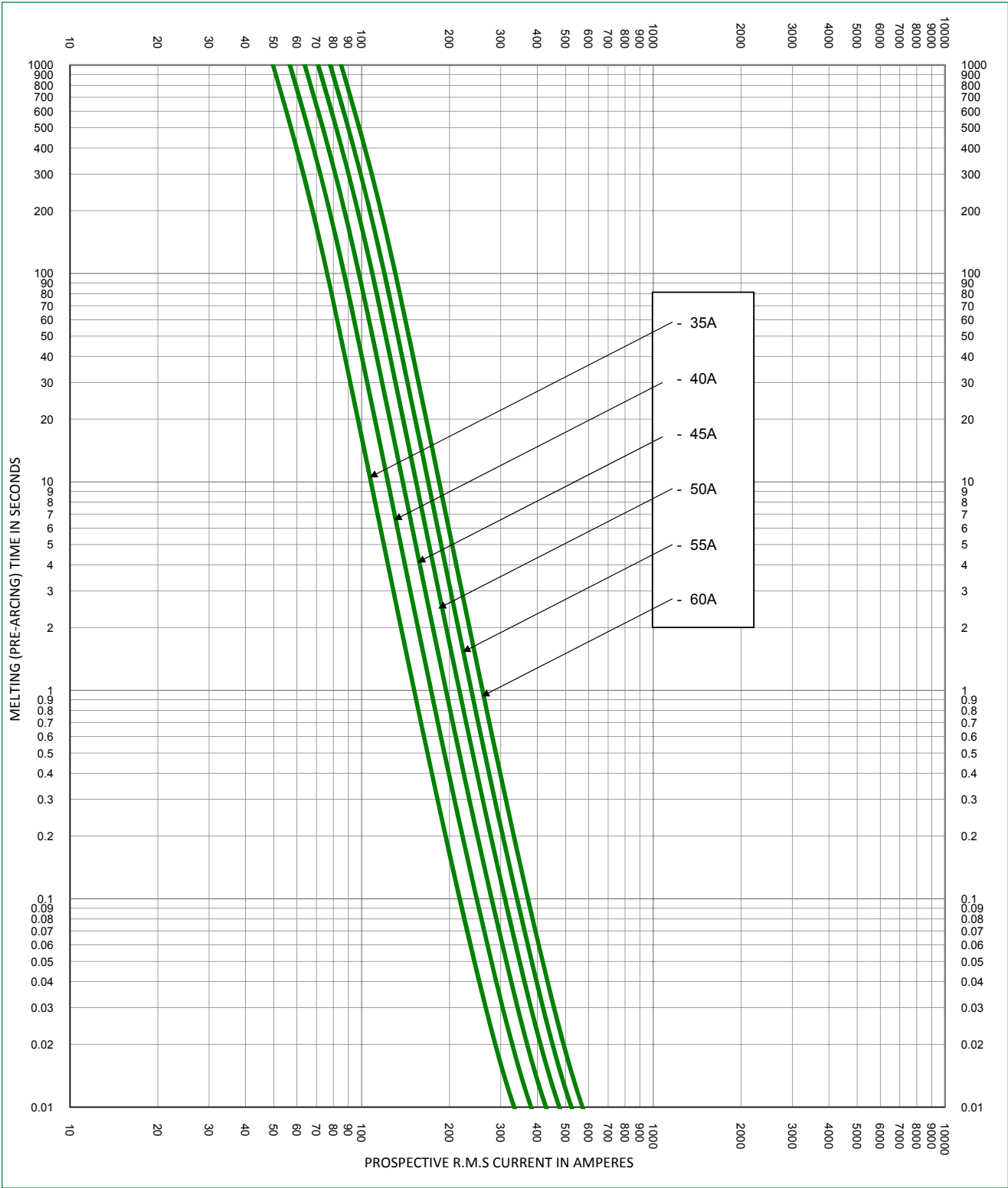
SPXV Time Current Curve (35–60 A)
