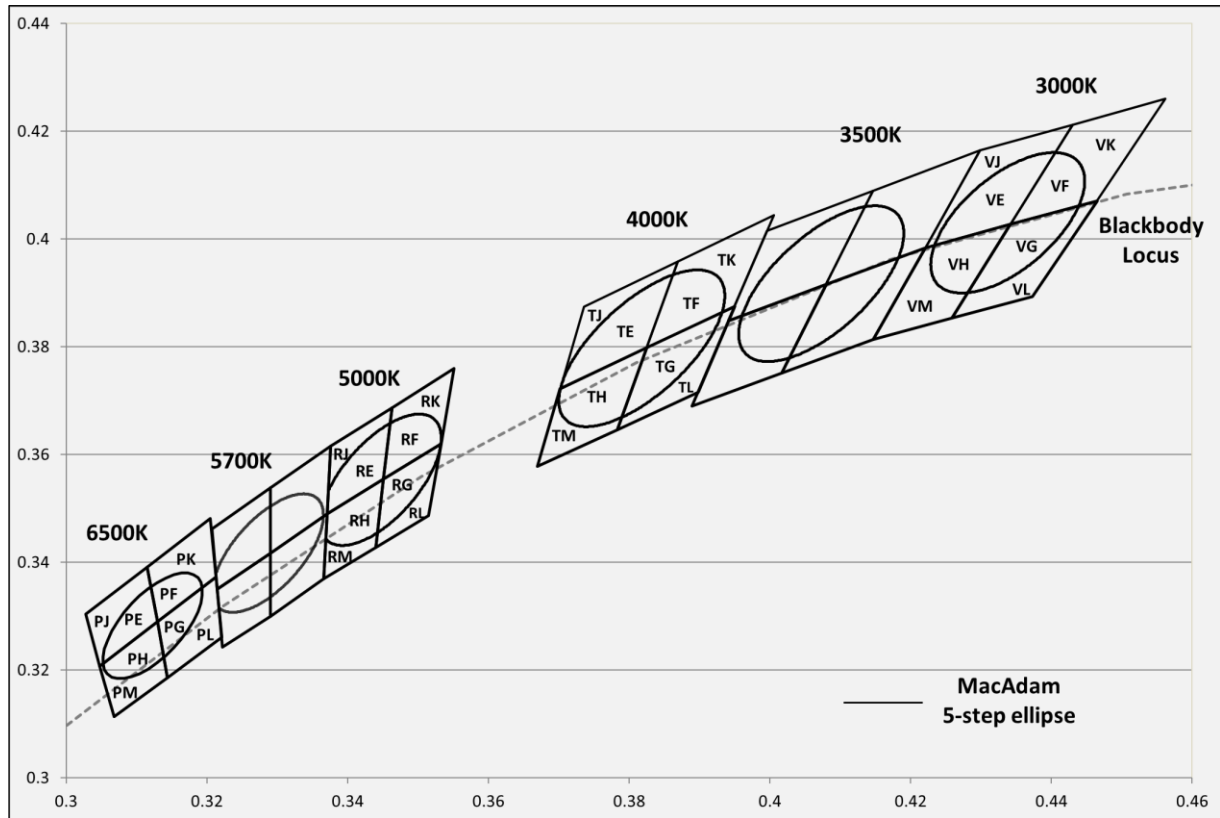
d) Chromaticity Region & Coordinates ( I_F = 65 \text{ mA} , T_s = 25^\circ\text{C} )
