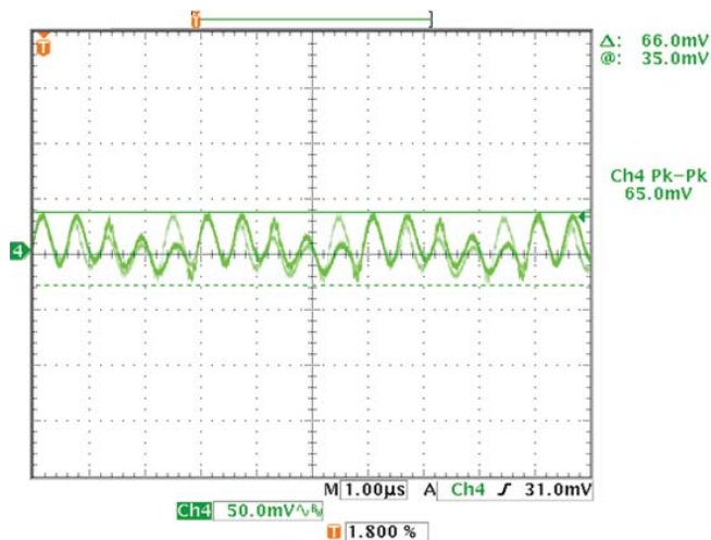
Output Ripple and Noise (Vin = 48V, Io = 2.1A, Cload = 1 \mu F || 10 \mu F, Ta = +25°C)
