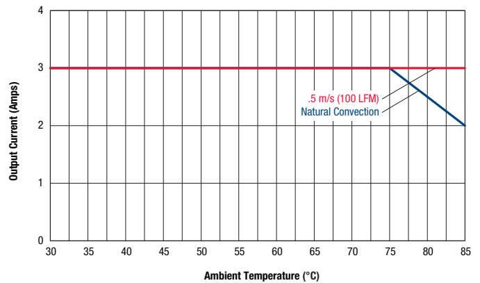
Maximum Current Temperature Derating at sea level V_{in} 36V (air flow from Pin J1 to Pin J3 on PCB)
