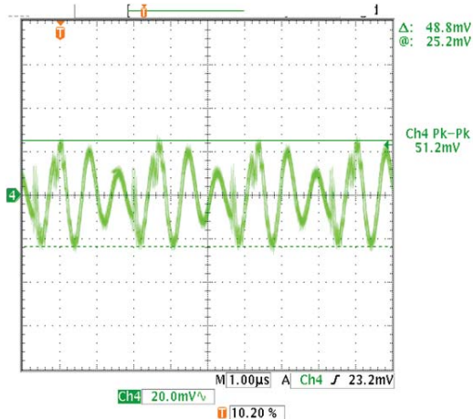
Output Ripple and Noise ( V_{in} = 24V , I_{out} = 0.30A , C_{load} = 1\mu F \parallel 10\mu F , T_a = +25^\circ C , BW = 20Mhz )
