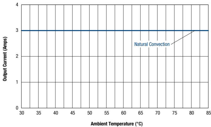
Maximum Current Temperature Derating at sea level V_{in} = 9V, 12V, \text{ or } 24V (air flow from Pin J1 to Pin J3 on PCB)
