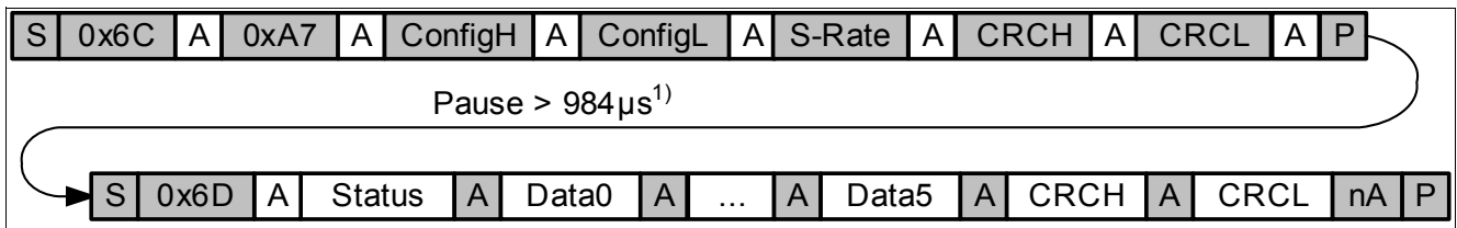
Figure 51 Measure Pressure
