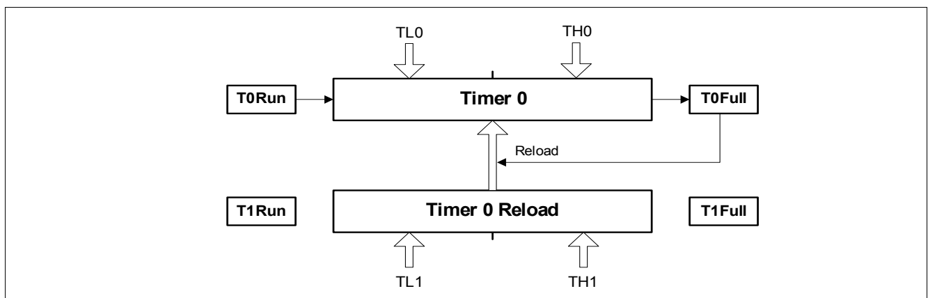
Figure 34 Timer Mode 0
