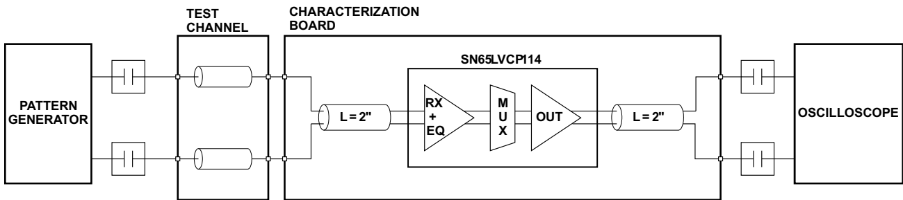
Figure 9. Receive-Side Performance Test Circuit
