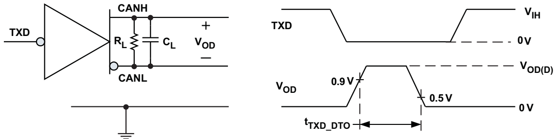
Figure 14. TXD Dominant Timeout Test Circuit and Measurement
