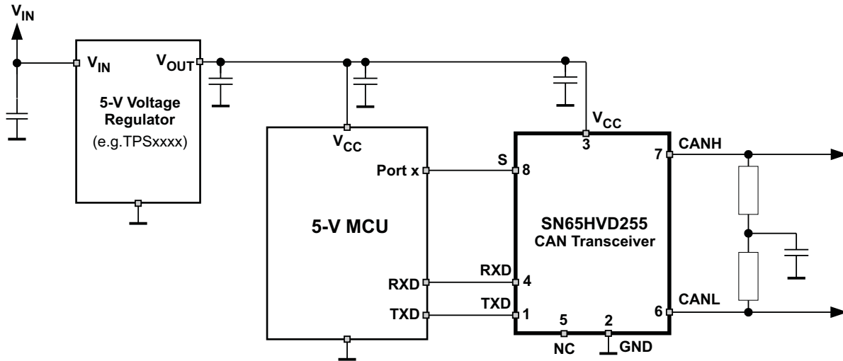
Figure 16. Typical 5V Application
