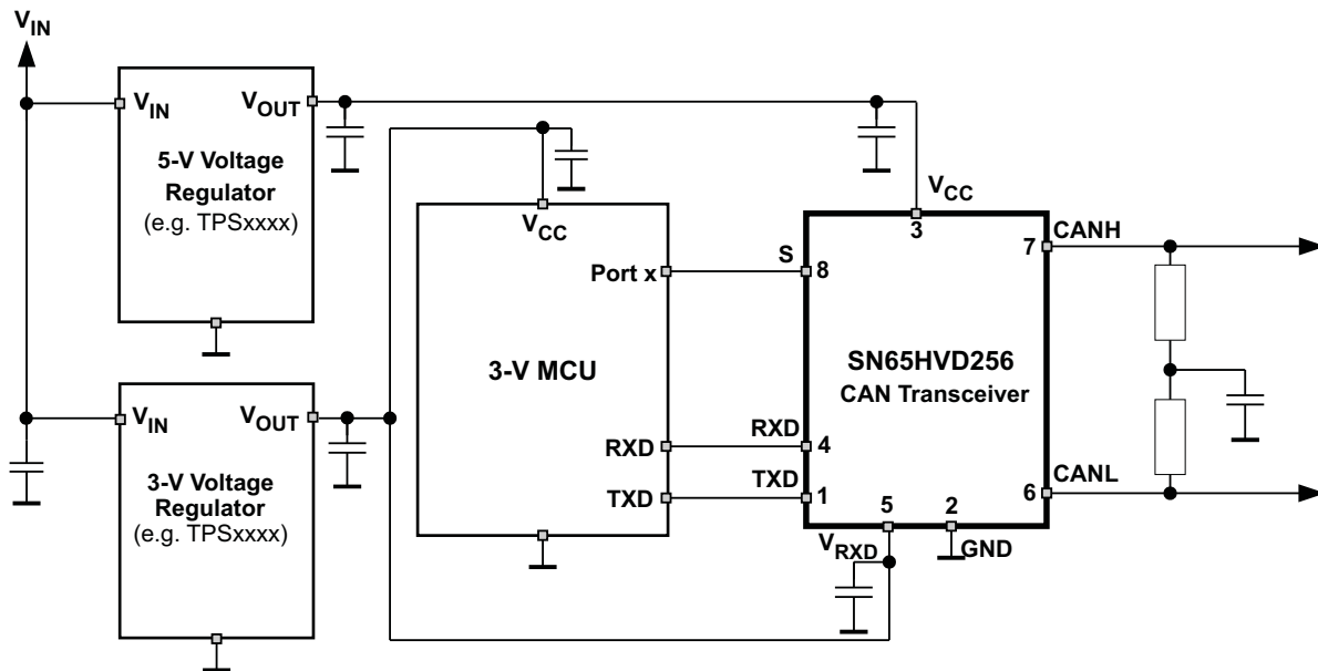
Figure 17. Typical 3.3V Application
