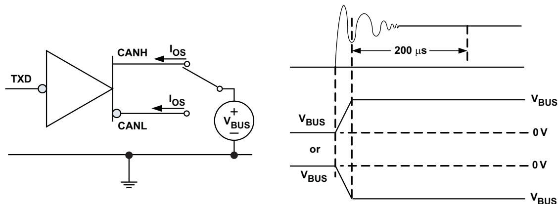
Figure 15. Driver Short Circuit Current Test and Measurement
