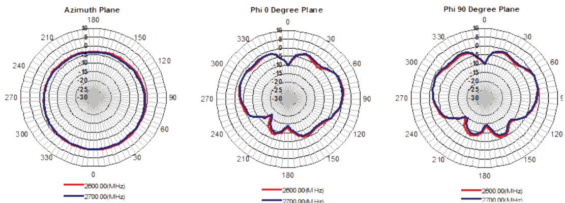
2400-2700 MHz Band
