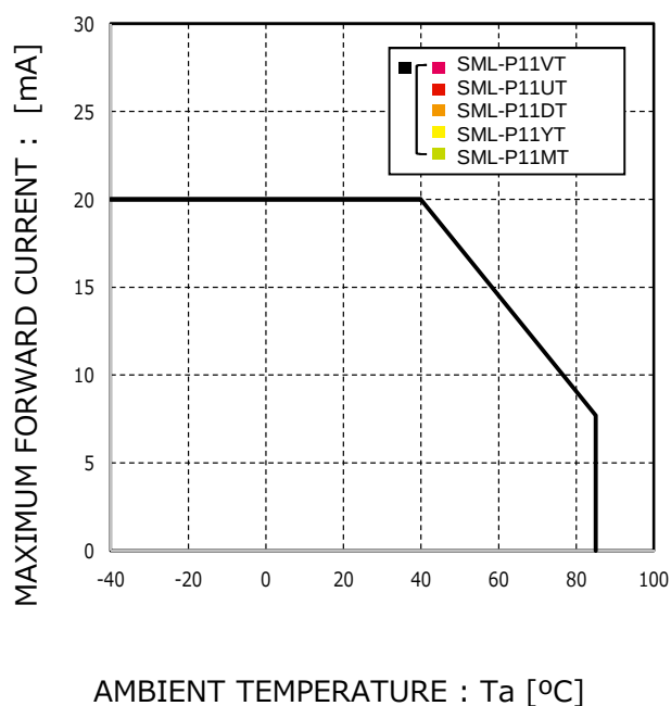
Fig.4 Derating
