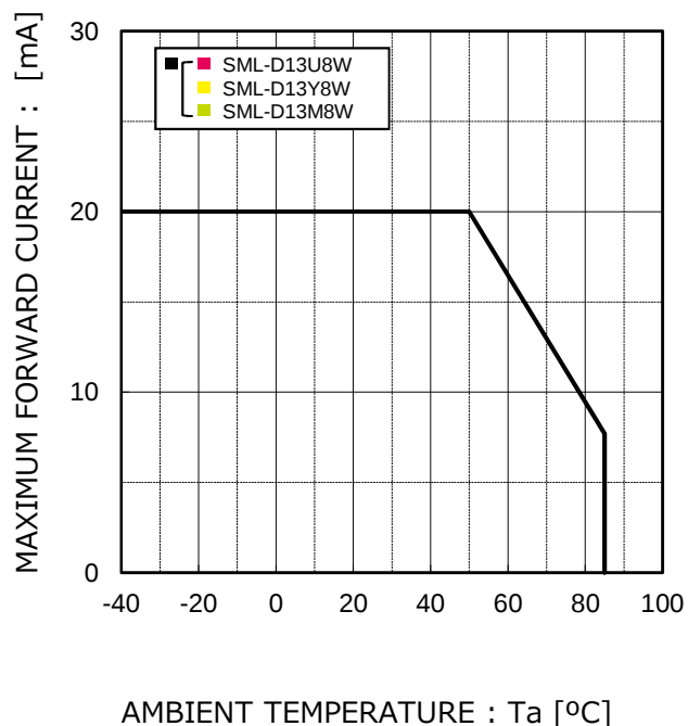
Fig.4 Derating
