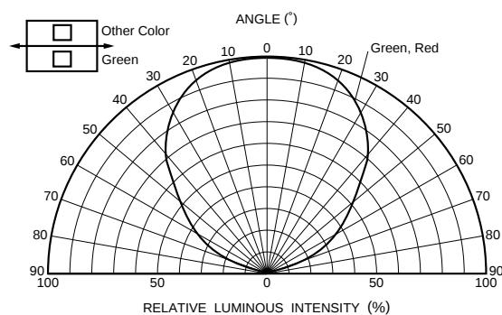
Fig. 2 Directional pattern (2)
