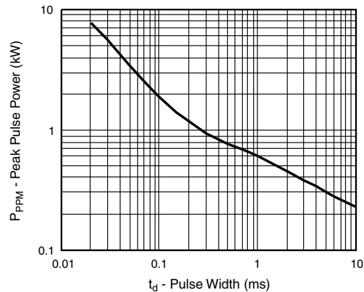
Fig. 2 - Peak Pulse Power Rating Curve
