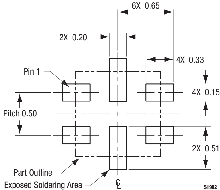
Figure 10. SKY13453-385LF PCB Layout Footprint (Top View)
