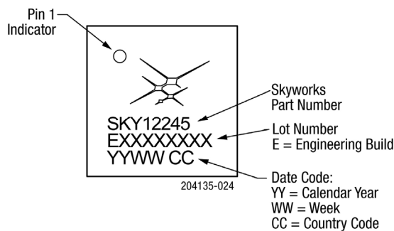
Figure 24. Typical Part Markings (Top View)
