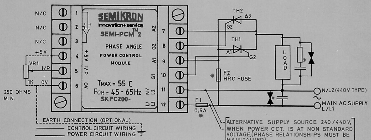
BASIC A.C. REGULATOR (W1C) WIRING
