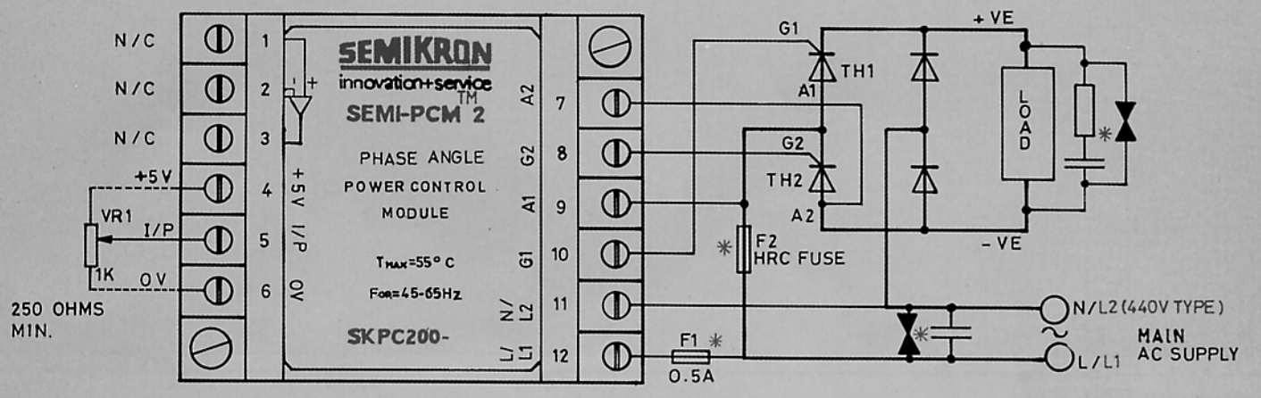
HALF CONTROLLED D.C. BRIDGE (B2HZ) WIRING
