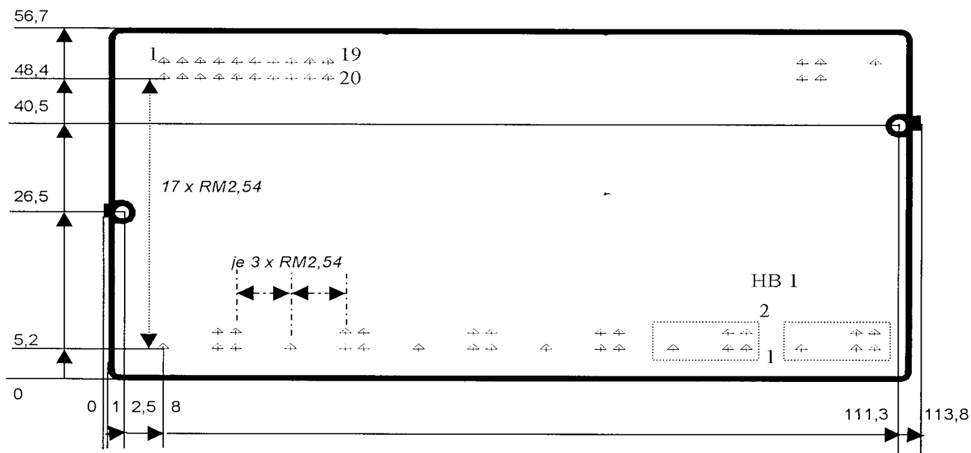
Fig. 9 Dimensional drawing, layout
