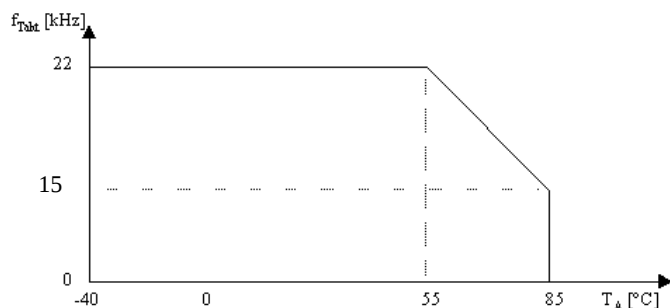
Fig. 6 Maximum cycling frequency at Q_{GE} = 1000 \text{ nC} vs temperature
