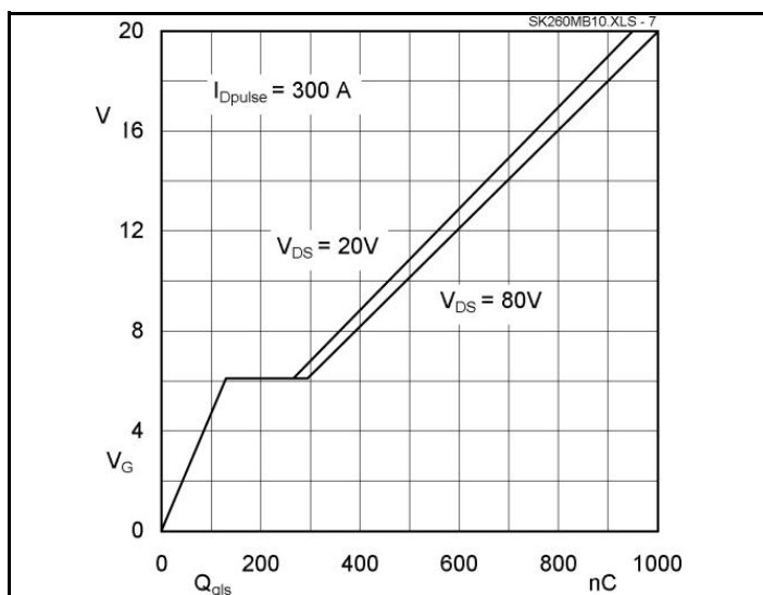
Fig. 7 Gate charge characteristic, I_{Dp} = 300 A
