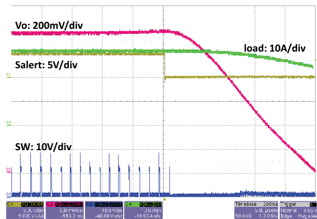
Fig. 32 - SiC451 OCP
