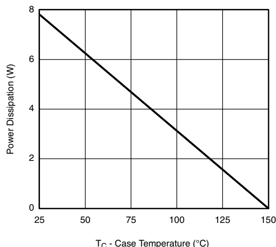
Power Derating
