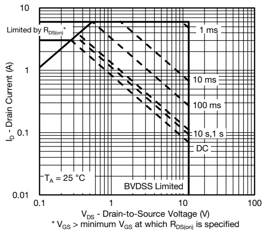
Safe Operating Area, Junction-to-Foot
