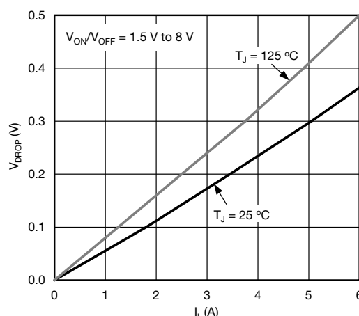
V_{DROP} vs. I_L at V_{IN} = 1.8\text{ V}
