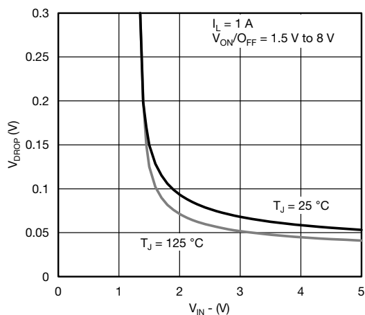
V_{DROP} vs. V_{IN} at I_L = 1\text{ A}
