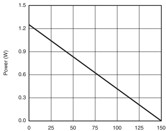
Power Derating ( T_A )
