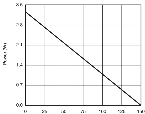
Power Derating ( T_C )
