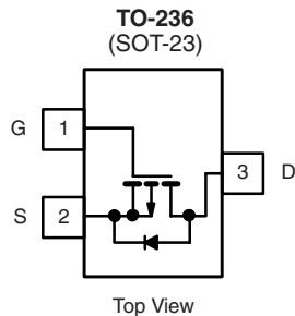
Top View Si2301 BDS (L1)* * Marking Code
