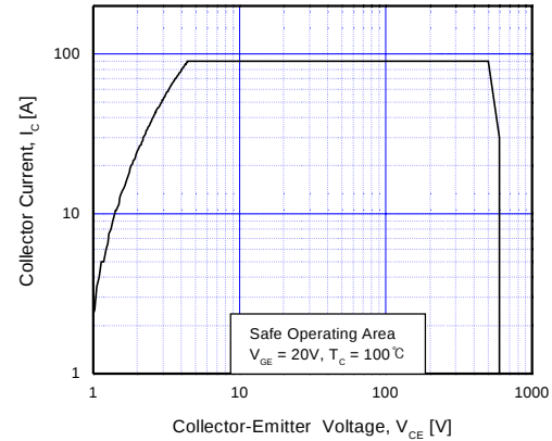
Fig 16. Turn-Off SOA Characteristics
