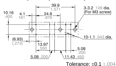
PC board pattern (Bottom view)
