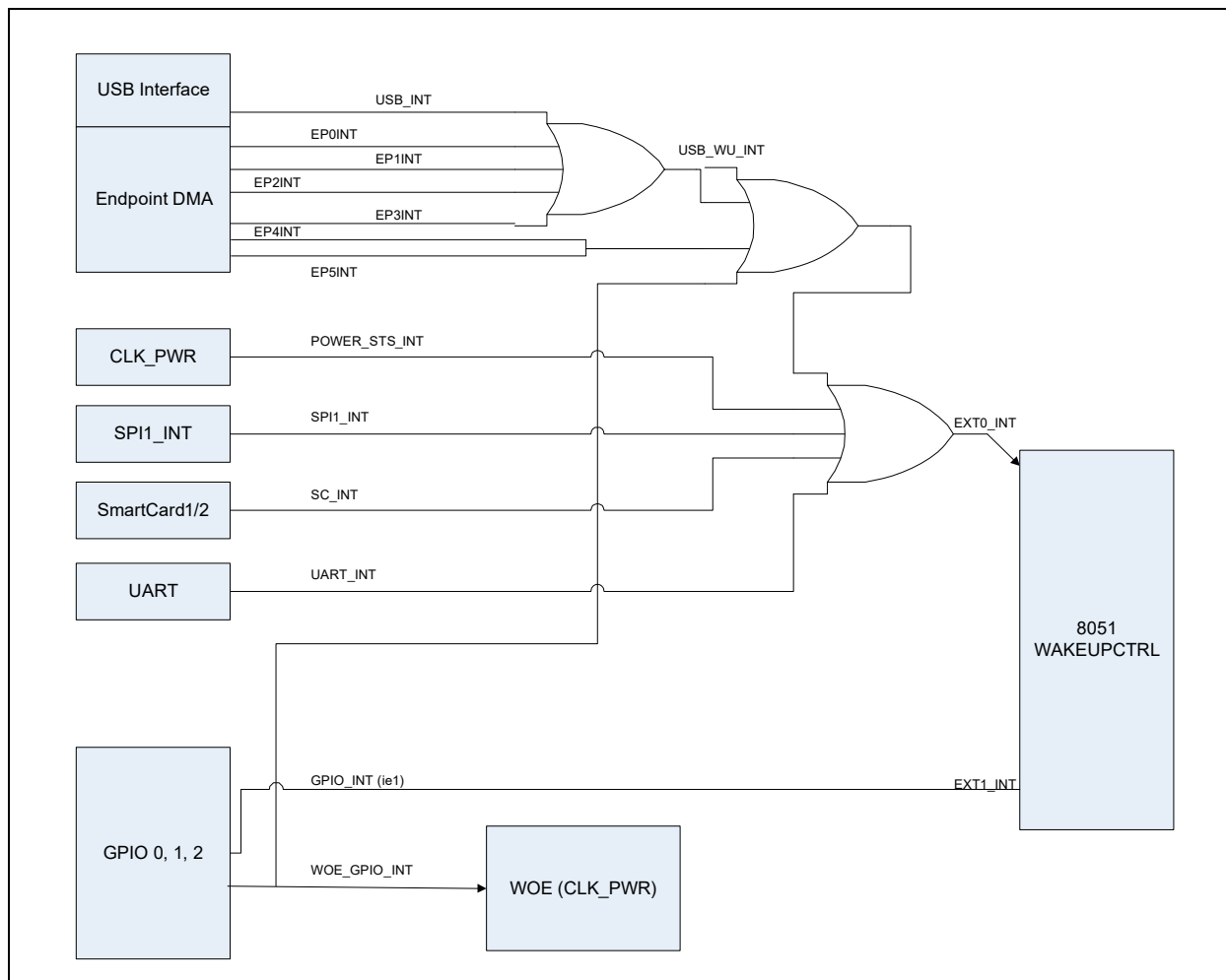
FIGURE 8-1: WAKE-UP INTERRUPT
