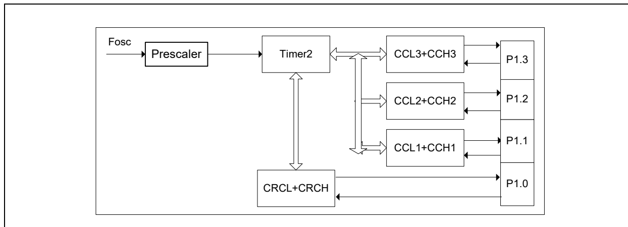
FIGURE 19-6: TIMER 2 BLOCK DIAGRAM
