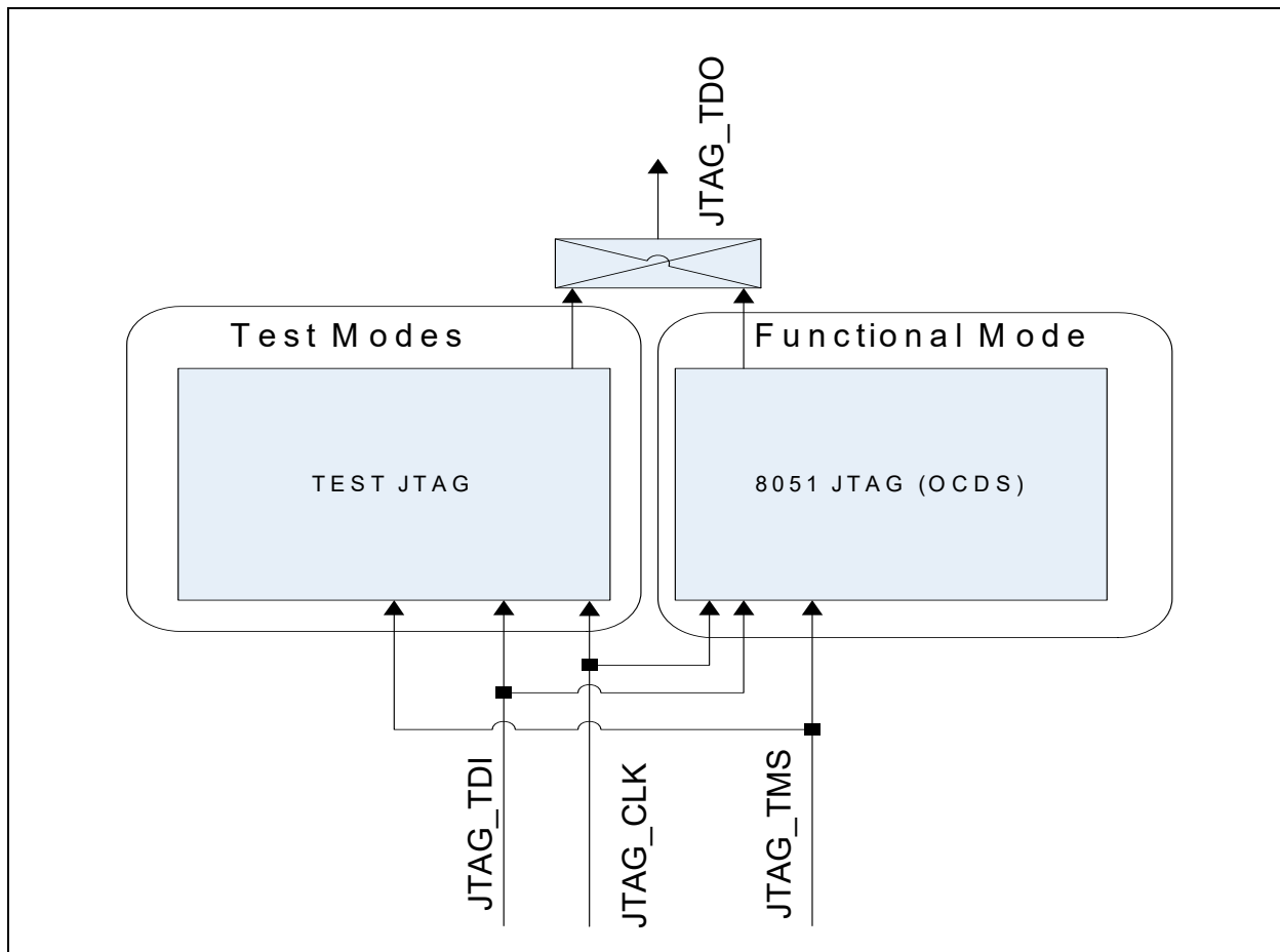
FIGURE 17-1: JTAG TEST BLOCK DIAGRAM
