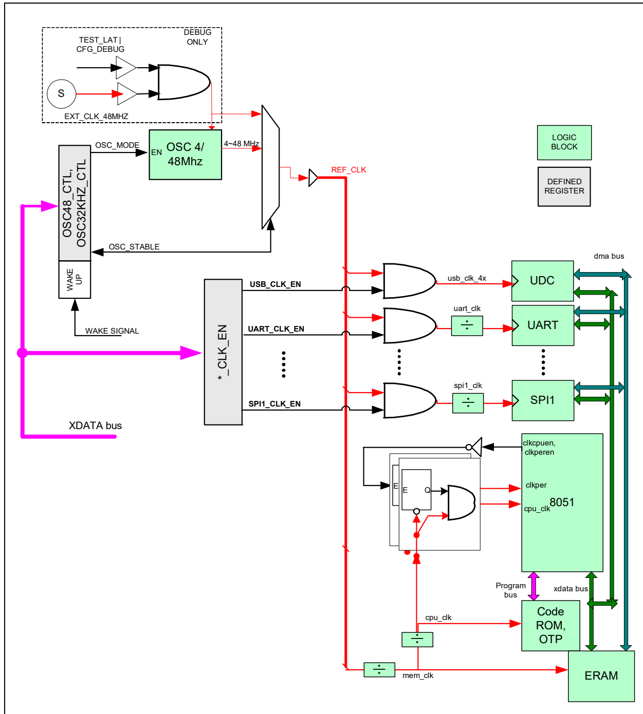
FIGURE 15-1: CLOCK GENERATION
