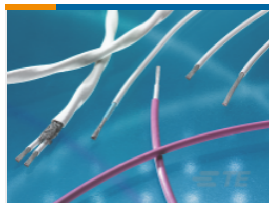
TE Part #955741-000 2 Core Twisted Pair Cable: Tin Coated Copper Cable, 22 AWG
