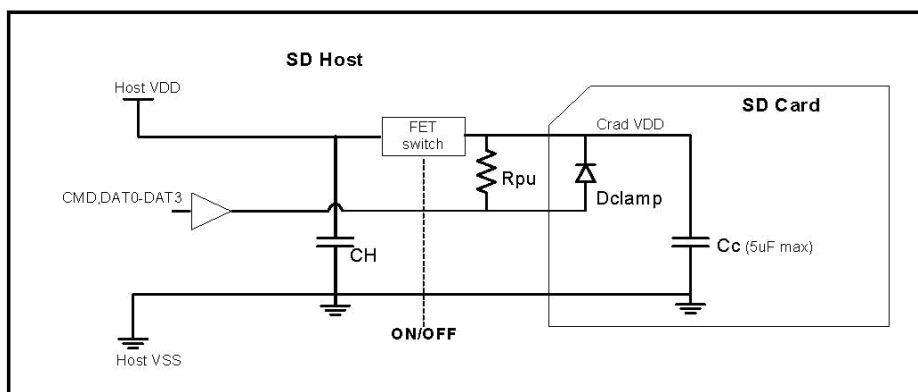
Figure 4: Recommended Power Control Scheme
