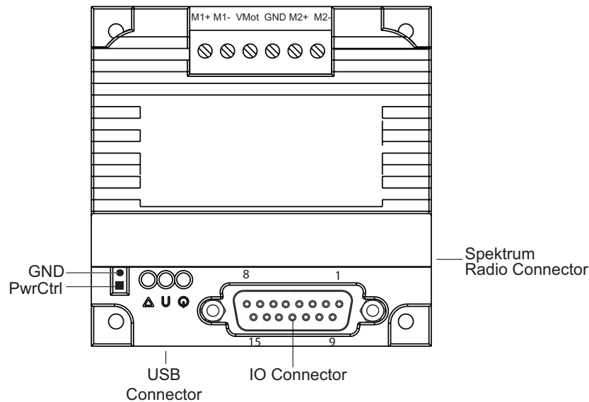
FIGURE 1. Controller top view layout
