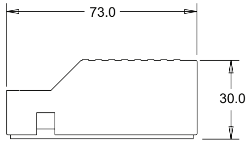
FIGURE 11. SDC21xx Front view and dimensions
