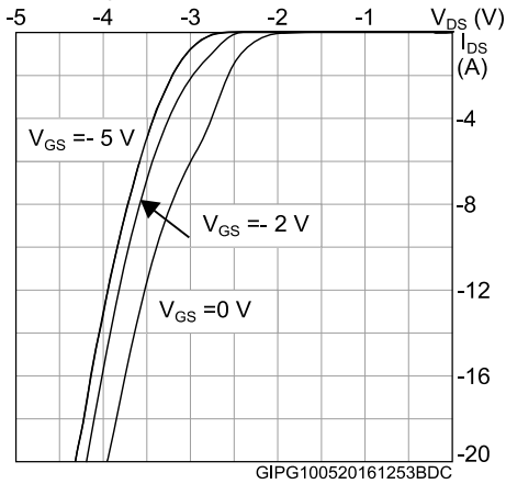
Figure 16: Body diode characteristics (Tj= -50 °C)
