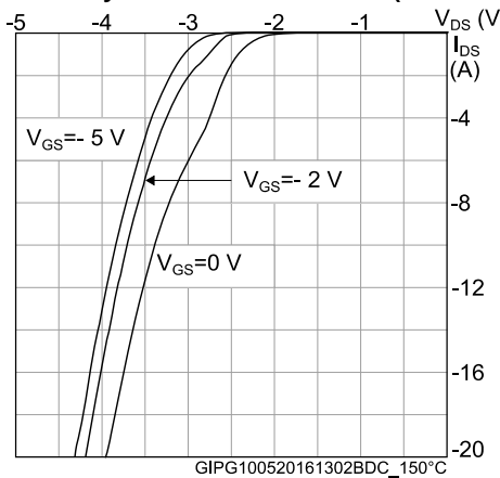
Figure 18: Body diode characteristics (Tj= 150 °C)
