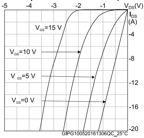
Figure 20: 3rd quadrant characteristics (T J = 25 °C)
