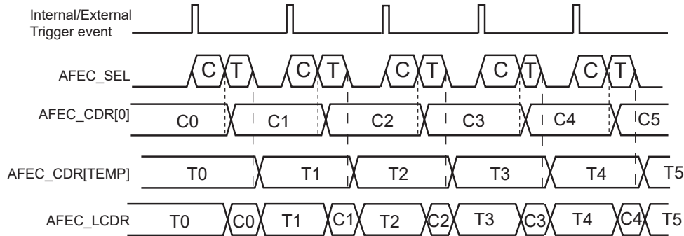
Figure 52-8. Non-Optimized Temperature Conversion
