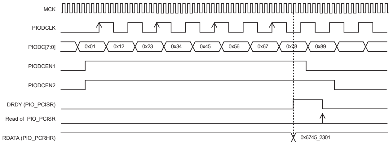
Figure 32-13. Parallel Capture Mode Waveforms (DSIZE = 2, ALWYS = 0, HALFS = 1, FRSTS = 1)
