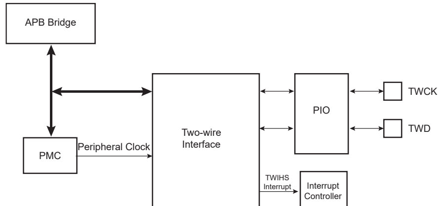
Figure 43-1. Block Diagram
