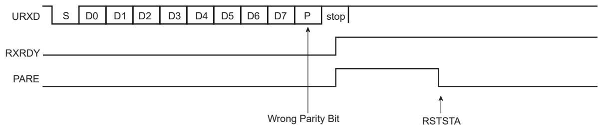
Figure 47-7. Parity Error
