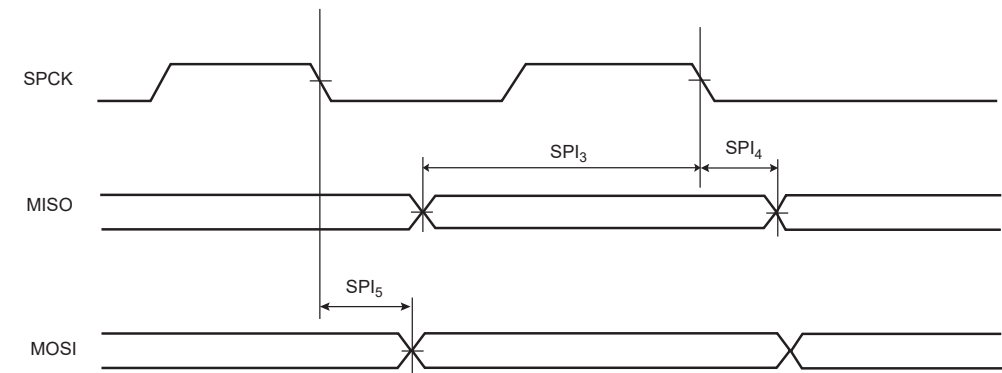
Figure 58-21. SPI Master Mode with (CPOL = 0 and NCPHA=1) or (CPOL=1 and NCPHA= 0)
