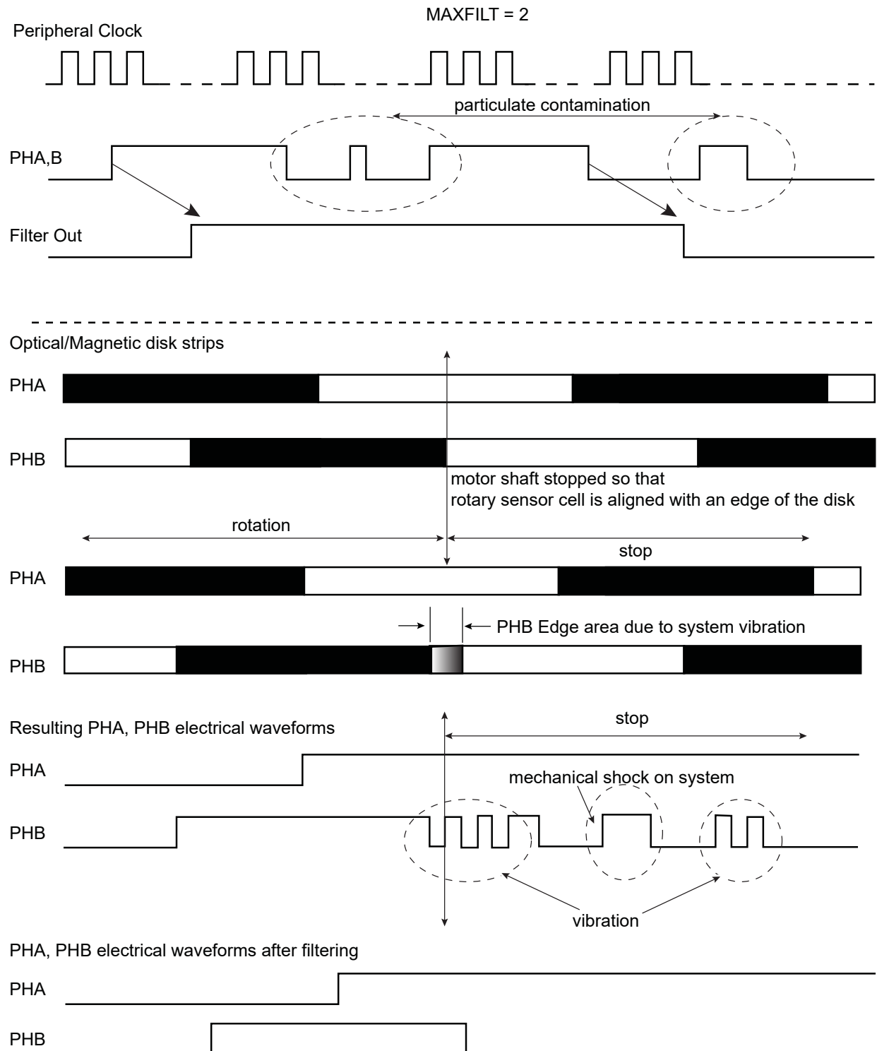
Figure 50-19. Filtering Examples
