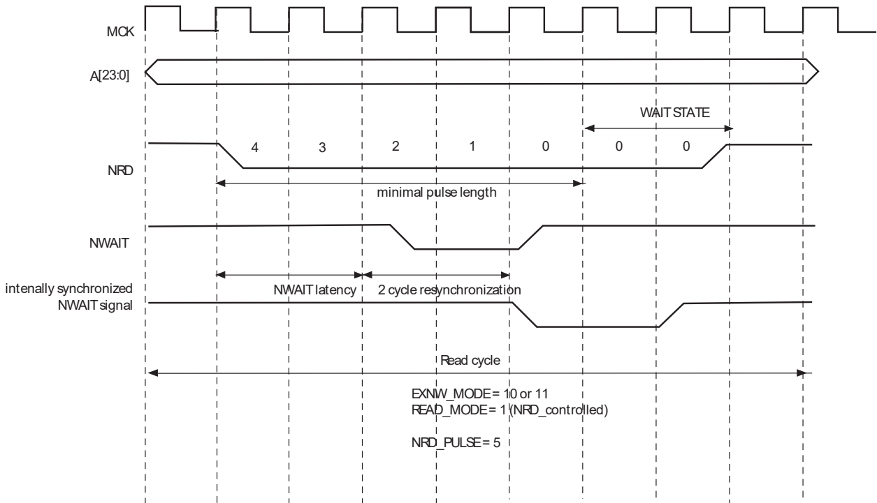
Figure 35-31. NWAIT Latency
