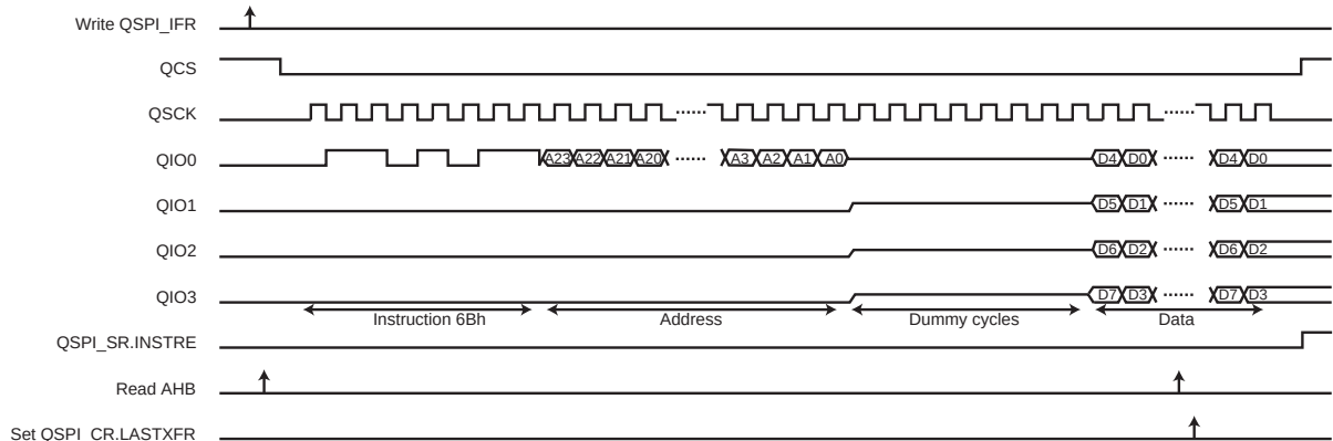
Figure 42-16. Instruction Transmission Waveform 6
