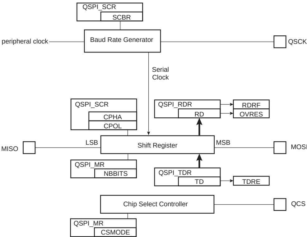
Figure 42-5. SPI Mode Block Diagram
