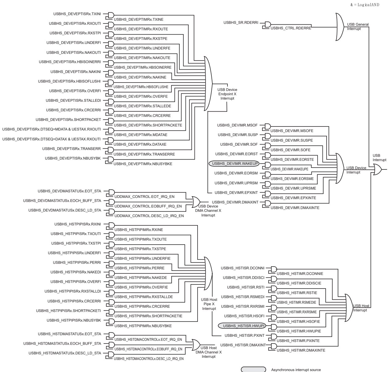
Figure 39-3. Interrupt System
