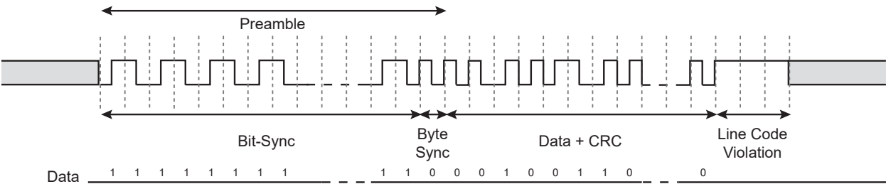
Figure 46-55. LON Framing
