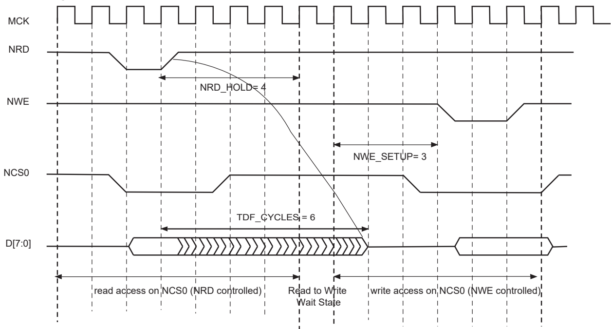
Figure 35-23. TDF Optimization: No TDF wait states are inserted if the TDF period is over when the next access begins
