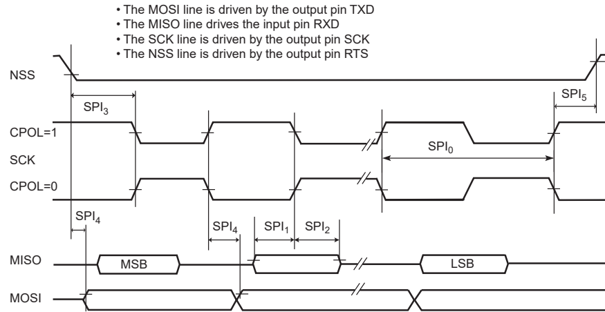
Figure 58-27. USART SPI Slave Mode (Mode 1 or 2)
