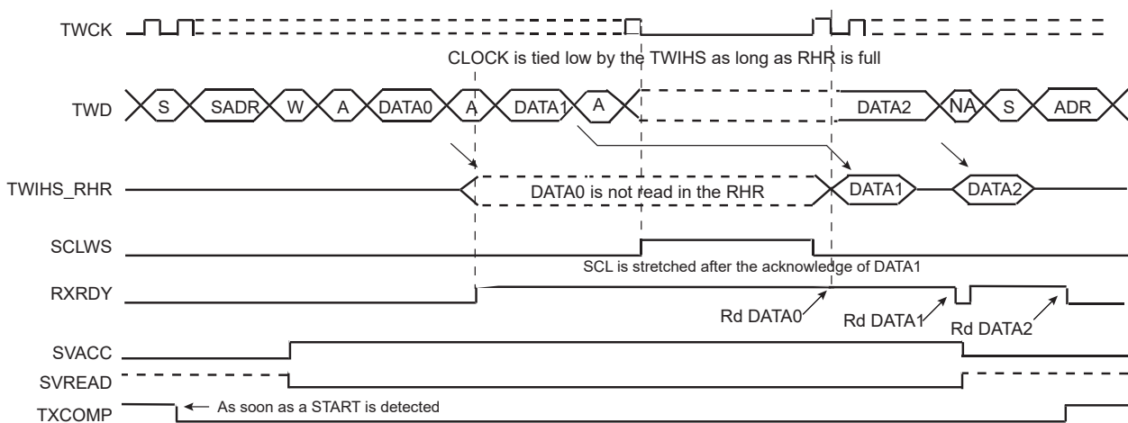
Figure 43-35. Clock Stretching in Write Mode
