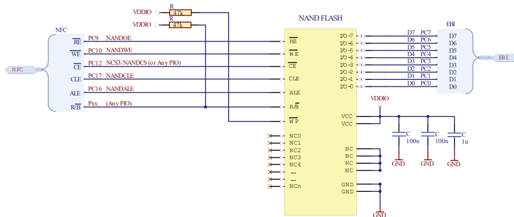
Figure 59-4. Schematic Example with a 2 Gb/8-bit NAND Flash
