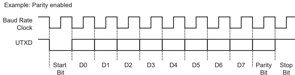
Figure 47-9. Character Transmission
