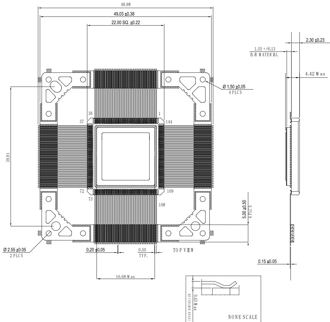
Figure 61-2. 144-pin CQFP Package Mechanical Drawing
