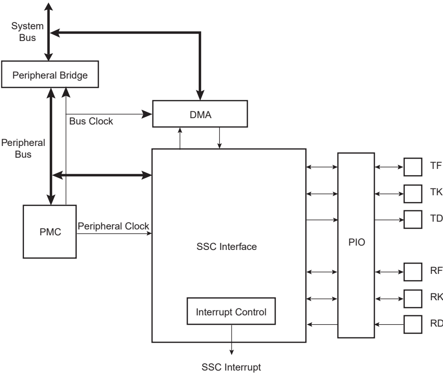
Figure 44-1. Block Diagram
