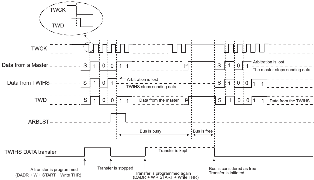
Figure 42-29. Arbitration Cases
