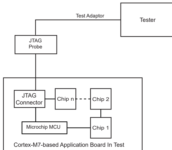
Figure 15-3. Application Test Environment Example
