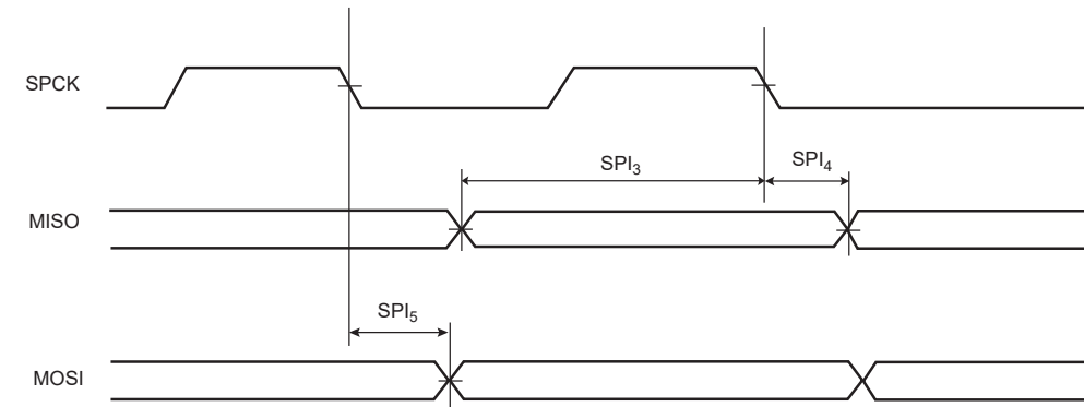
Figure 57-21. SPI Master Mode with (CPOL = 0 and NCPHA=1) or (CPOL=1 and NCPHA= 0)
