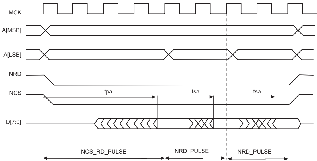
Figure 34-35. Page Mode Read Protocol (Address MSB and LSB are defined in Table 34-7)
