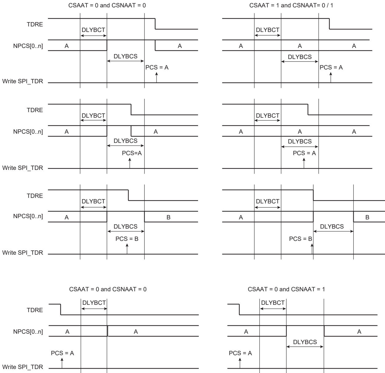
Figure 40-11. Peripheral Deselection
