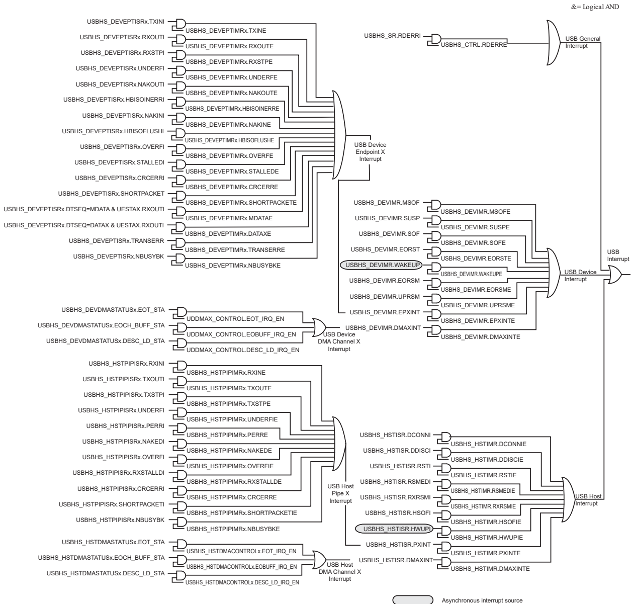
Figure 38-3. Interrupt System
