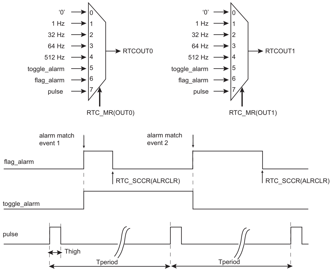
Figure 26-6. Waveform Generation
