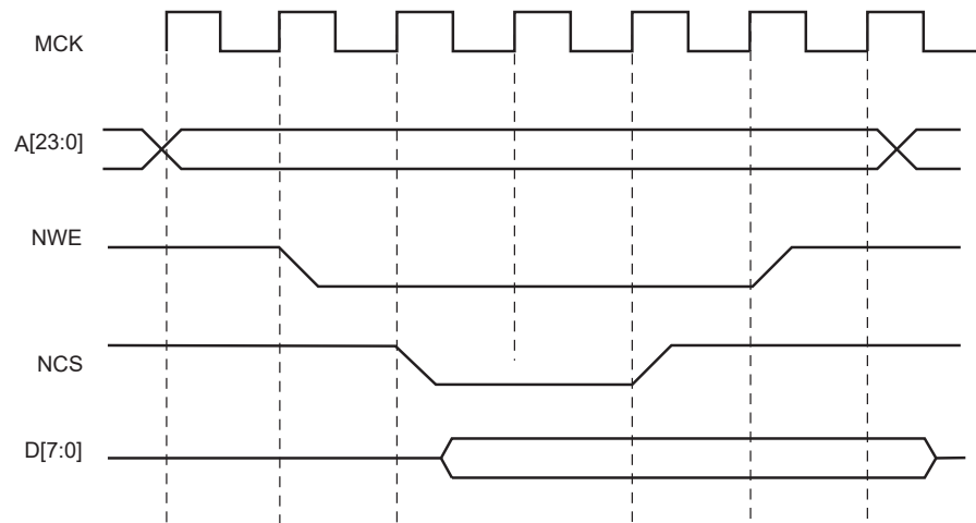
Figure 34-22. TDF Period in NCS Controlled Read Operation (TDF = 3)
