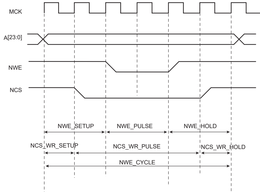
Figure 34-13. Write Cycle
