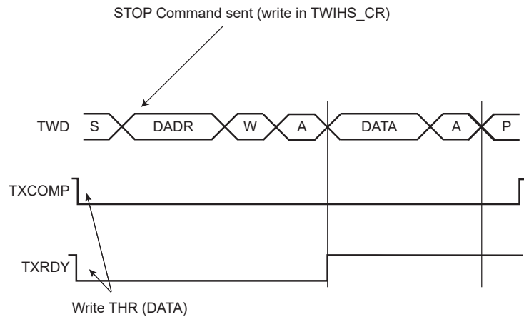
Figure 42-5. Master Write with Multiple Data Bytes
