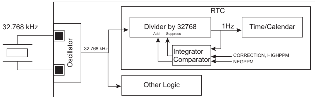
Figure 26-4. Calibration Circuitry
