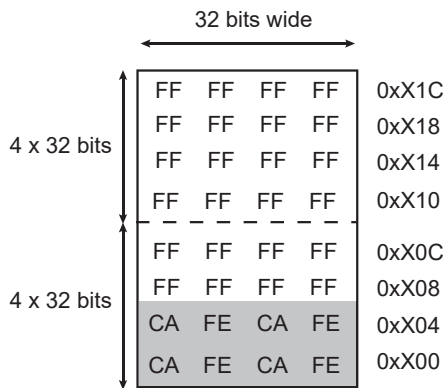
Figure 21-10. Optimized Partial Page Programming
