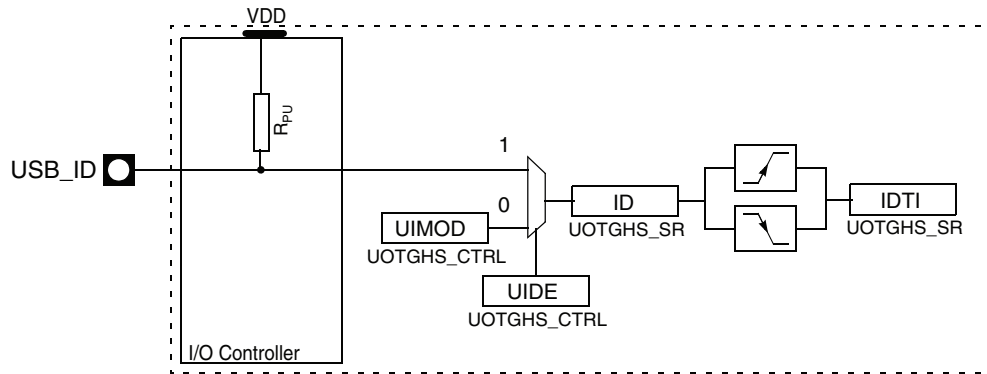
FIGURE 39-17: ID DETECTION INPUT BLOCK DIAGRAM
