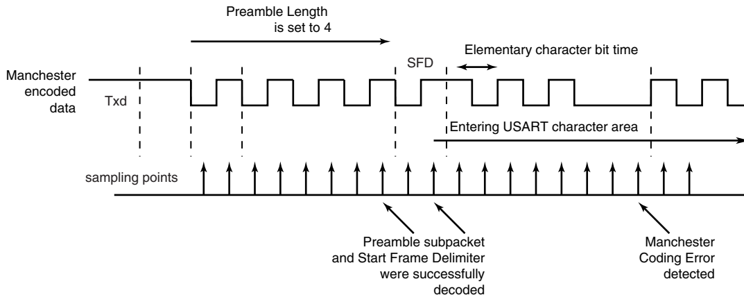
FIGURE 35-24: MANCHESTER ERROR FLAG
