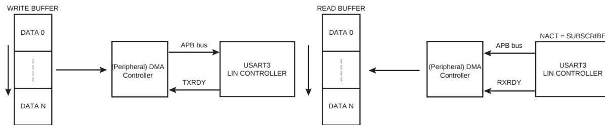
FIGURE 35-62: SLAVE NODE WITH PDC
