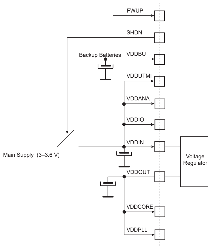
FIGURE 6-4: BACKUP BATTERIES USED
