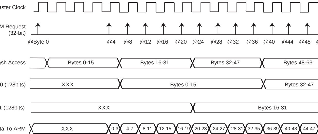
FIGURE 19-3: CODE READ OPTIMIZATION FOR FWS = 3
