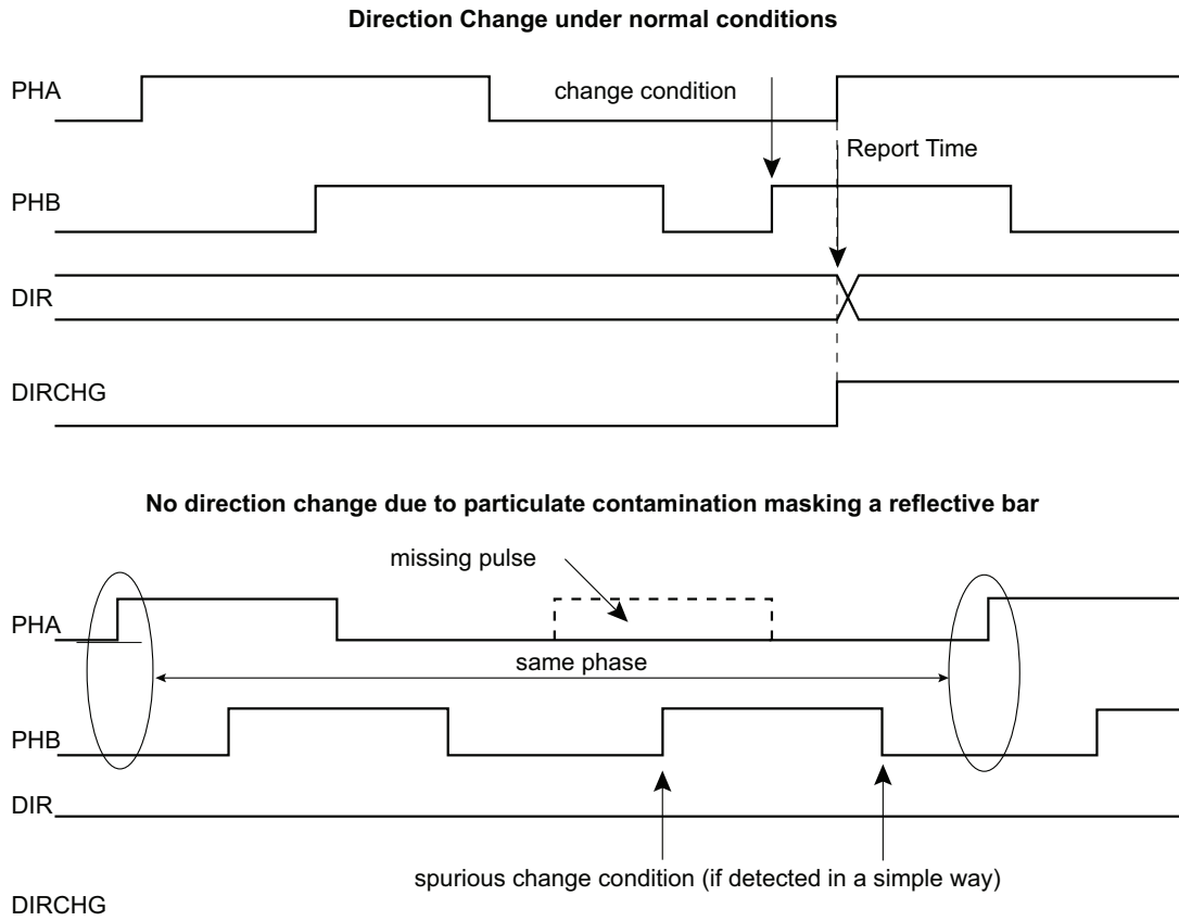
FIGURE 36-22: ROTATION CHANGE DETECTION
