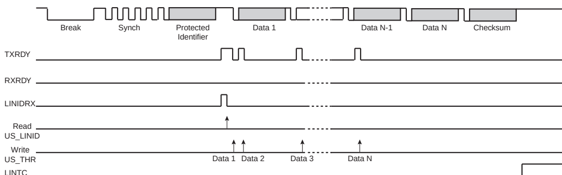
FIGURE 35-57: SLAVE NODE CONFIGURATION, NACT = PUBLISH
