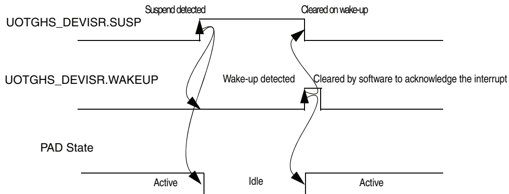
FIGURE 39-15: PAD EVENTS
