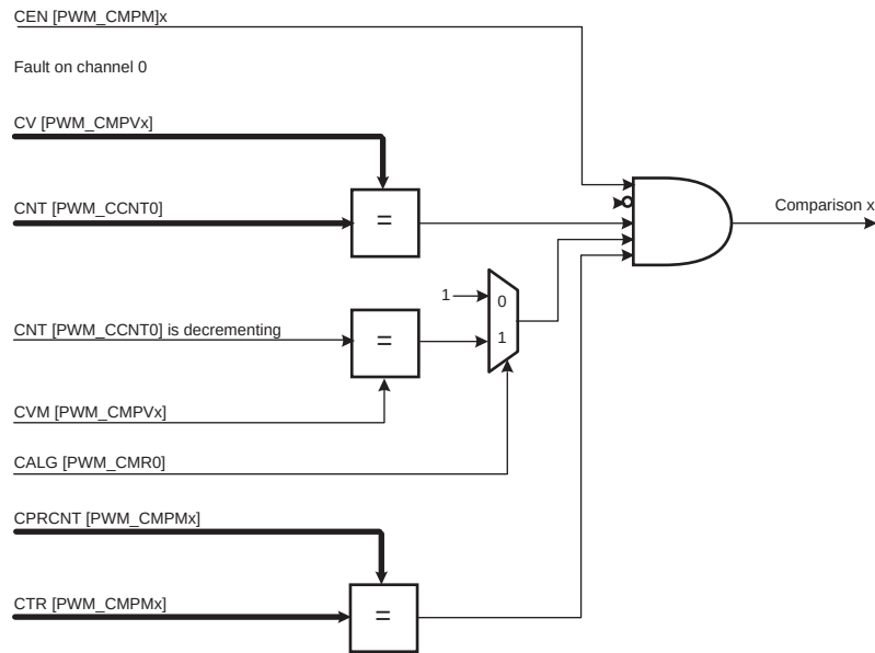
FIGURE 38-18: COMPARISON UNIT BLOCK DIAGRAM
