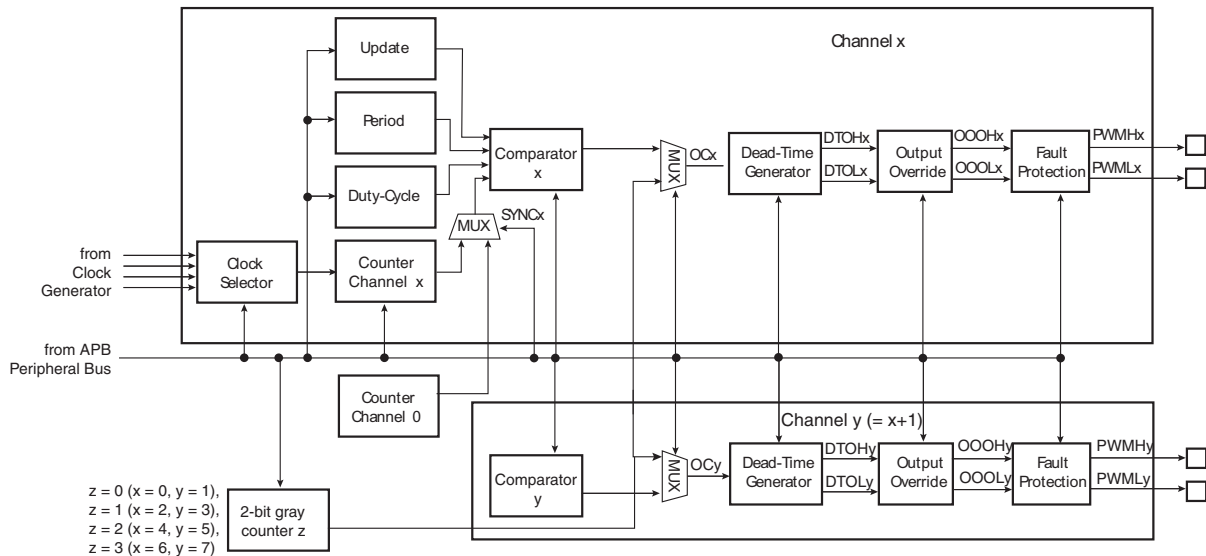
FIGURE 38-7: FUNCTIONAL VIEW OF THE CHANNEL BLOCK DIAGRAM
