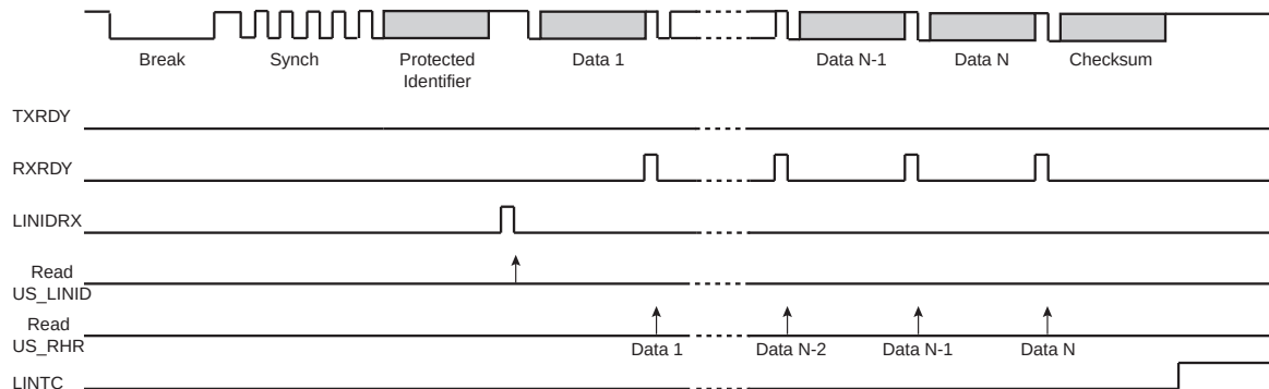
FIGURE 35-58: SLAVE NODE CONFIGURATION, NACT = SUBSCRIBE
