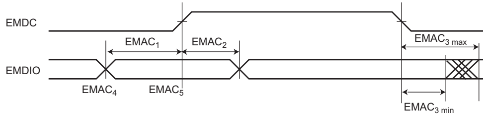
FIGURE 45-35: MIN AND MAX ACCESS TIME OF EMAC OUTPUT SIGNALS
