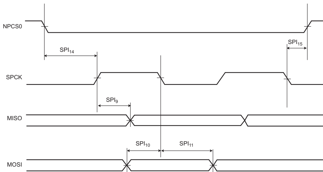
FIGURE 45-20: SPI SLAVE MODE WITH (CPOL = NCPHA = 0) OR (CPOL = NCPHA = 1)
