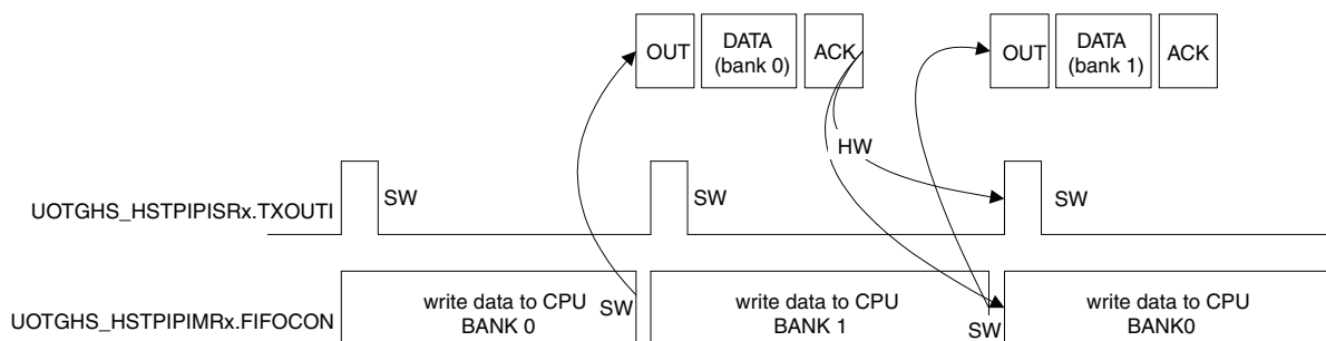
FIGURE 39-33: EXAMPLE OF AN OUT PIPE WITH TWO DATA BANKS AND NO BANK SWITCHING DELAY
