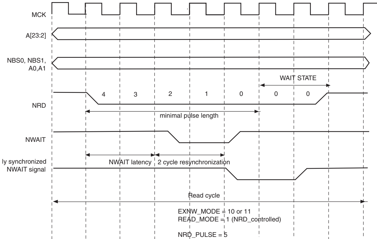
FIGURE 25-27: NWAIT LATENCY
