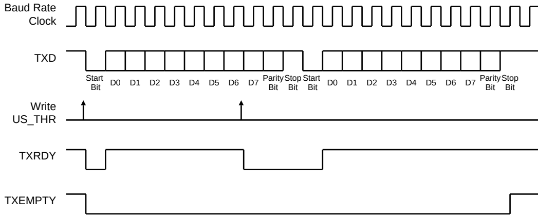
FIGURE 35-15: TRANSMITTER STATUS
