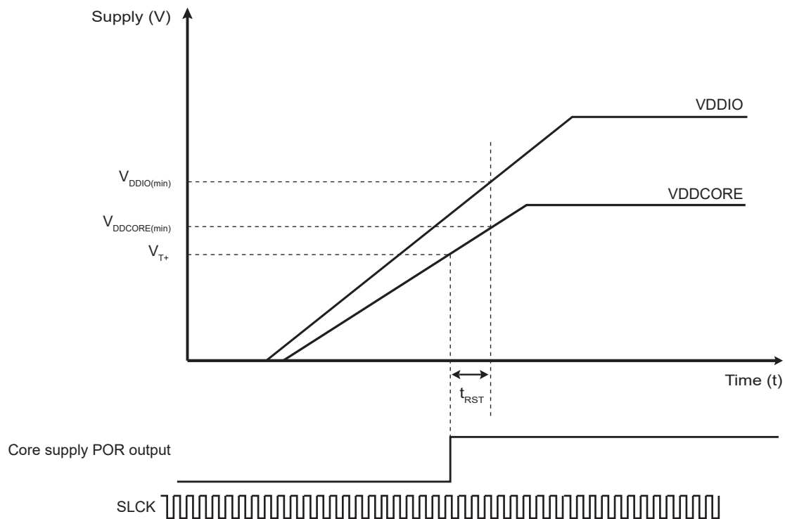
FIGURE 6-1: VDDCORE AND VDDIO CONSTRAINTS AT STARTUP
