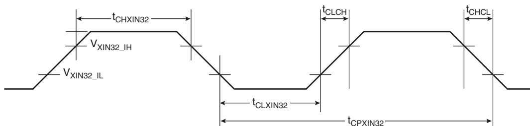
FIGURE 45-11: XIN32 CLOCK TIMING
