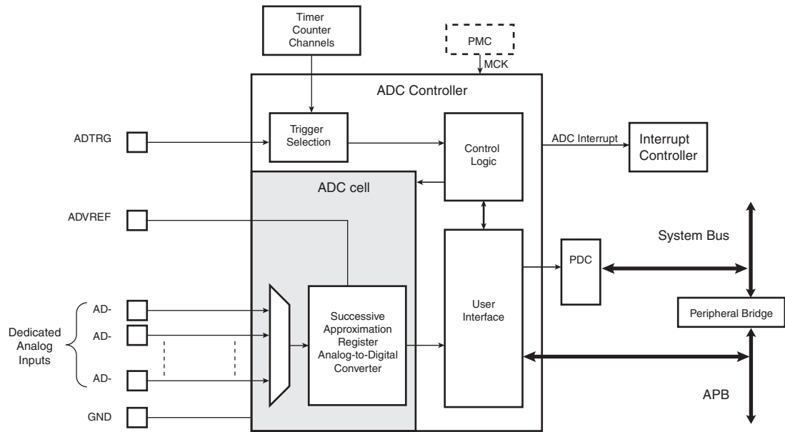
FIGURE 43-4: ANALOG-TO-DIGITAL CONVERTER BLOCK DIAGRAM
