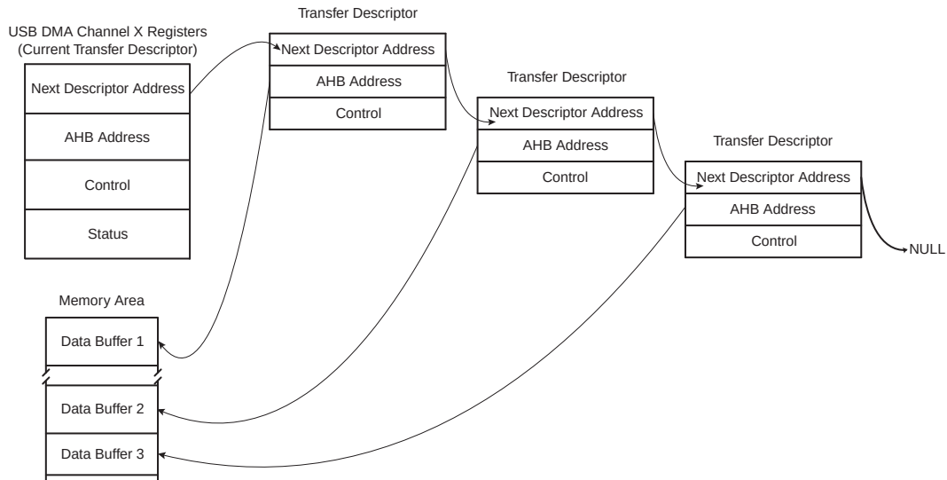
FIGURE 39-35: EXAMPLE OF DMA CHAINED LIST
