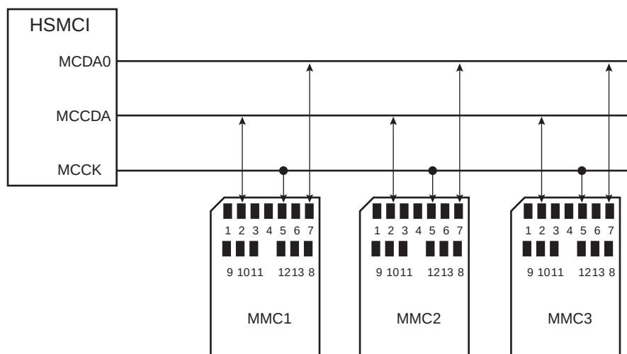
FIGURE 37-14: MMC BUS CONNECTIONS (ONE SLOT)
