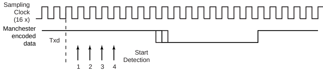
FIGURE 35-22: ASYNCHRONOUS START BIT DETECTION
