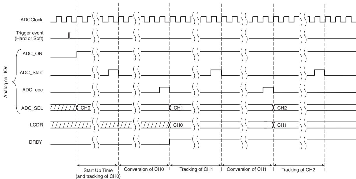
FIGURE 43-10: SEQUENCE OF ADC CONVERSIONS
