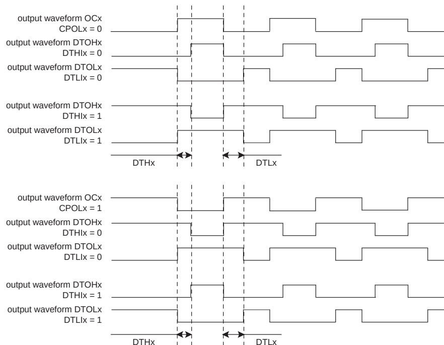
FIGURE 38-11: COMPLEMENTARY OUTPUT WAVEFORMS
