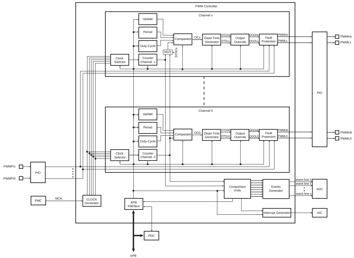
FIGURE 38-2: PULSE WIDTH MODULATION CONTROLLER BLOCK DIAGRAM
