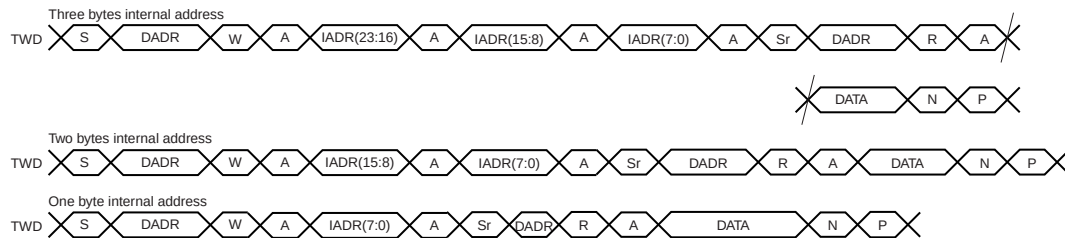
FIGURE 33-17: MASTER READ WITH ONE, TWO OR THREE BYTES INTERNAL ADDRESS AND ONE DATA BYTE
