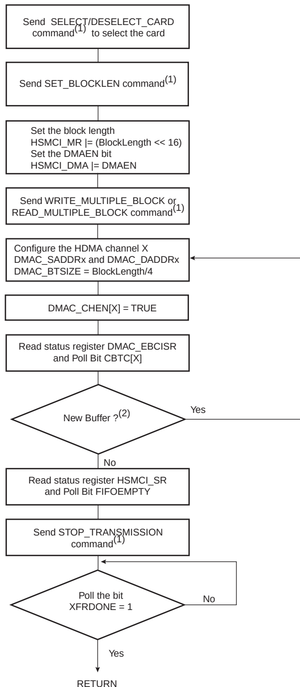
FIGURE 37-24: READ MULTIPLE BLOCK AND WRITE MULTIPLE BLOCK
