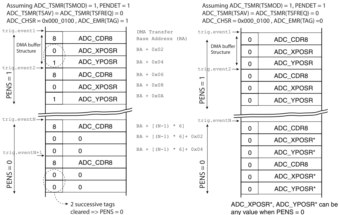
FIGURE 43-17: BUFFER STRUCTURE WITH AND WITHOUT PEN DETECTION ENABLED
