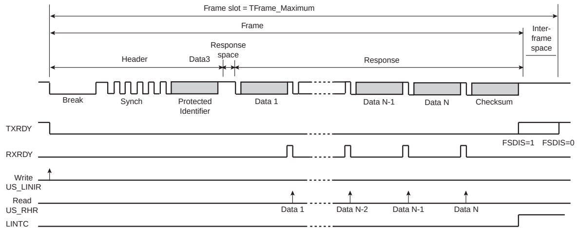
FIGURE 35-55: MASTER NODE CONFIGURATION, NACT=SUBSCRIBE
