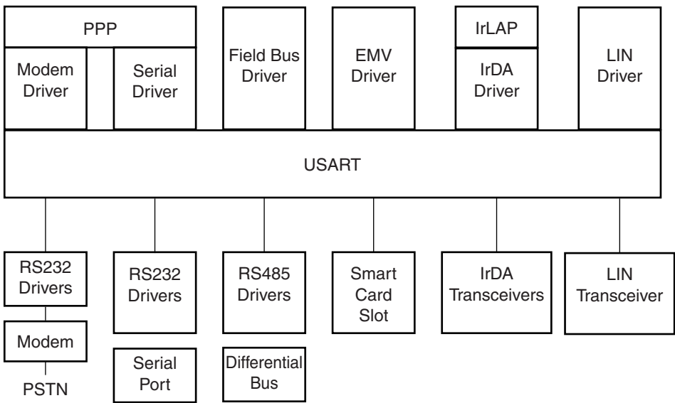
FIGURE 35-4: APPLICATION BLOCK DIAGRAM
