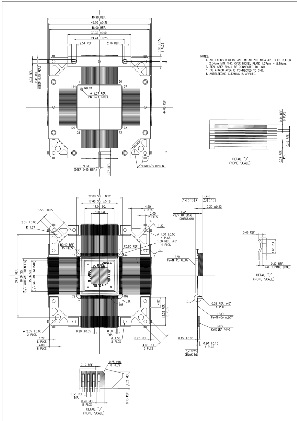
FIGURE 46-4: 144-LEAD CQFP PACKAGE DRAWING
