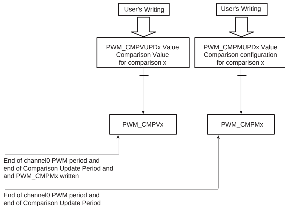
FIGURE 38-23: SYNCHRONIZED UPDATE OF COMPARISON VALUES AND CONFIGURATIONS
