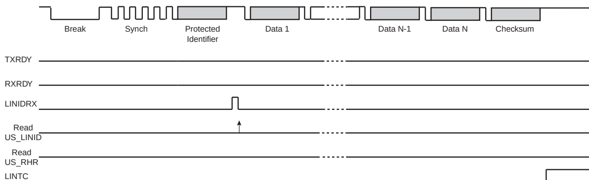
FIGURE 35-59: SLAVE NODE CONFIGURATION, NACT = IGNORE
