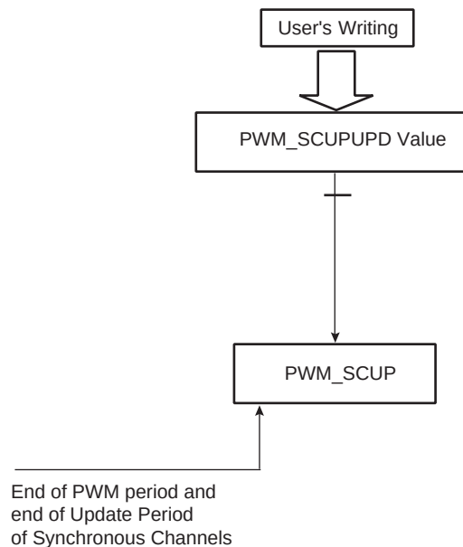
FIGURE 38-22: SYNCHRONIZED UPDATE OF UPDATE PERIOD VALUE OF SYNCHRONOUS CHANNELS
