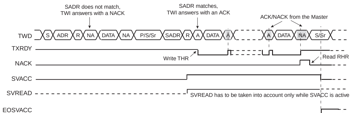
FIGURE 33-34: READ ACCESS ORDERED BY A MASTER
