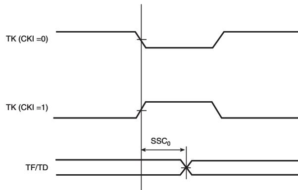
FIGURE 45-21: SSC TRANSMITTER, TK AND TF AS OUTPUT
