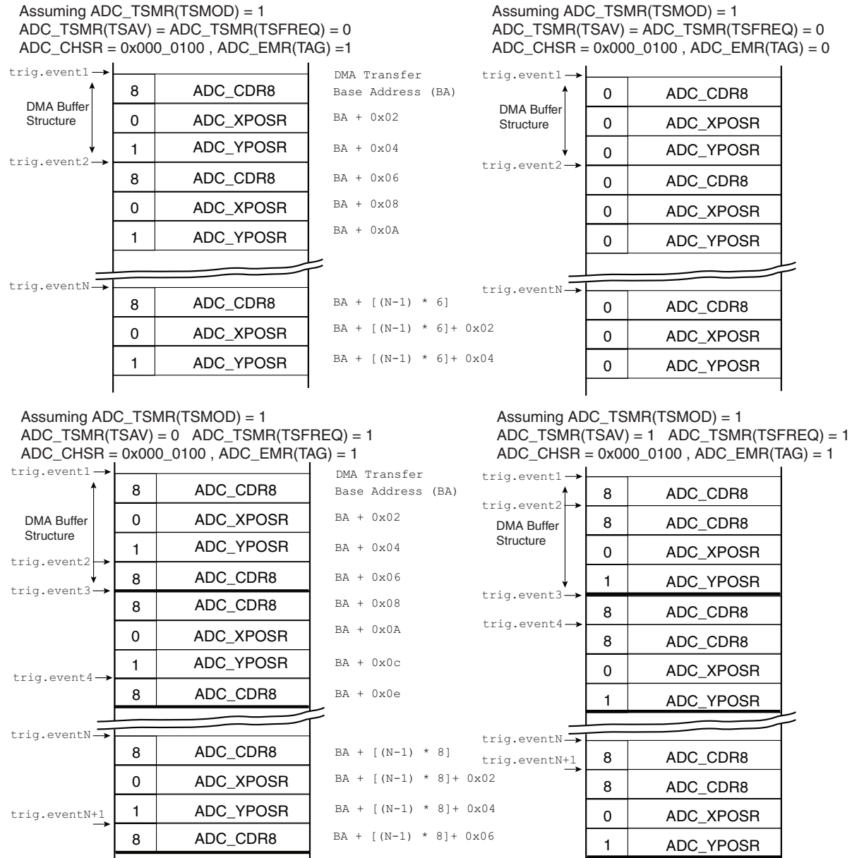
FIGURE 43-16: BUFFER STRUCTURE WHEN CLASSIC ADC AND TOUCHSCREEN CHANNELS
