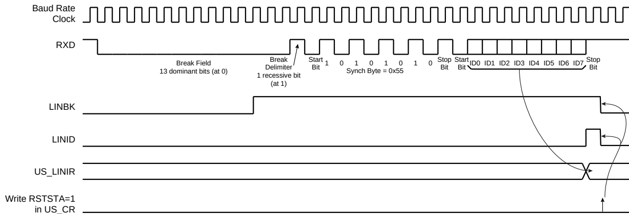
FIGURE 35-49: HEADER RECEPTION
