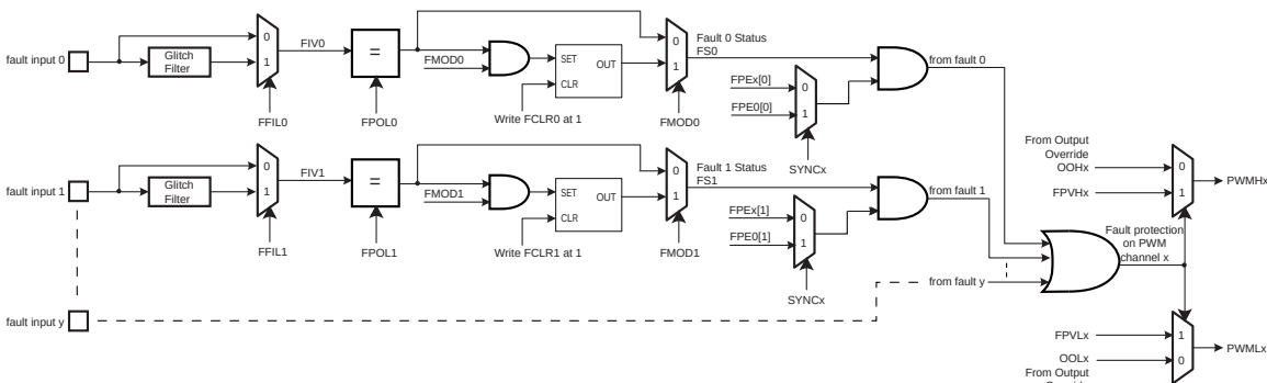
FIGURE 38-13: FAULT PROTECTION
