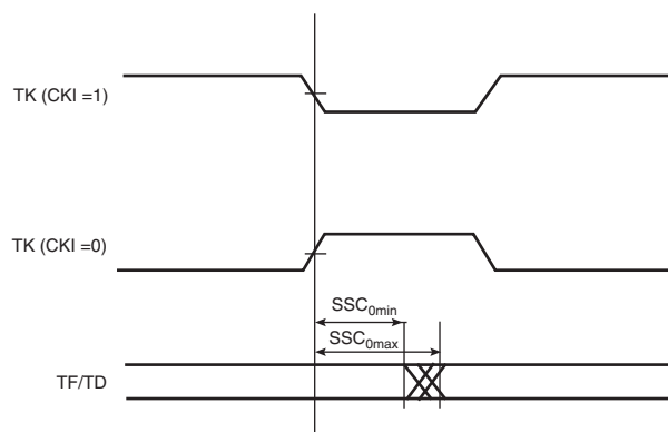
FIGURE 45-29: MIN AND MAX ACCESS TIME OF OUTPUT SIGNALS
