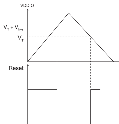
FIGURE 45-2: VDDUTMI SUPPLY MONITOR
