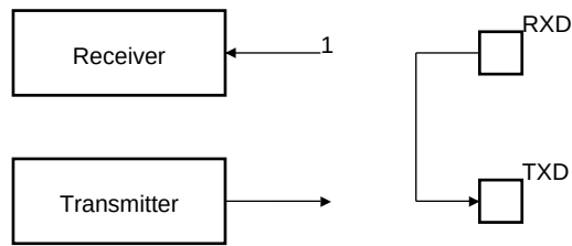
FIGURE 35-66: REMOTE LOOPBACK MODE CONFIGURATION
