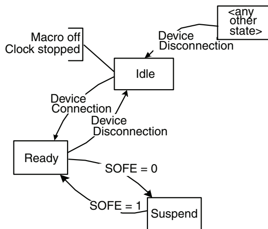
FIGURE 39-28: HOST MODE STATES
