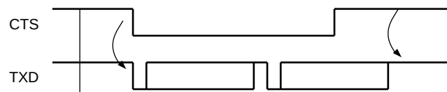
FIGURE 35-37: TRANSMITTER BEHAVIOR WHEN OPERATING WITH HARDWARE HANDSHAKING
