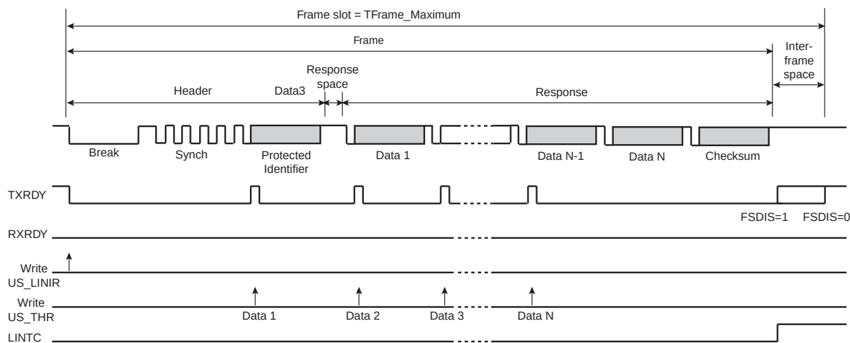
FIGURE 35-54: MASTER NODE CONFIGURATION, NACT = PUBLISH
