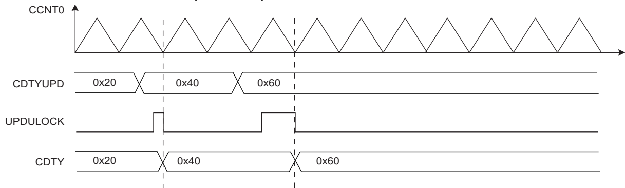
FIGURE 38-14: METHOD 1 (UPDM = 0)
