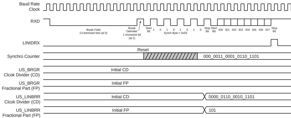
FIGURE 35-51: SLAVE NODE SYNCHRONIZATION
