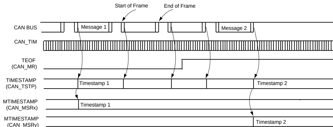
FIGURE 40-19: MAILBOX TIMESTAMP
