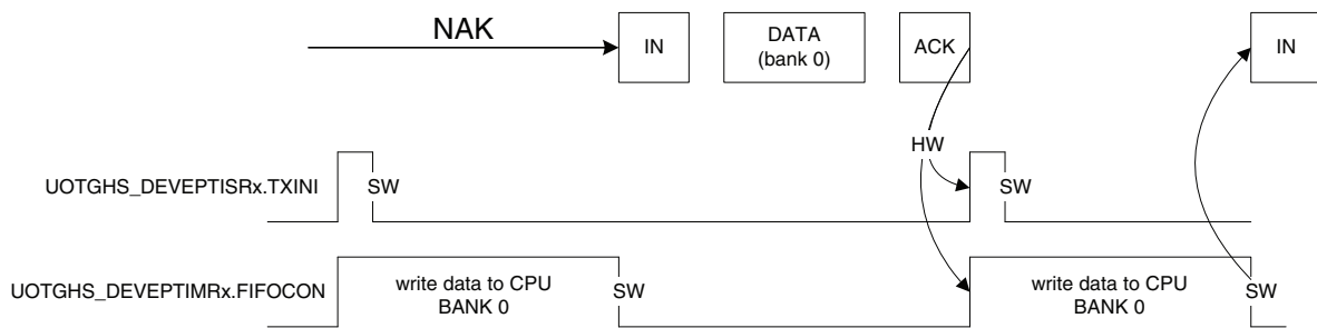
FIGURE 39-22: EXAMPLE OF AN IN ENDPOINT WITH 1 DATA BANK
