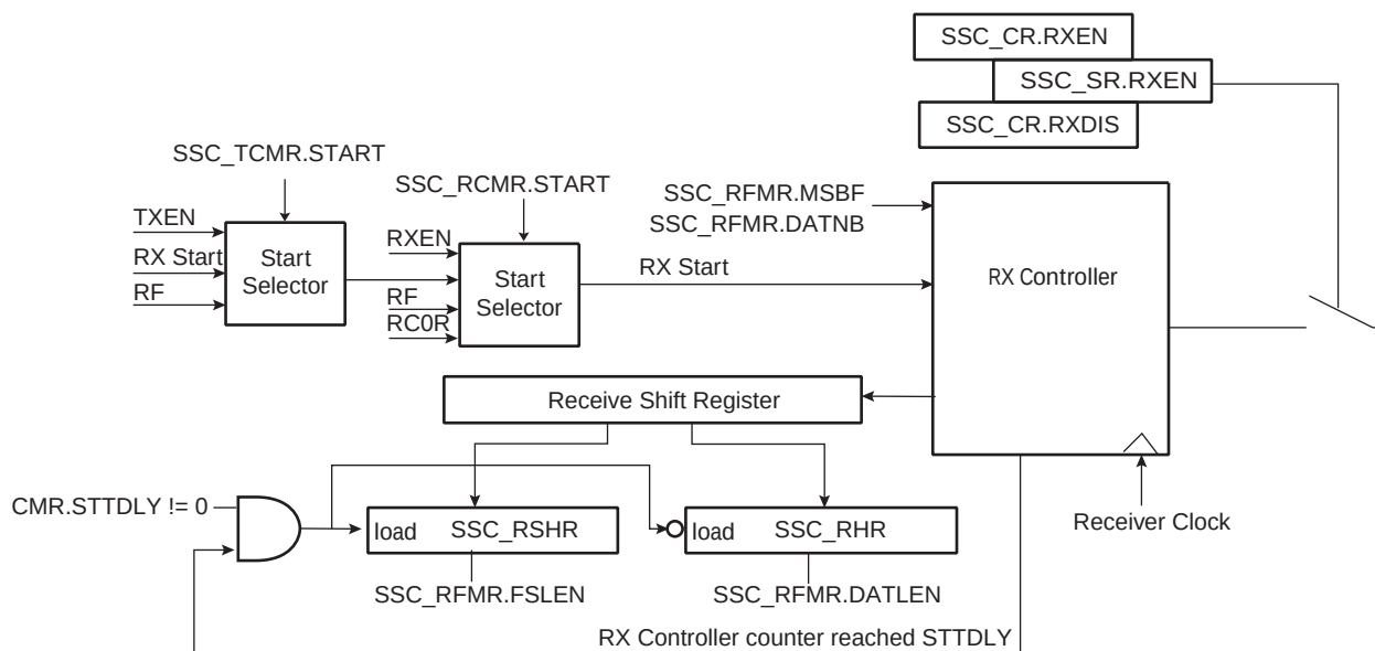
FIGURE 30-9: RECEIVER BLOCK DIAGRAM
