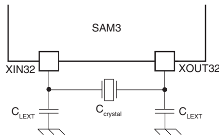
FIGURE 45-10: 32.768 KHZ CRYSTAL OSCILLATOR SCHEMATICS
