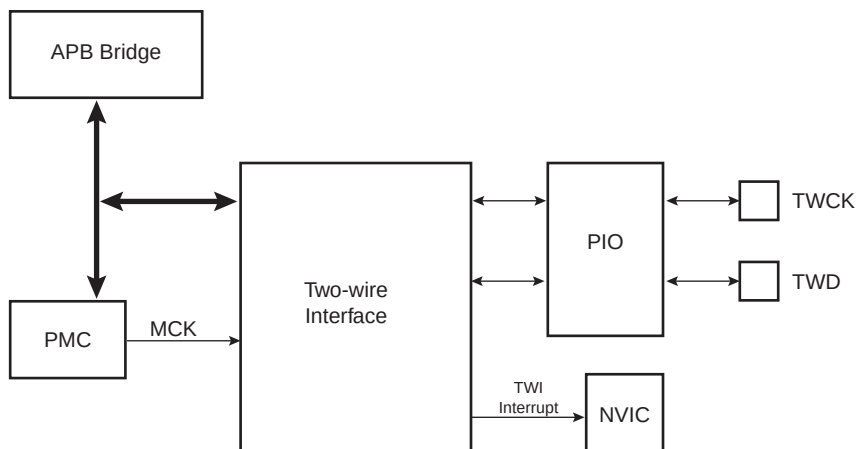
FIGURE 33-2: BLOCK DIAGRAM
