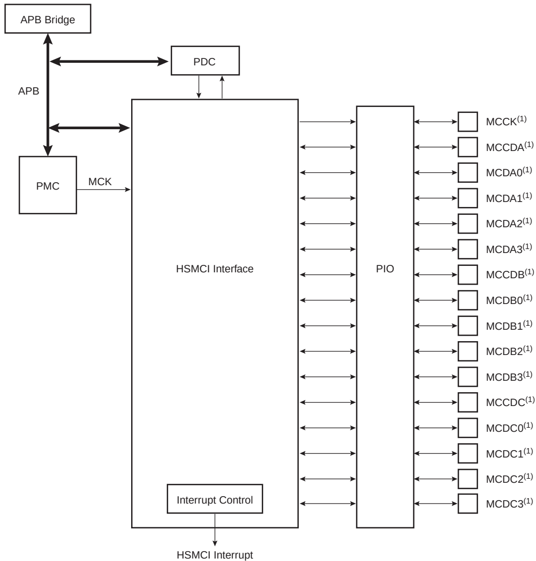
FIGURE 37-9: BLOCK DIAGRAM
