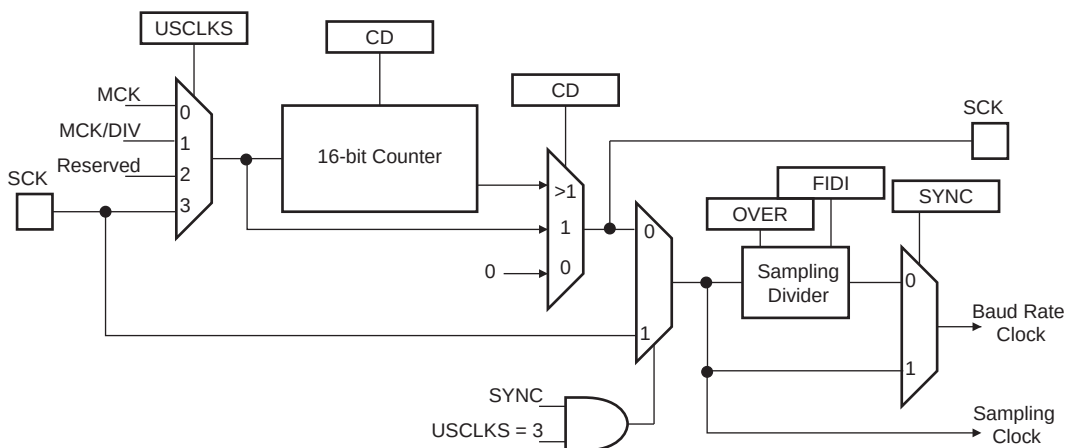
FIGURE 35-11: BAUD RATE GENERATOR
