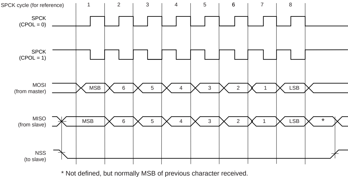
FIGURE 32-4: SPI TRANSFER FORMAT (NCPHA = 1, 8 BITS PER TRANSFER)
