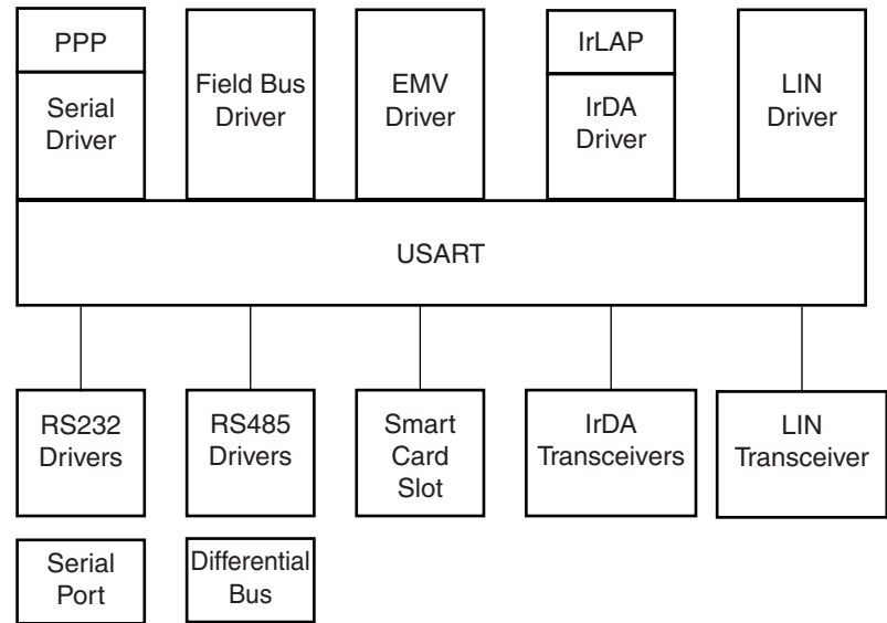
FIGURE 35-8: APPLICATION BLOCK DIAGRAM
