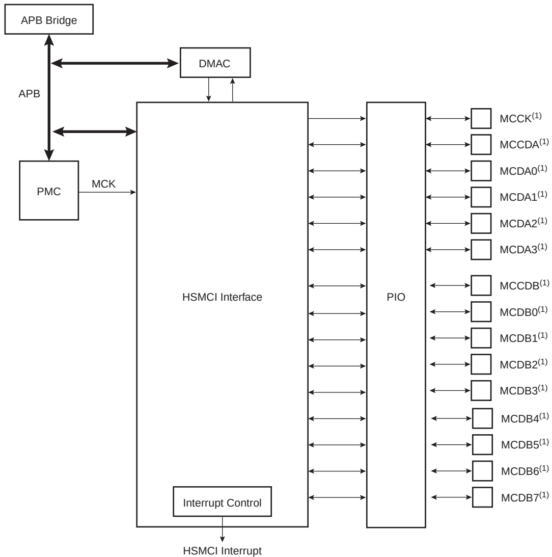
FIGURE 37-6: BLOCK DIAGRAM
