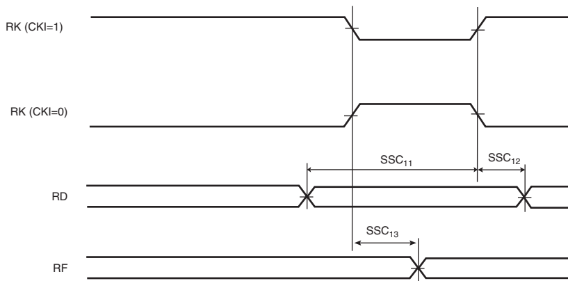
FIGURE 45-27: SSC RECEIVER, RK AND RF AS OUTPUT
