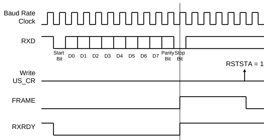
FIGURE 35-33: FRAMING ERROR STATUS
