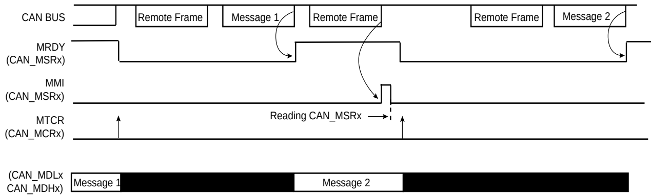
FIGURE 40-17: PRODUCER HANDLING
