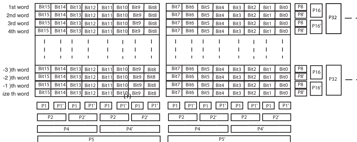
FIGURE 25-40: PARITY GENERATION FOR 512/1024/2048/4096 16-BIT WORDS
