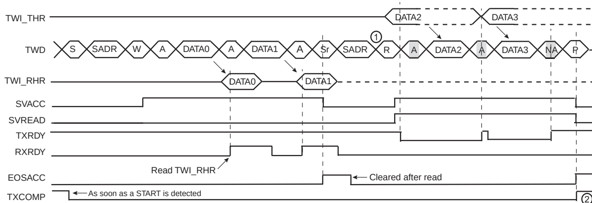
FIGURE 33-40: REPEATED START + REVERSAL FROM WRITE TO READ MODE
