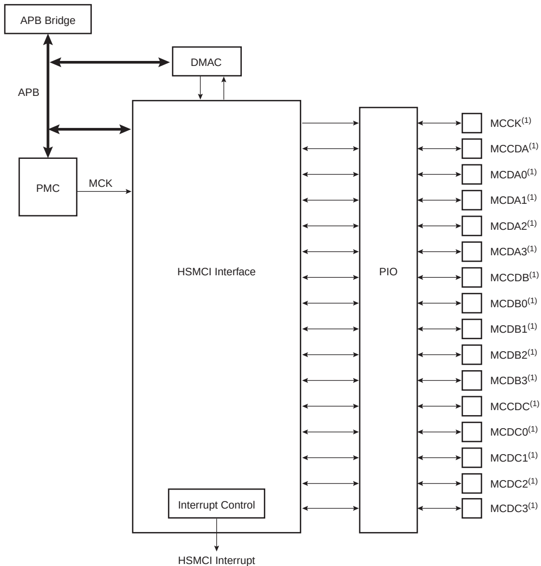
FIGURE 37-8: BLOCK DIAGRAM
