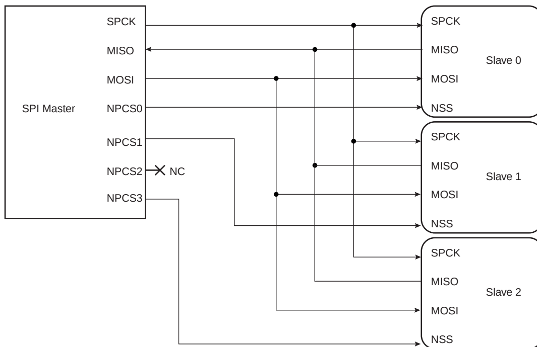
FIGURE 32-3: APPLICATION BLOCK DIAGRAM: SINGLE MASTER/MULTIPLE SLAVE IMPLEMENTATION
