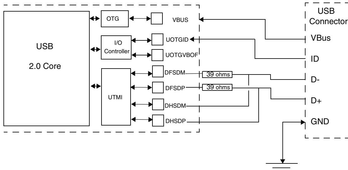
FIGURE 39-6: SELF-POWERED DEVICE APPLICATION BLOCK DIAGRAM
