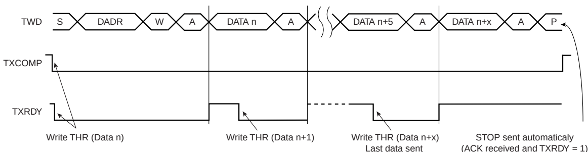
FIGURE 33-11: MASTER WRITE WITH MULTIPLE DATA BYTE
