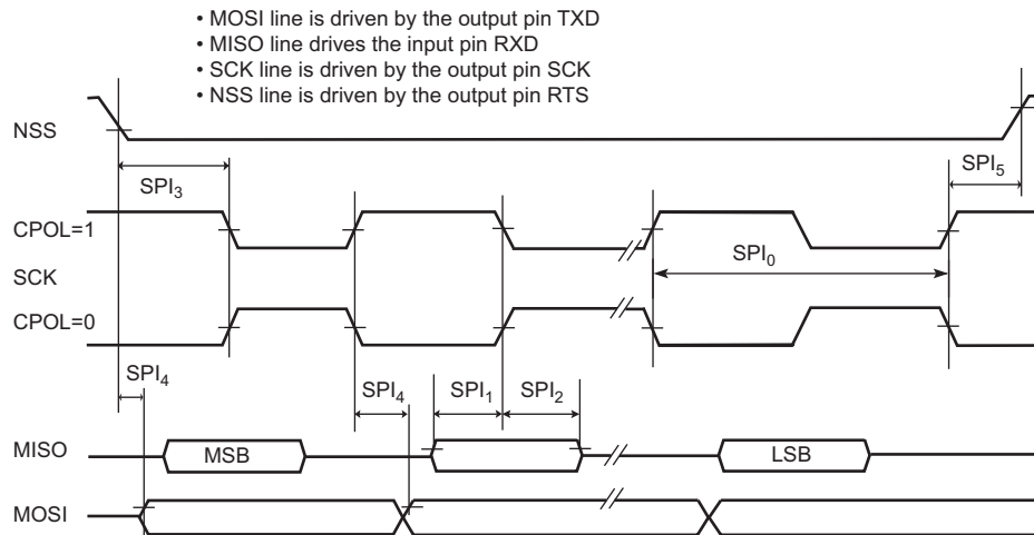
FIGURE 45-32: USART SPI MASTER MODE
