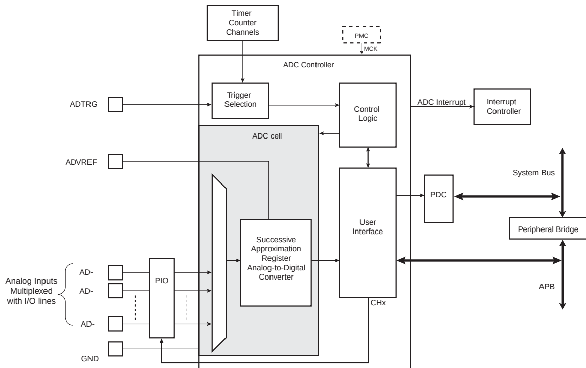
FIGURE 43-6: ANALOG-TO-DIGITAL CONVERTER BLOCK DIAGRAM
