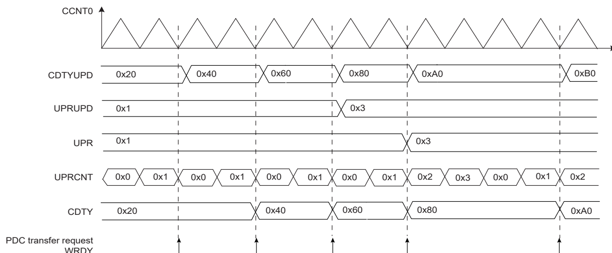
FIGURE 38-16: METHOD 3 (UPDM=2 AND PTRM=0)
