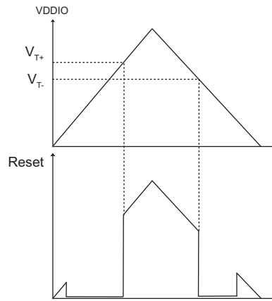
FIGURE 45-3: ZERO-POWER-ON RESET CHARACTERISTICS
