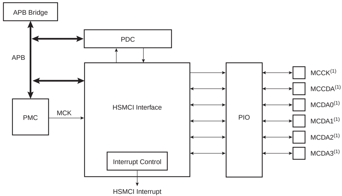
FIGURE 37-4: BLOCK DIAGRAM
