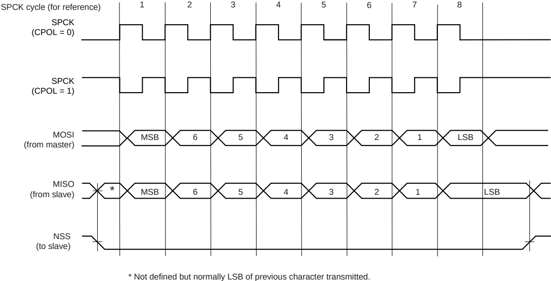
FIGURE 32-5: SPI TRANSFER FORMAT (NCPHA = 0, 8 BITS PER TRANSFER)
