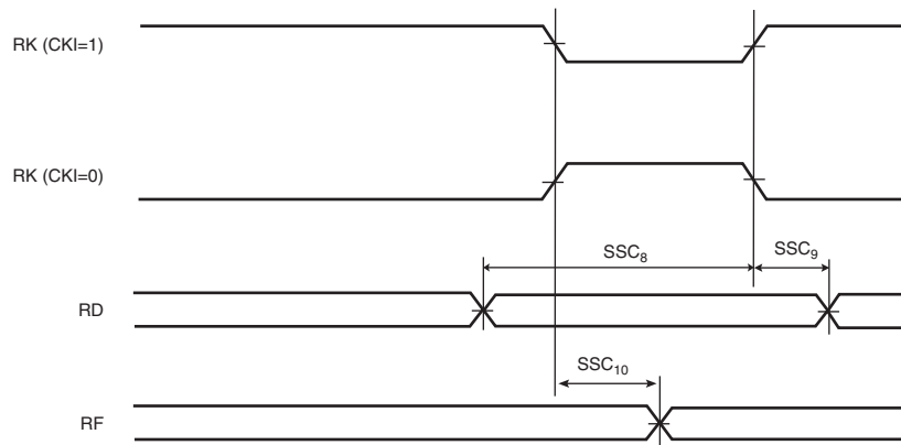
FIGURE 45-26: SSC RECEIVER, RK AS INPUT AND RF AS OUTPUT
