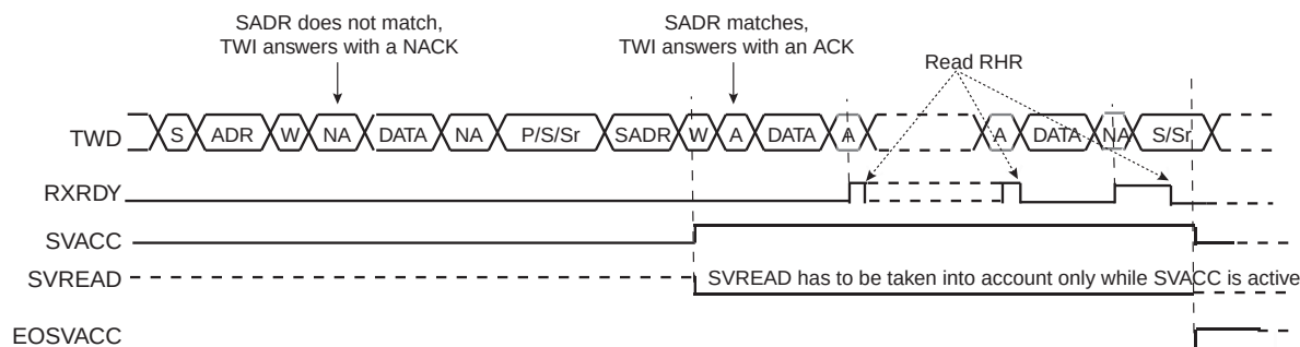
FIGURE 33-35: WRITE ACCESS ORDERED BY A MASTER
