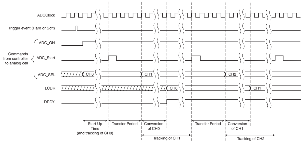
FIGURE 43-8: SEQUENCE OF ADC CONVERSIONS WHEN TRACKING TIME > CONVERSION TIME
