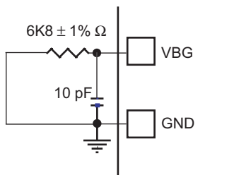
FIGURE 45-14: EXTERNAL CONNECTION OF VBG PIN
