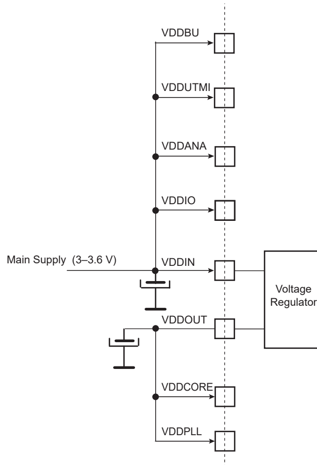
FIGURE 6-2: SINGLE SUPPLY
