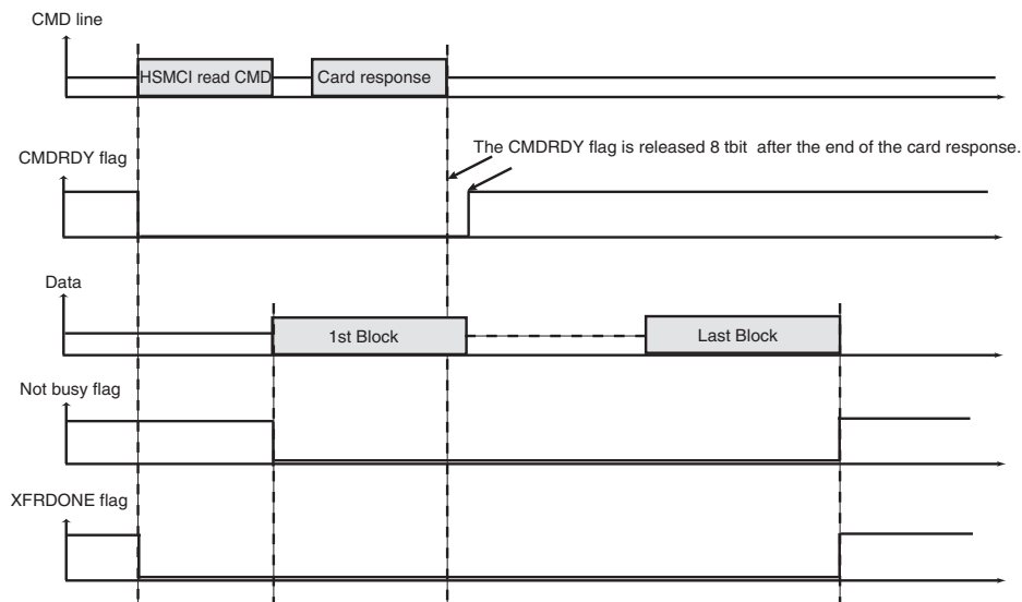
FIGURE 37-25: XFRDONE DURING A READ ACCESS
