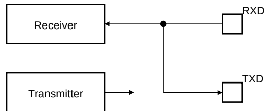
FIGURE 35-64: AUTOMATIC ECHO MODE CONFIGURATION
