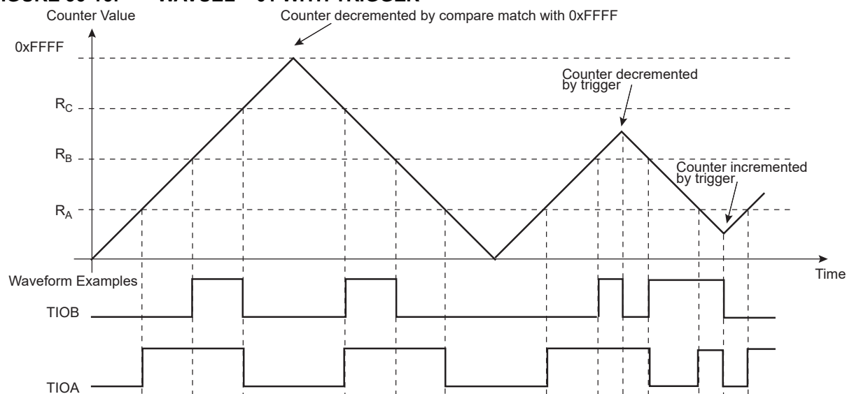
FIGURE 36-15: WAVSEL = 01 WITH TRIGGER
