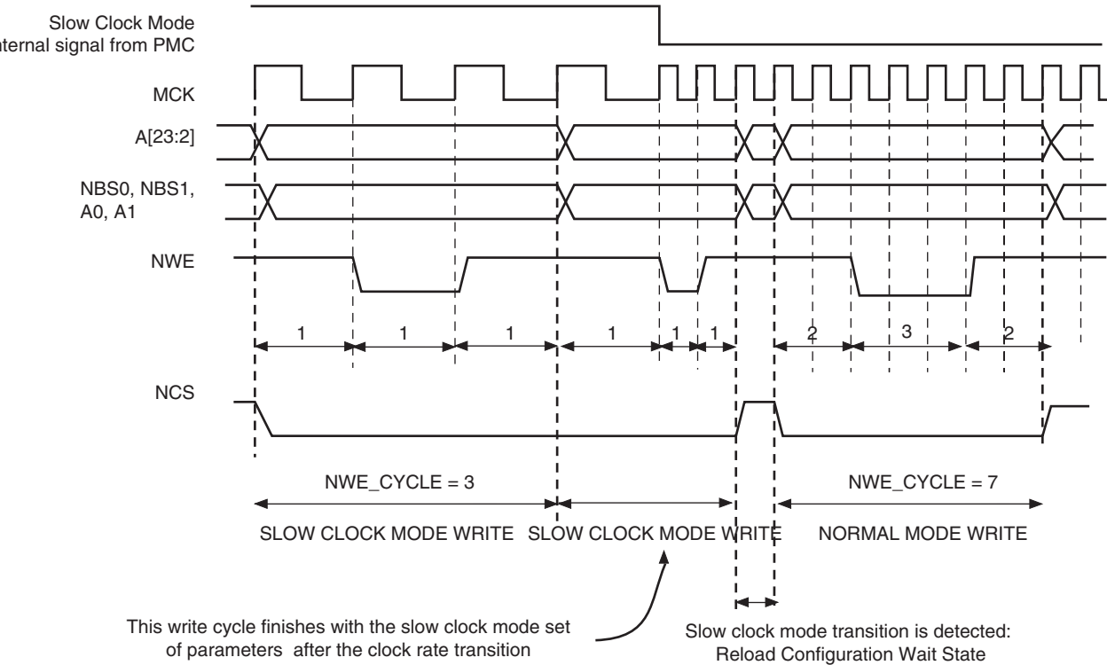
FIGURE 25-29: CLOCK RATE TRANSITION OCCURS WHILE THE SMC IS PERFORMING A WRITE OPERATION
