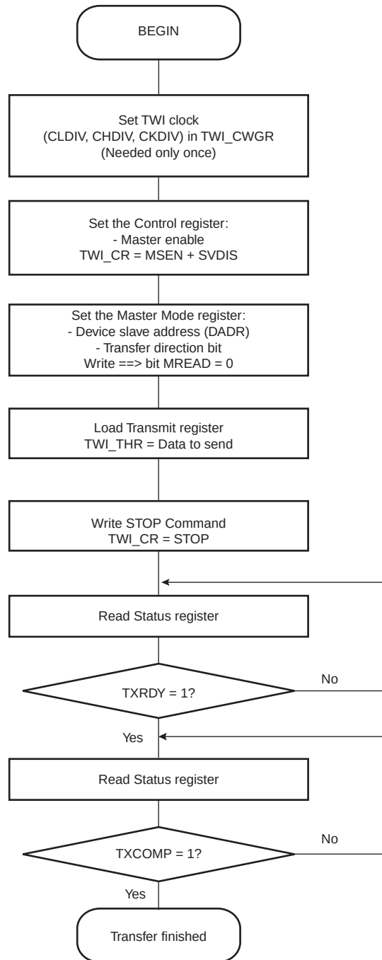
FIGURE 33-20: TWI WRITE OPERATION WITH SINGLE DATA BYTE WITHOUT INTERNAL ADDRESS
