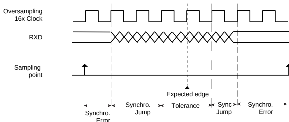
FIGURE 35-19: BIT RESYNCHRONIZATION
