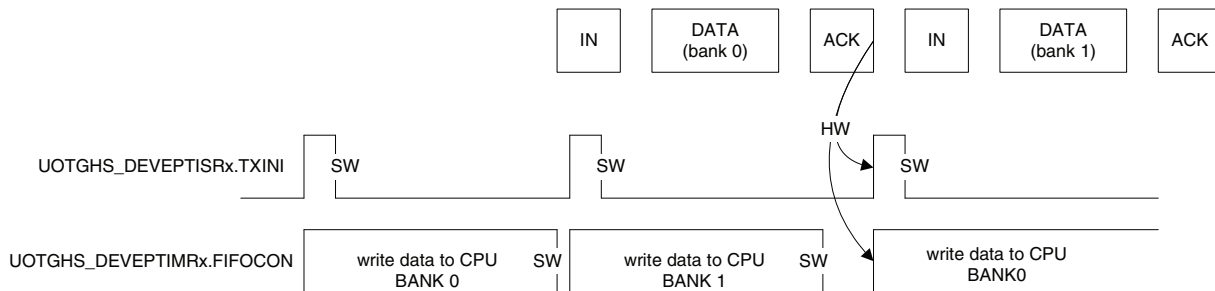
FIGURE 39-23: EXAMPLE OF AN IN ENDPOINT WITH 2 DATA BANKS
