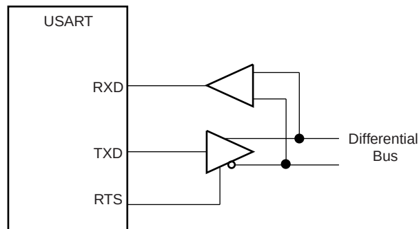
FIGURE 35-44: TYPICAL CONNECTION TO A RS485 BUS
