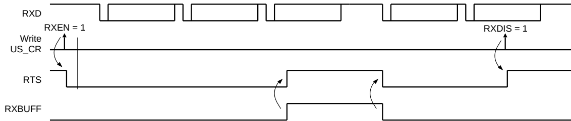
FIGURE 35-36: RECEIVER BEHAVIOR WHEN OPERATING WITH HARDWARE HANDSHAKING
