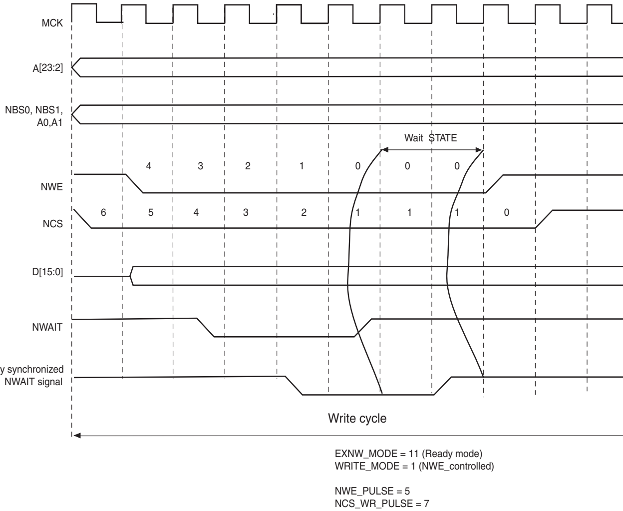
FIGURE 25-25: NWAIT ASSERTION IN WRITE ACCESS: READY MODE (EXNW_MODE = 11)
