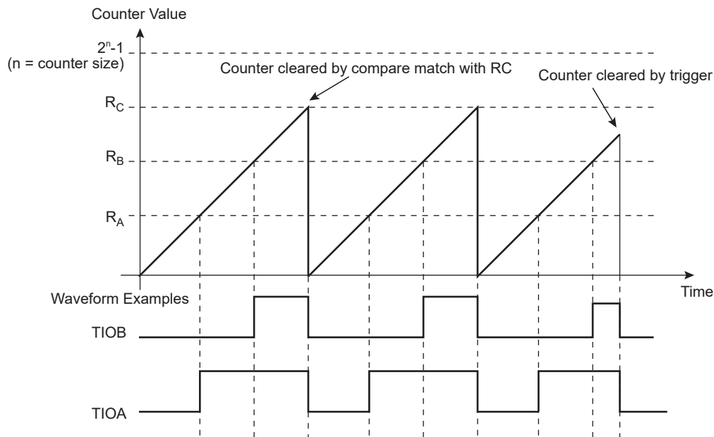
FIGURE 36-13: WAVSEL = 10 WITH TRIGGER
