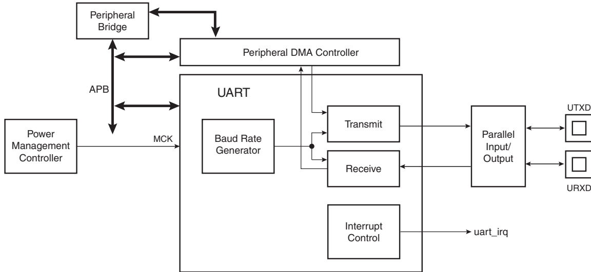
FIGURE 34-2: UART FUNCTIONAL BLOCK DIAGRAM
