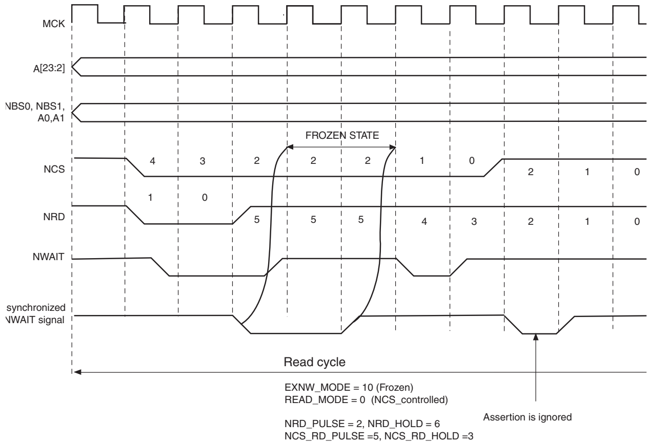
FIGURE 25-24: READ ACCESS WITH NWAIT ASSERTION IN FROZEN MODE (EXNW_MODE = 10)
