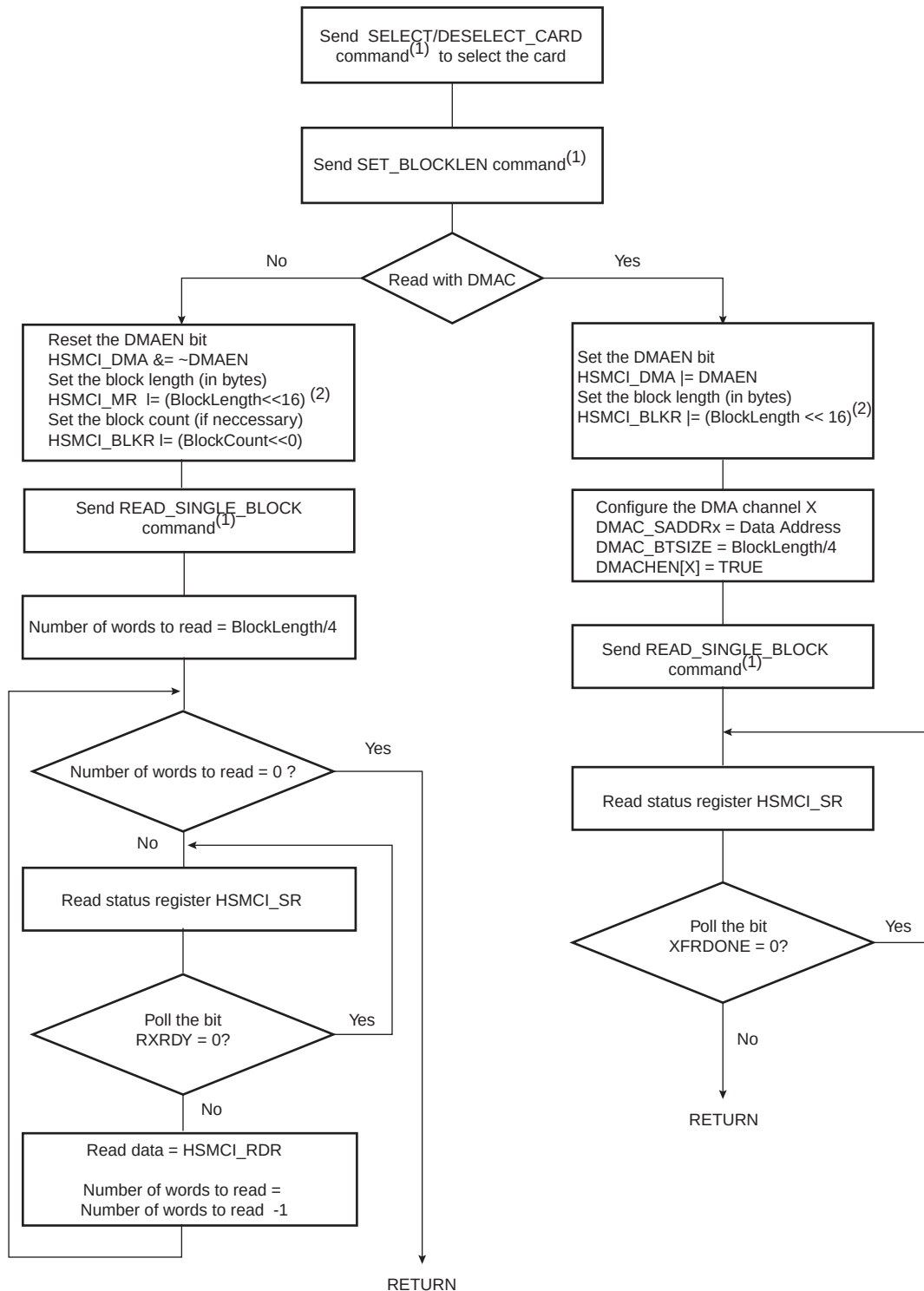
FIGURE 37-20: READ FUNCTIONAL FLOW DIAGRAM
