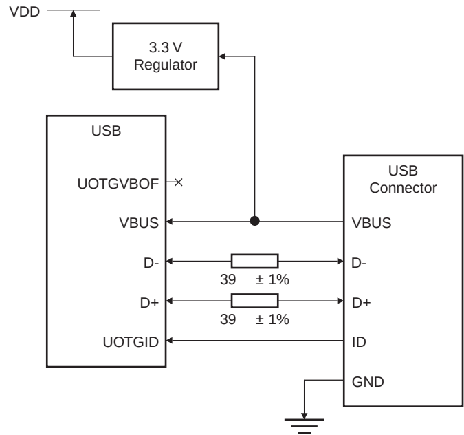
FIGURE 39-3: BUS-POWERED DEVICE APPLICATION BLOCK DIAGRAM
