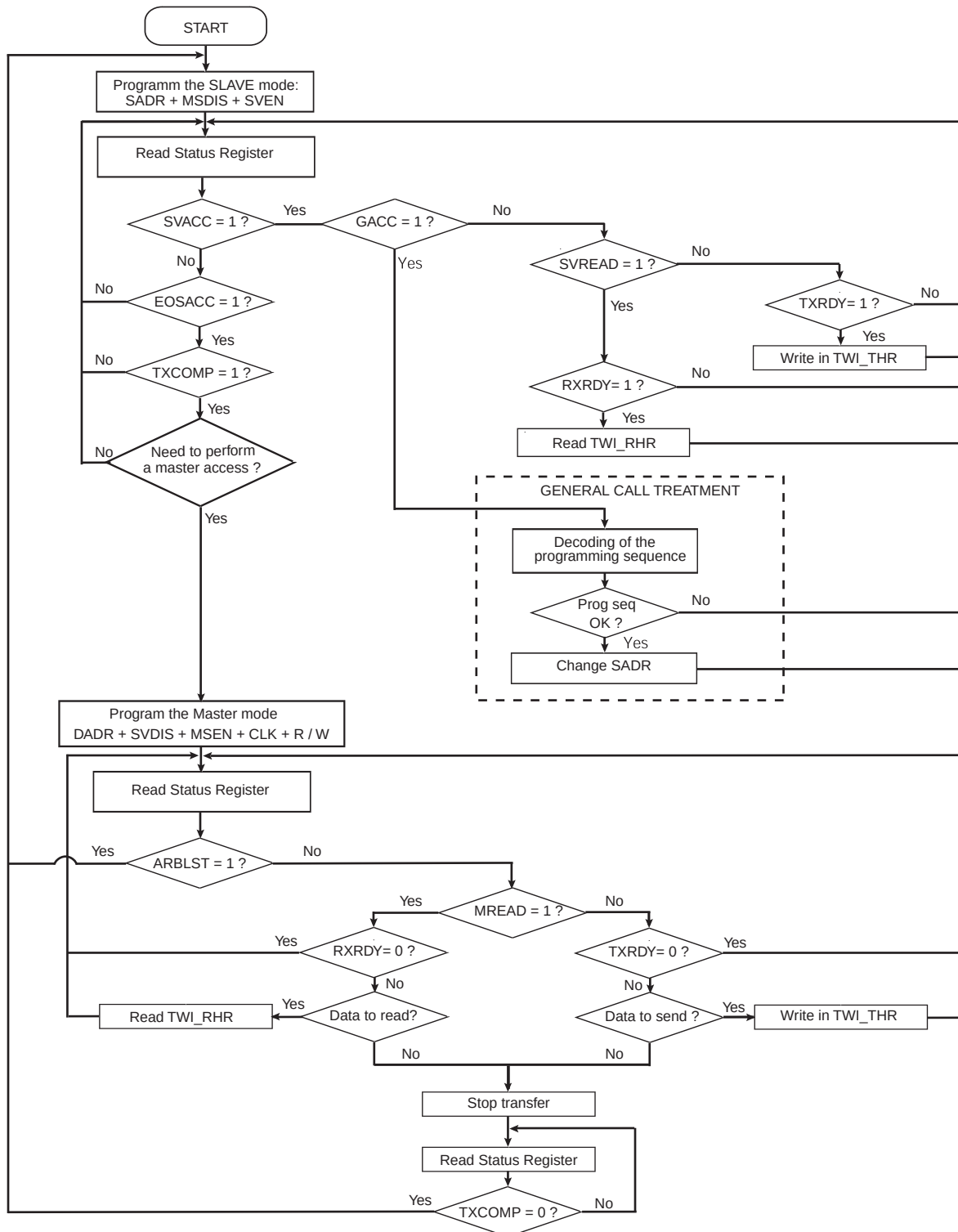
FIGURE 33-32: MULTI-MASTER FLOWCHART
