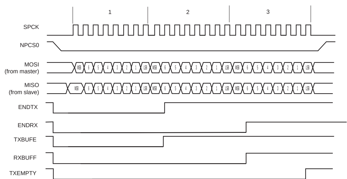
FIGURE 32-9: PDC STATUS REGISTER FLAGS BEHAVIOR
