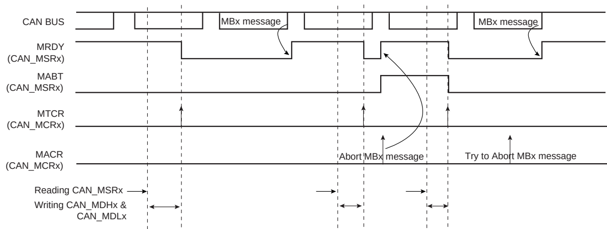
FIGURE 40-15: TRANSMITTING MESSAGES
