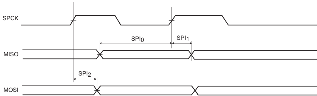
FIGURE 45-17: SPI MASTER MODE WITH (CPOL = NCPHA = 0) OR (CPOL = NCPHA = 1)
