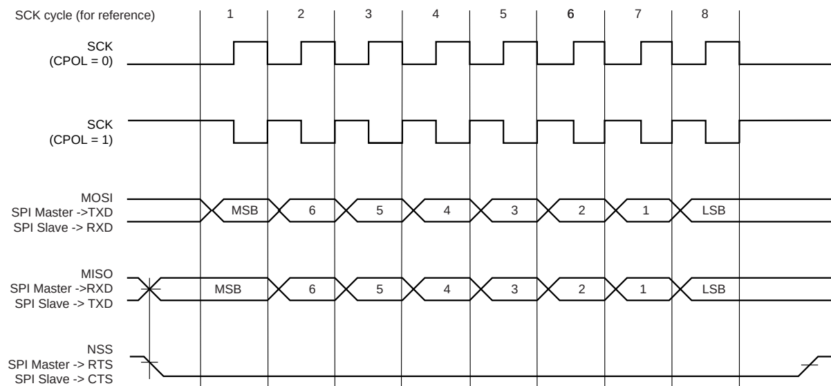
FIGURE 35-46: SPI TRANSFER FORMAT (CPHA=1, 8 BITS PER TRANSFER)
