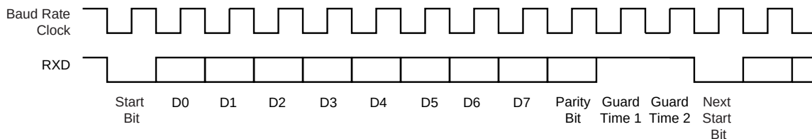
FIGURE 35-39: T = 0 PROTOCOL WITHOUT PARITY ERROR
