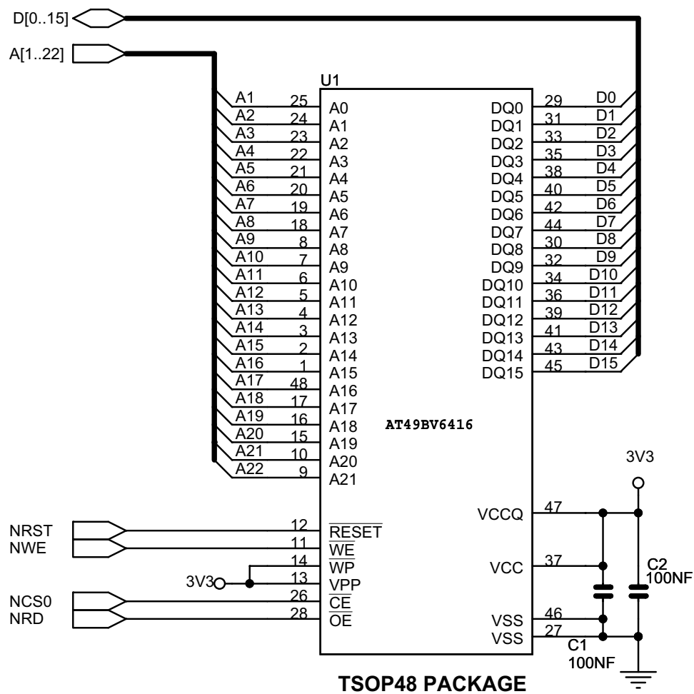
FIGURE 24-3: NOR FLASH ON NCS0 HARDWARE CONFIGURATION
