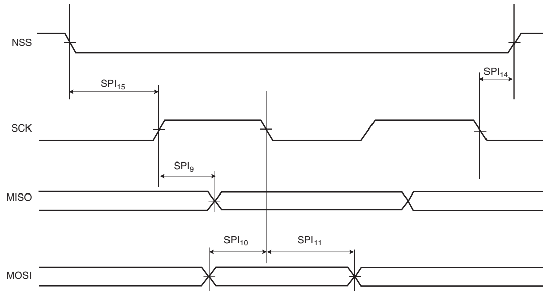
FIGURE 45-34: USART SPI SLAVE MODE (MODE 0 OR 3)
