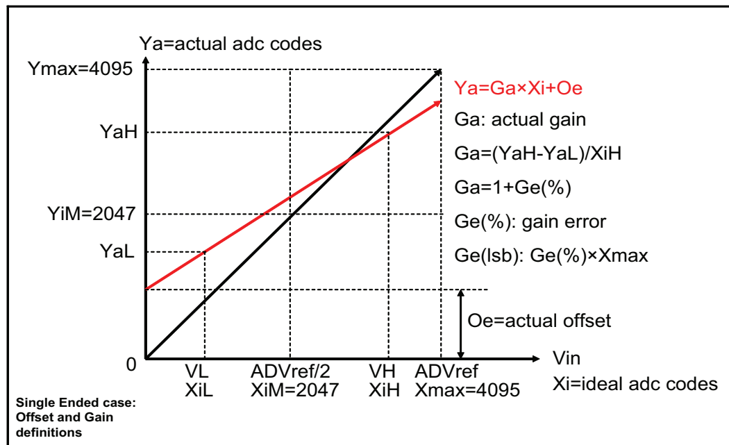
FIGURE 45-15: OFFSET AND GAIN DEFINITIONS
