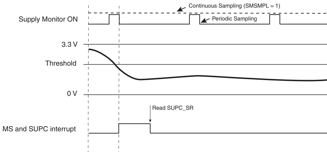
FIGURE 17-4: SUPPLY MONITOR STATUS BIT AND ASSOCIATED INTERRUPT
