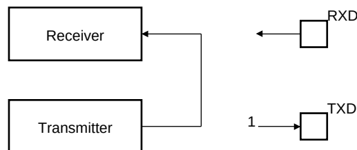
FIGURE 35-65: LOCAL LOOPBACK MODE CONFIGURATION
