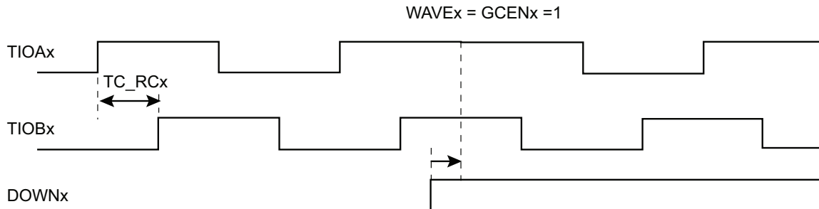
FIGURE 36-25: 2-BIT GRAY UP/DOWN COUNTER
