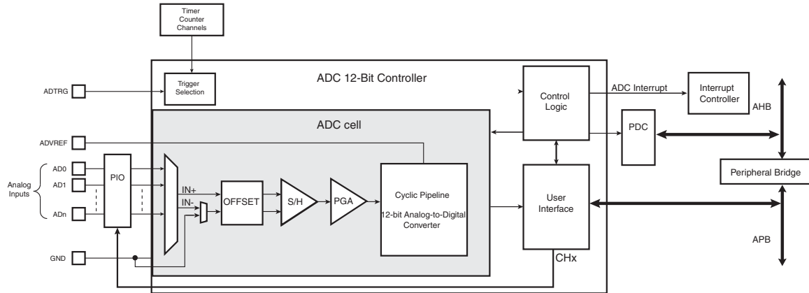
FIGURE 43-1: ANALOG-TO-DIGITAL CONVERTER BLOCK DIAGRAM
