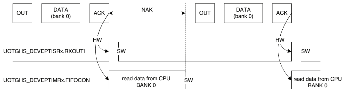
FIGURE 39-25: EXAMPLE OF AN OUT ENDPOINT WITH ONE DATA BANK
