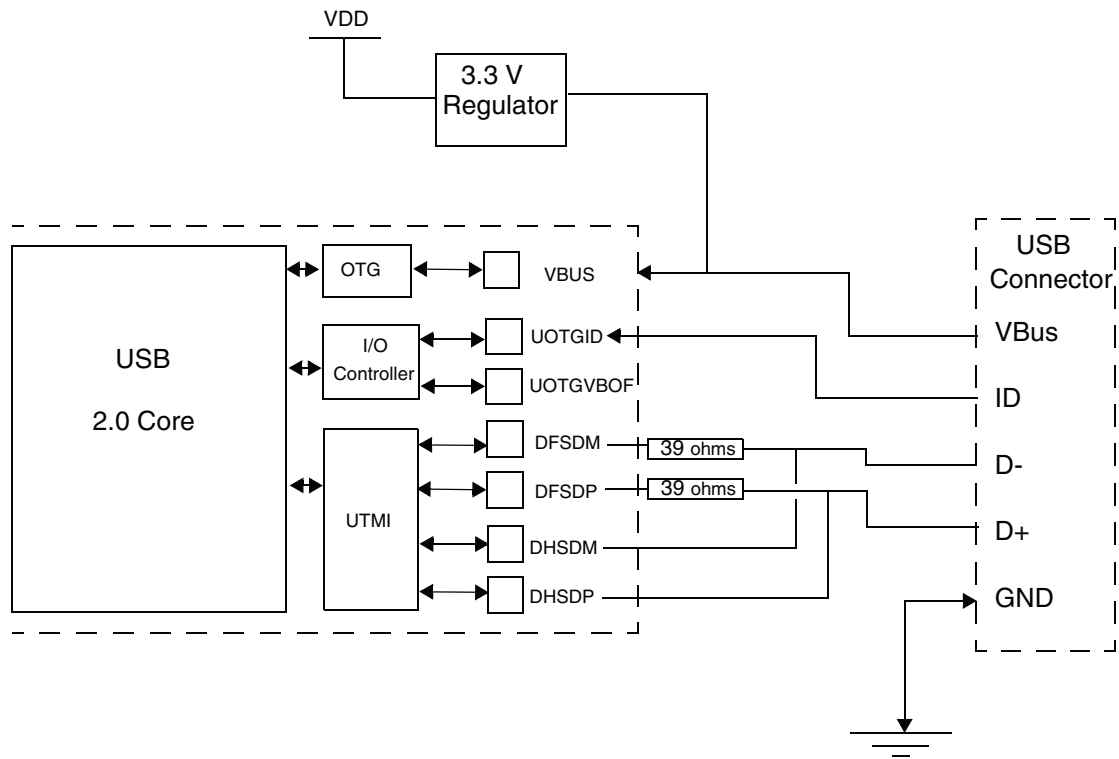
FIGURE 39-4: BUS-POWERED DEVICE APPLICATION BLOCK DIAGRAM
