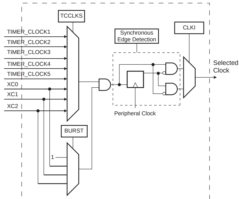
FIGURE 36-4: CLOCK SELECTION
