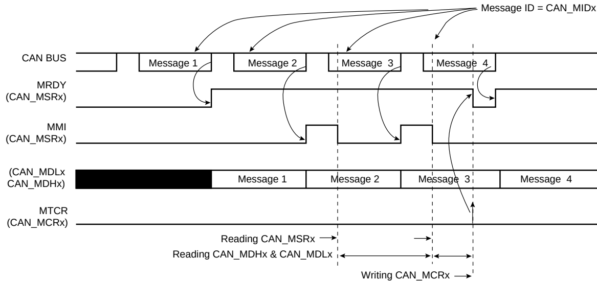
FIGURE 40-12: RECEIVE WITH OVERWRITE MAILBOX
