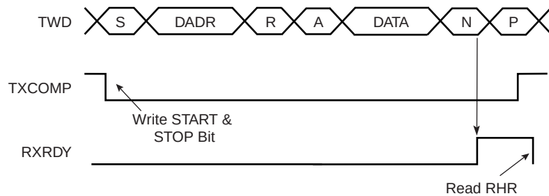
FIGURE 33-13: MASTER READ WITH ONE DATA BYTE
