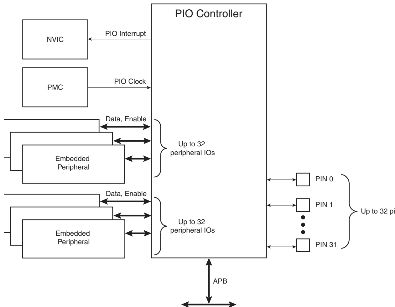
FIGURE 31-1: BLOCK DIAGRAM
