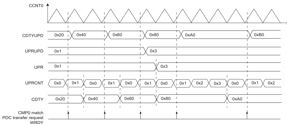
FIGURE 38-17: METHOD 3 (UPDM=2 AND PTRM=1 AND PTRCS=0)
