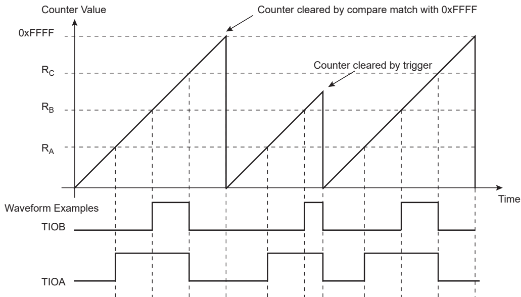
FIGURE 36-11: WAVSEL = 00 WITH TRIGGER
