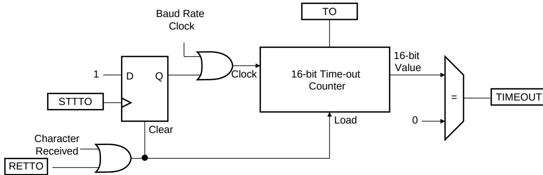
FIGURE 35-32: RECEIVER TIME-OUT BLOCK DIAGRAM
