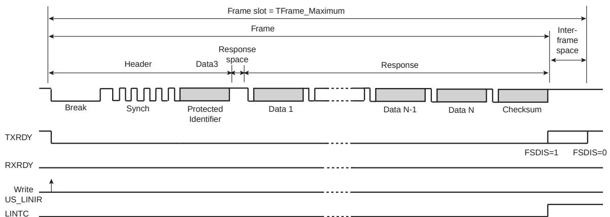
FIGURE 35-56: MASTER NODE CONFIGURATION, NACT=IGNORE
