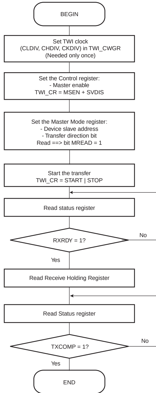
FIGURE 33-26: TWI READ OPERATION WITH SINGLE DATA BYTE WITHOUT INTERNAL ADDRESS
