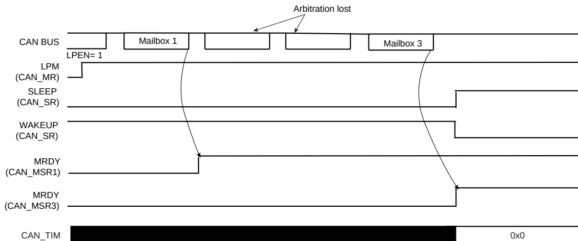
FIGURE 40-8: ENABLING LOW-POWER MODE
