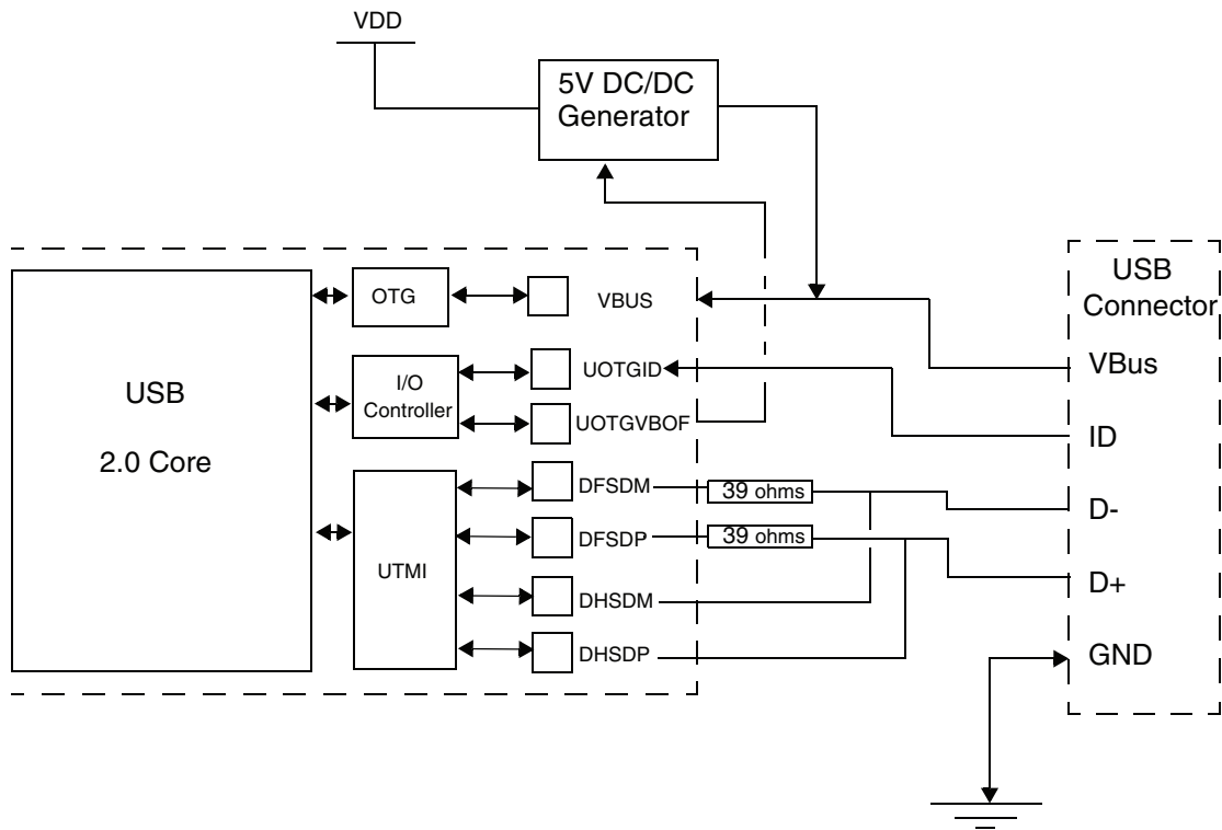
FIGURE 39-8: HOST AND OTG APPLICATION BLOCK DIAGRAM
