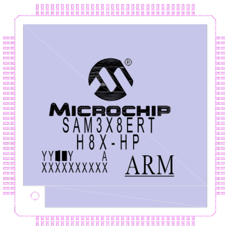
FIGURE 47-1: LQFP144
