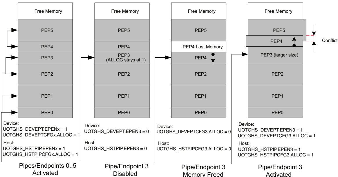
FIGURE 39-13: ALLOCATION AND REORGANIZATION OF THE DPRAM
