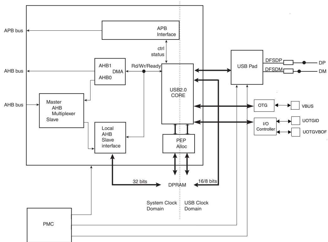
FIGURE 39-2: UOTGHS BLOCK DIAGRAM
