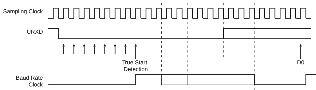
FIGURE 34-4: START BIT DETECTION
