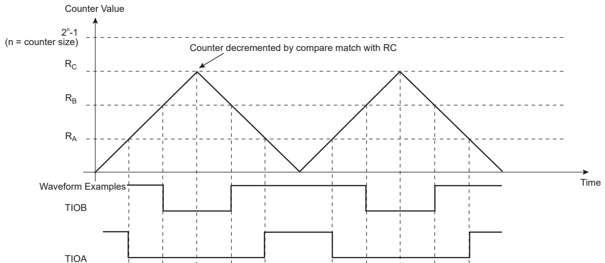
FIGURE 36-16: WAVSEL = 11 WITHOUT TRIGGER
