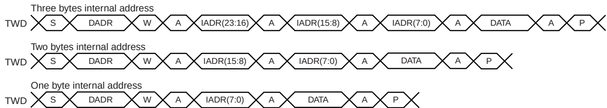
FIGURE 33-16: MASTER WRITE WITH ONE, TWO OR THREE BYTES INTERNAL ADDRESS AND ONE DATA BYTE
