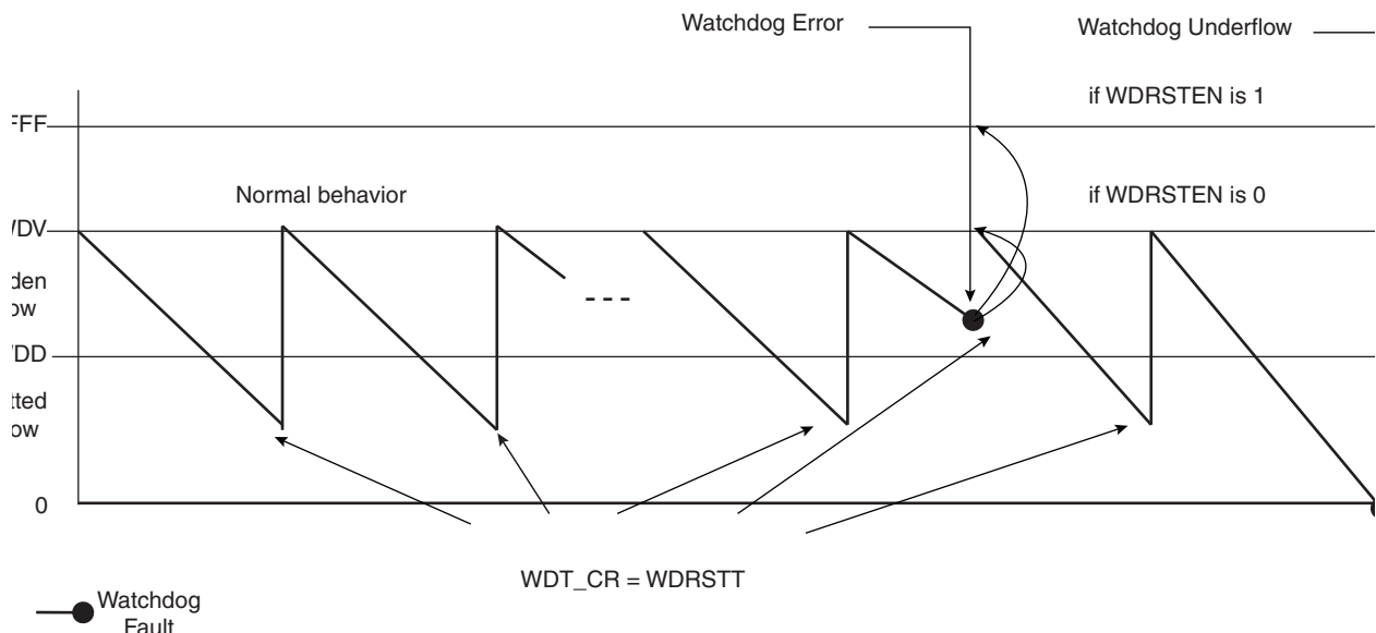
FIGURE 16-2: WATCHDOG BEHAVIOR
