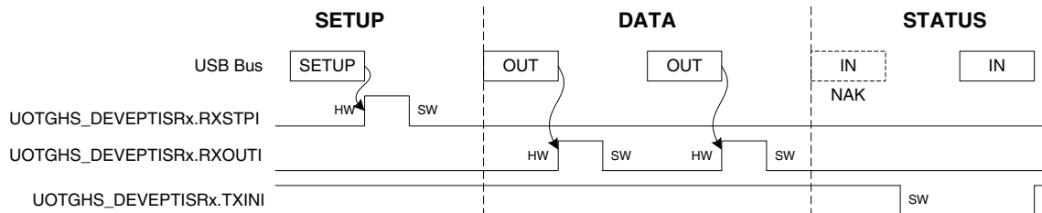
FIGURE 39-20: CONTROL WRITE
