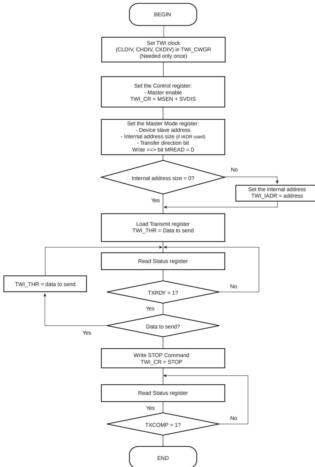
FIGURE 33-22: TWI WRITE OPERATION WITH MULTIPLE DATA BYTES WITH OR WITHOUT INTERNAL ADDRESS
