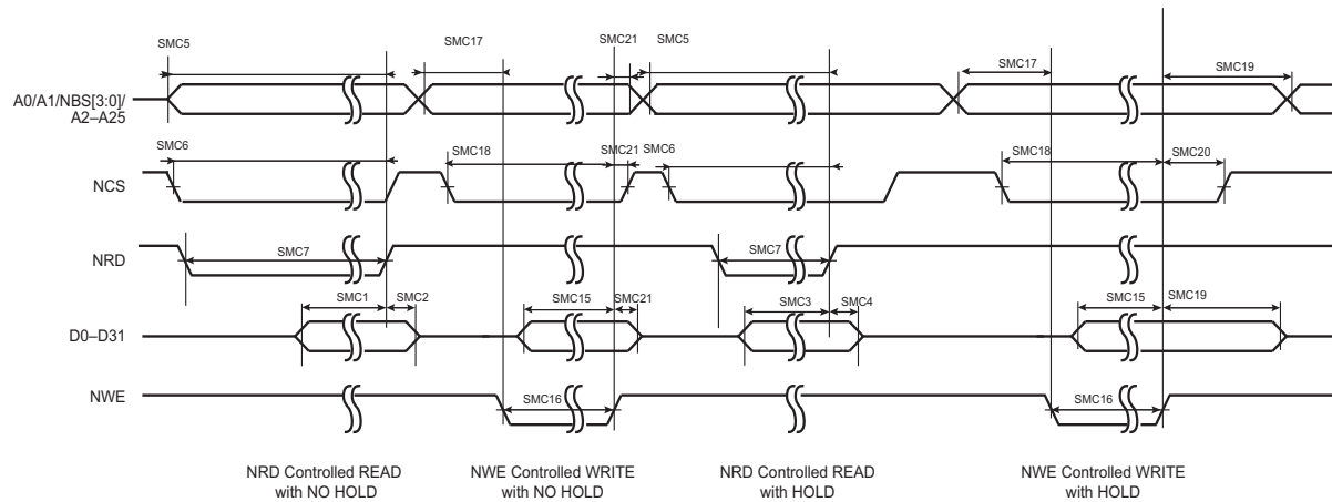
FIGURE 45-31: SMC TIMINGS - NRD CONTROLLED READ AND NWE CONTROLLED WRITE
