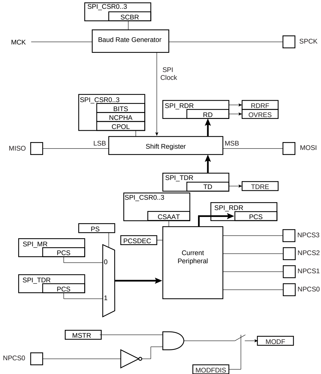
FIGURE 32-6: MASTER MODE BLOCK DIAGRAM
