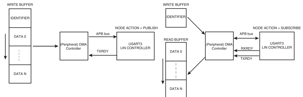
FIGURE 35-61: MASTER NODE WITH PDC (PDCM = 0)
