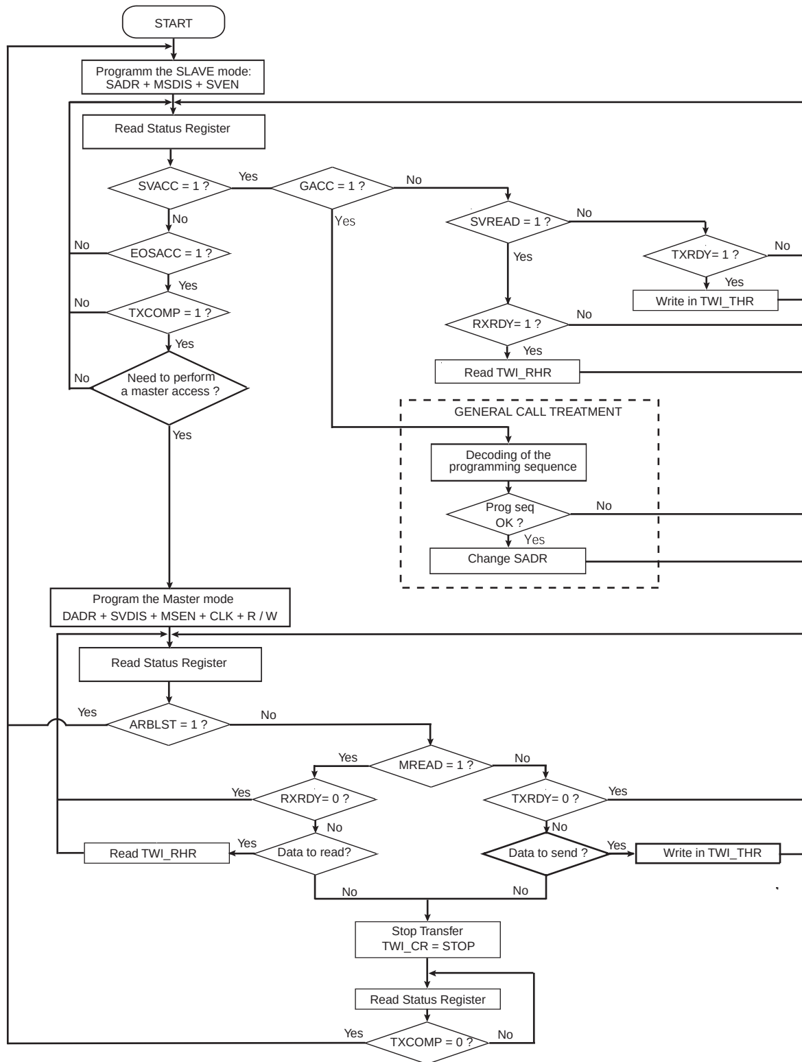
FIGURE 33-31: MULTI-MASTER FLOWCHART
