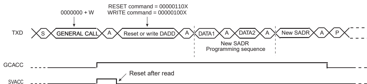
FIGURE 33-36: MASTER PERFORMS A GENERAL CALL
