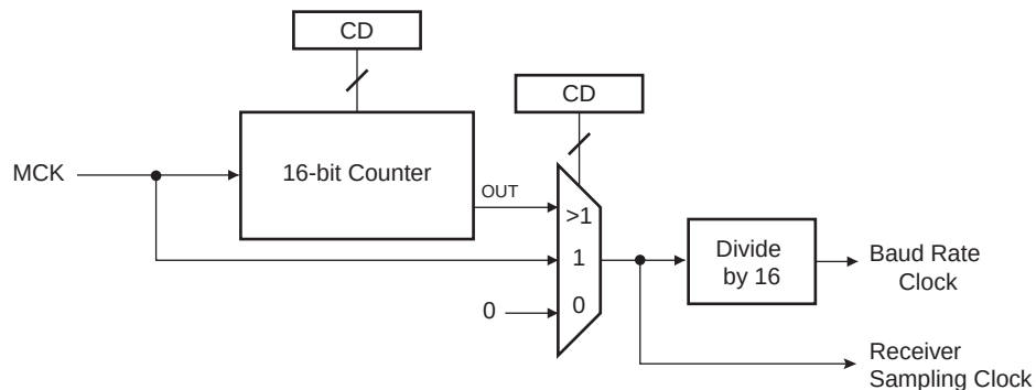
FIGURE 34-3: BAUD RATE GENERATOR
