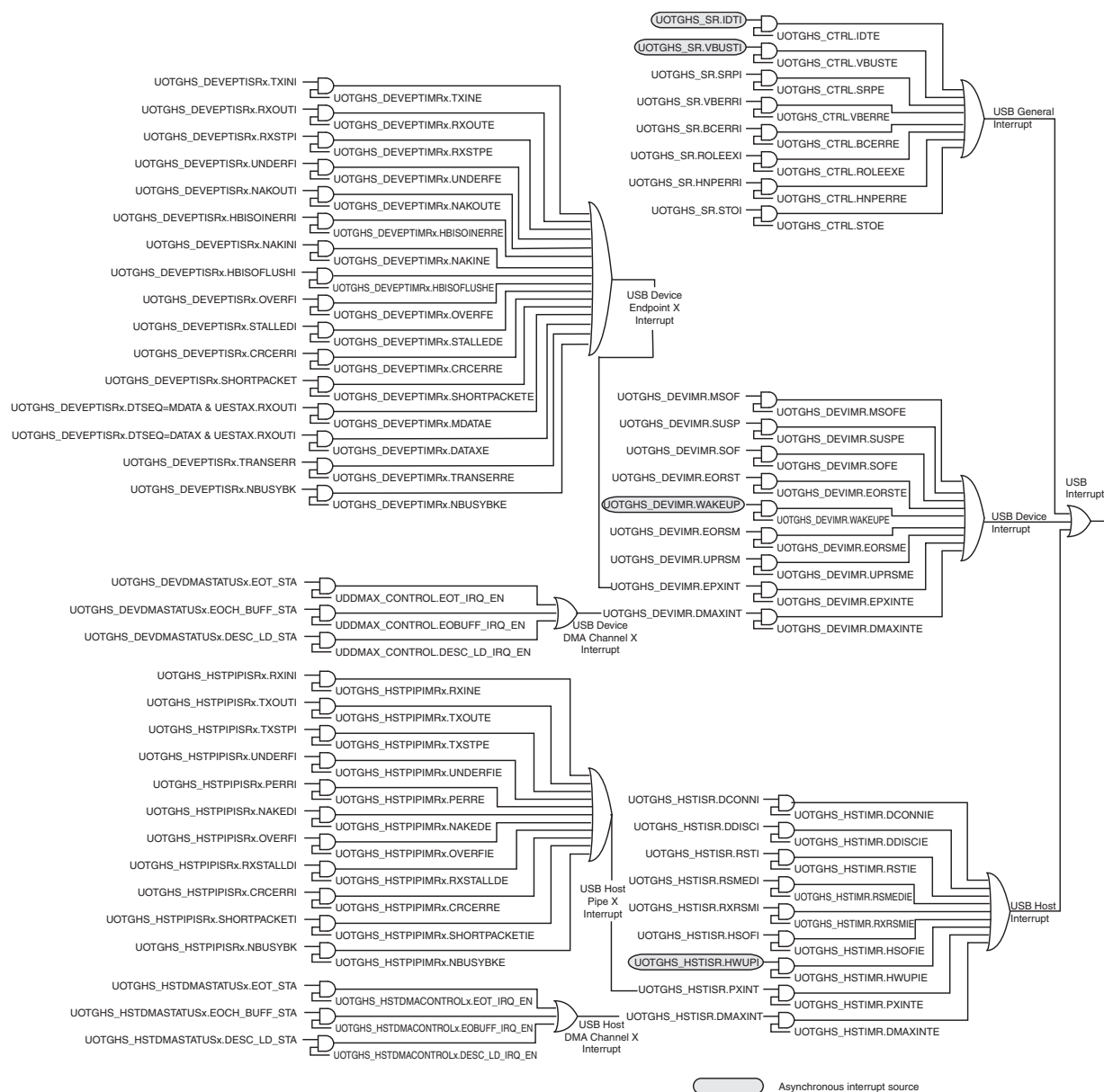
FIGURE 39-11: INTERRUPT SYSTEM
