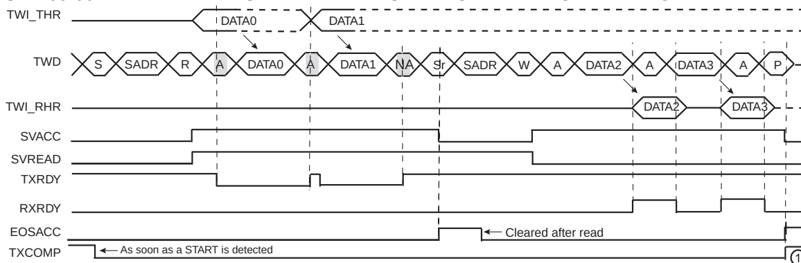
FIGURE 33-39: REPEATED START + REVERSAL FROM READ TO WRITE MODE
