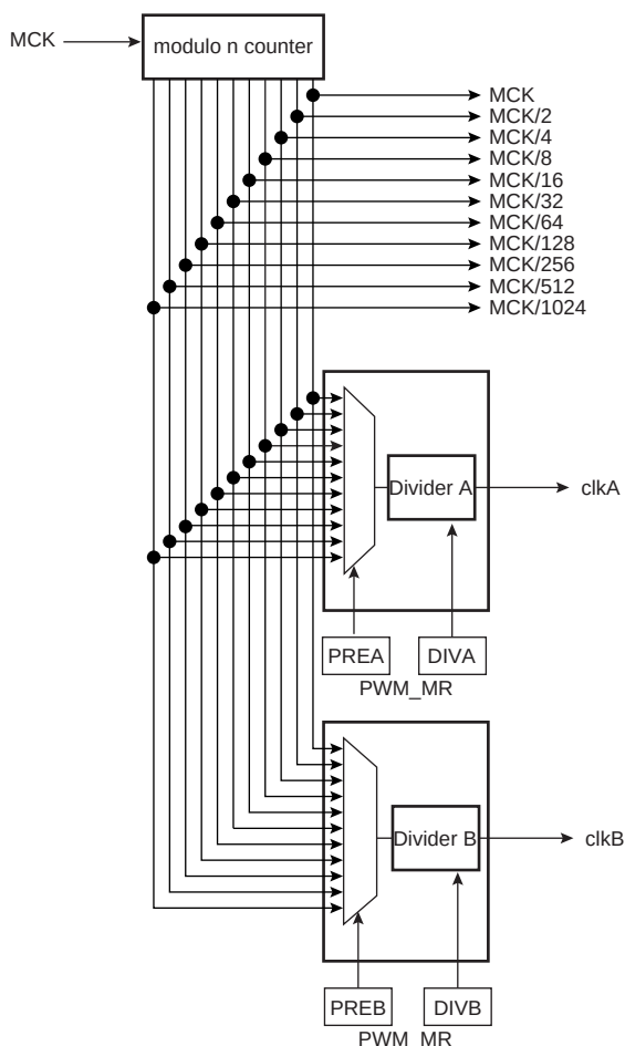
FIGURE 38-5: FUNCTIONAL VIEW OF THE CLOCK GENERATOR BLOCK DIAGRAM
