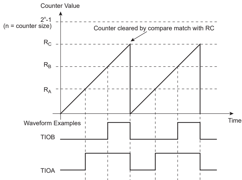
FIGURE 36-12: WAVSEL = 10 WITHOUT TRIGGER
