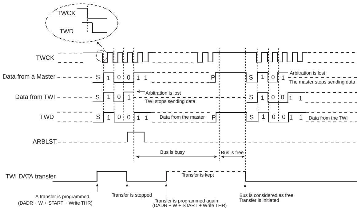
FIGURE 33-30: ARBITRATION CASES
