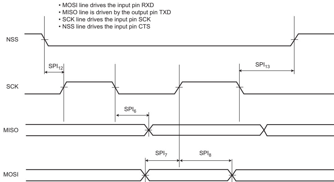
FIGURE 45-33: USART SPI SLAVE MODE (MODE 1 OR 2)
