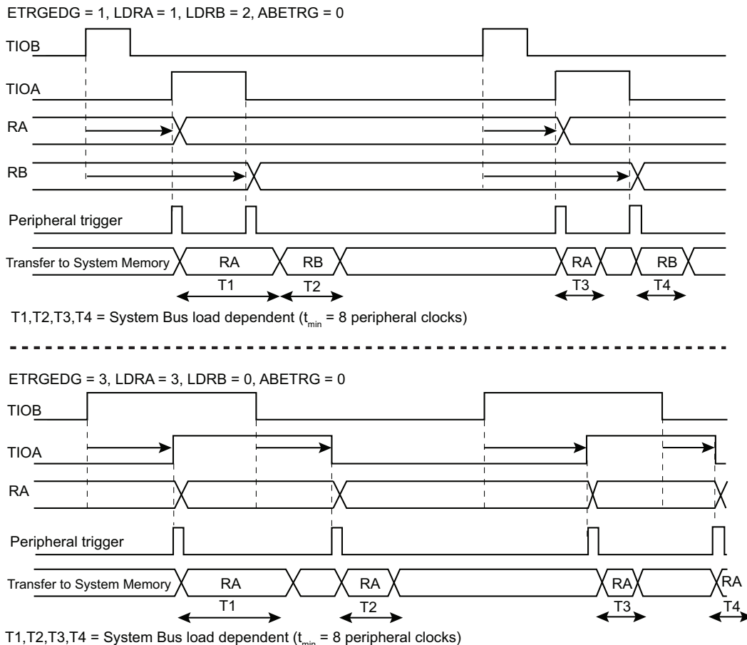
FIGURE 36-6: EXAMPLE OF TRANSFER WITH PDC
