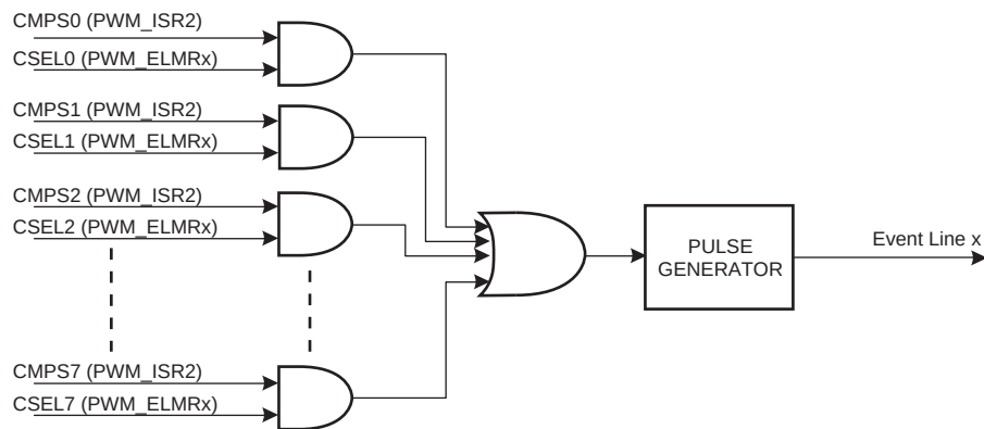
FIGURE 38-20: EVENT LINE BLOCK DIAGRAM
