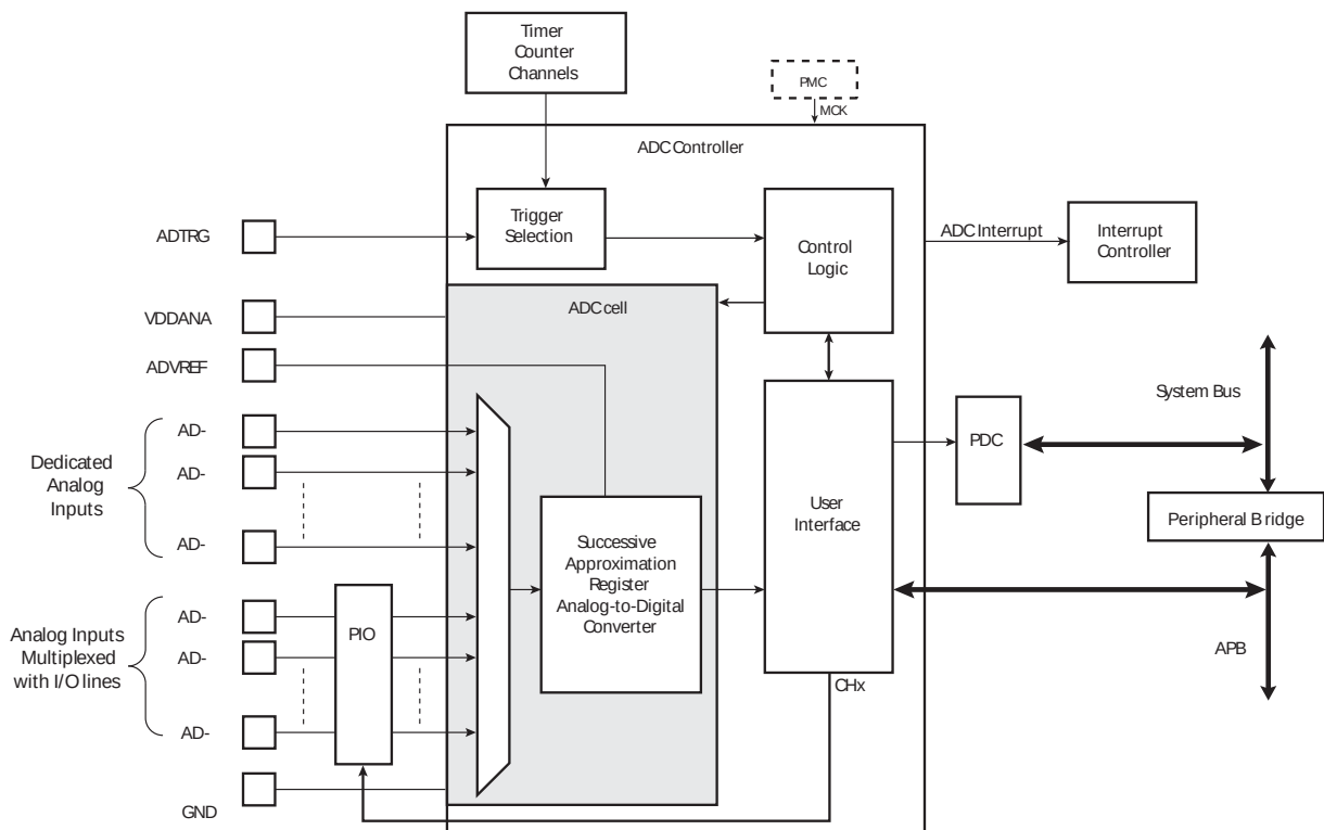
FIGURE 43-2: ANALOG-TO-DIGITAL CONVERTER BLOCK DIAGRAM
