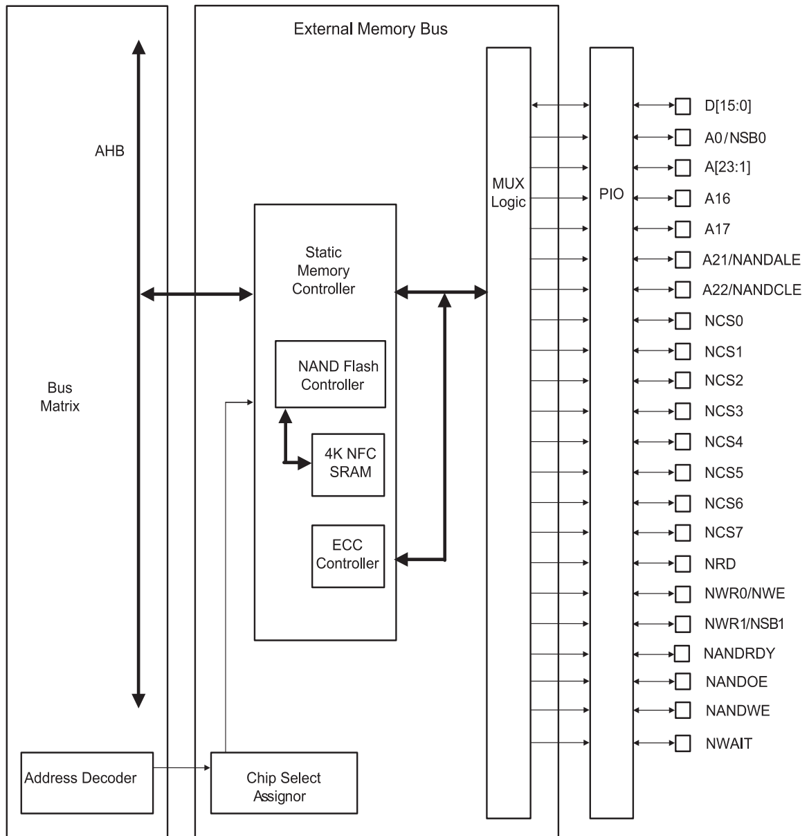
FIGURE 24-1: ORGANIZATION OF THE EXTERNAL BUS INTERFACE
