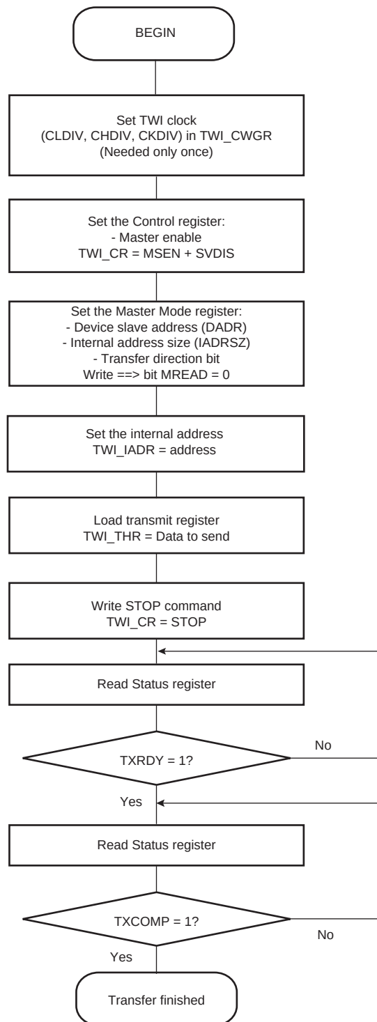
FIGURE 33-21: TWI WRITE OPERATION WITH SINGLE DATA BYTE AND INTERNAL ADDRESS
