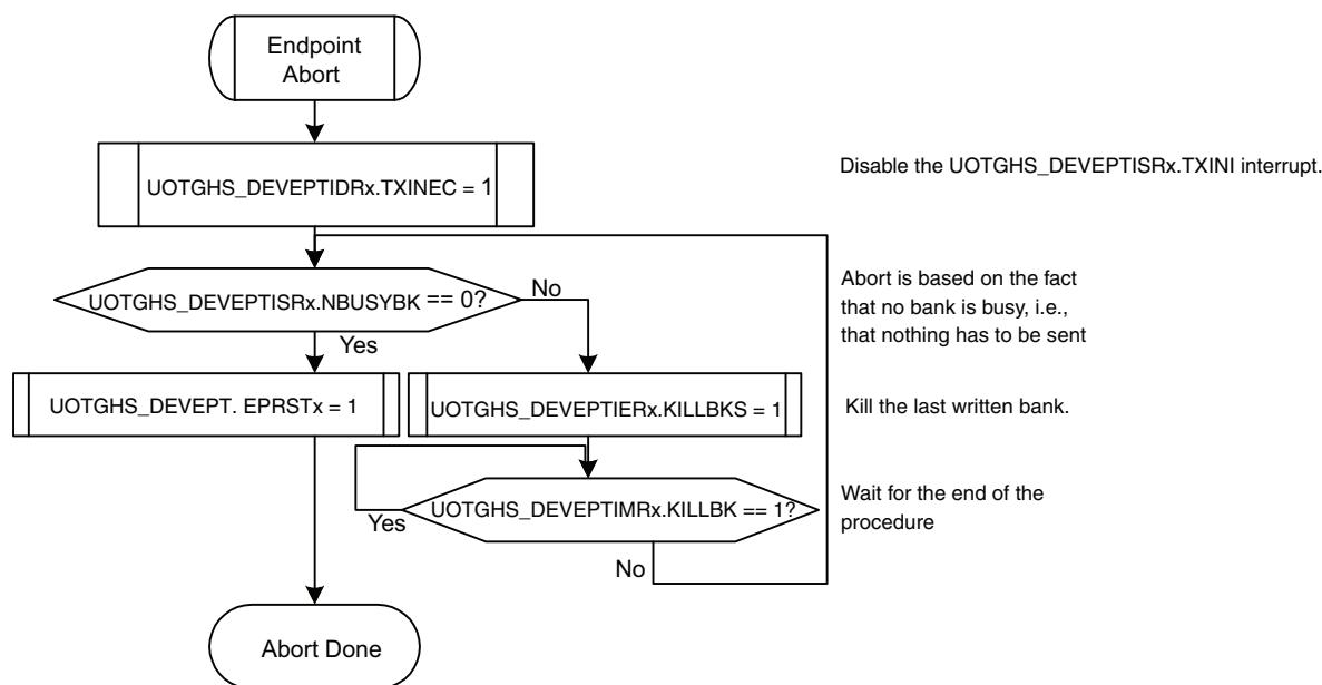
FIGURE 39-24: ABORT ALGORITHM
