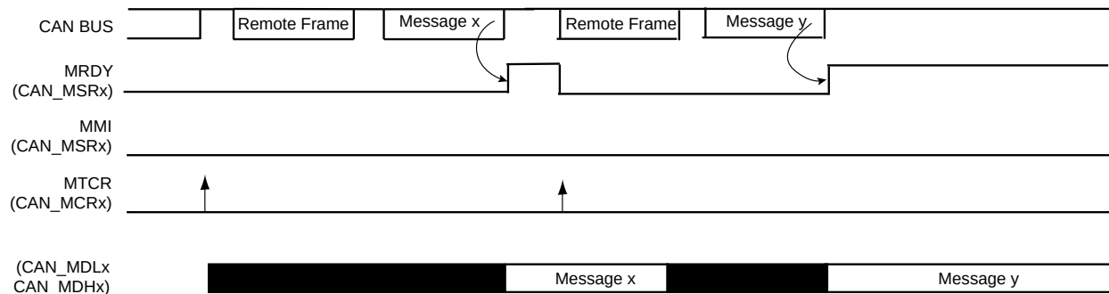
FIGURE 40-18: CONSUMER HANDLING
