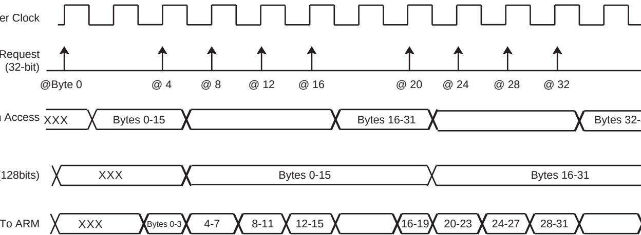
FIGURE 19-4: DATA READ OPTIMIZATION FOR FWS = 1
