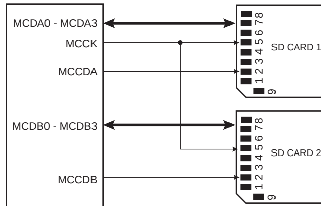
FIGURE 37-17: SD CARD BUS CONNECTIONS WITH TWO SLOTS
