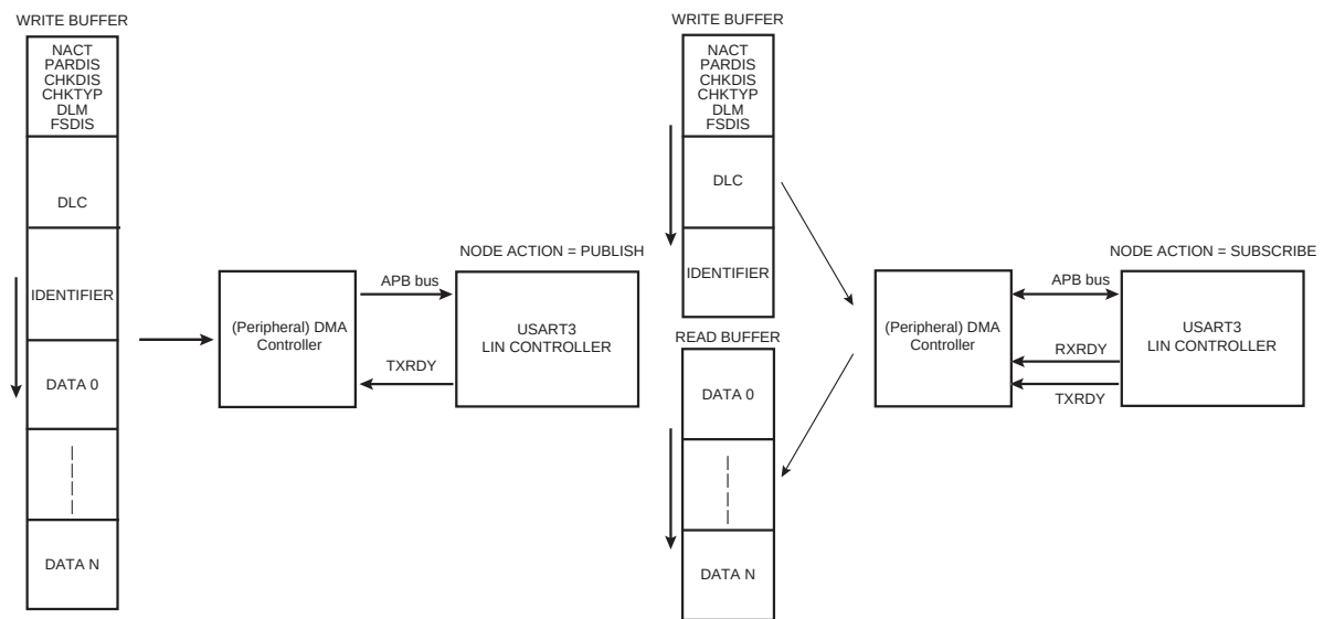
FIGURE 35-60: MASTER NODE WITH PDC (PDCM = 1)
