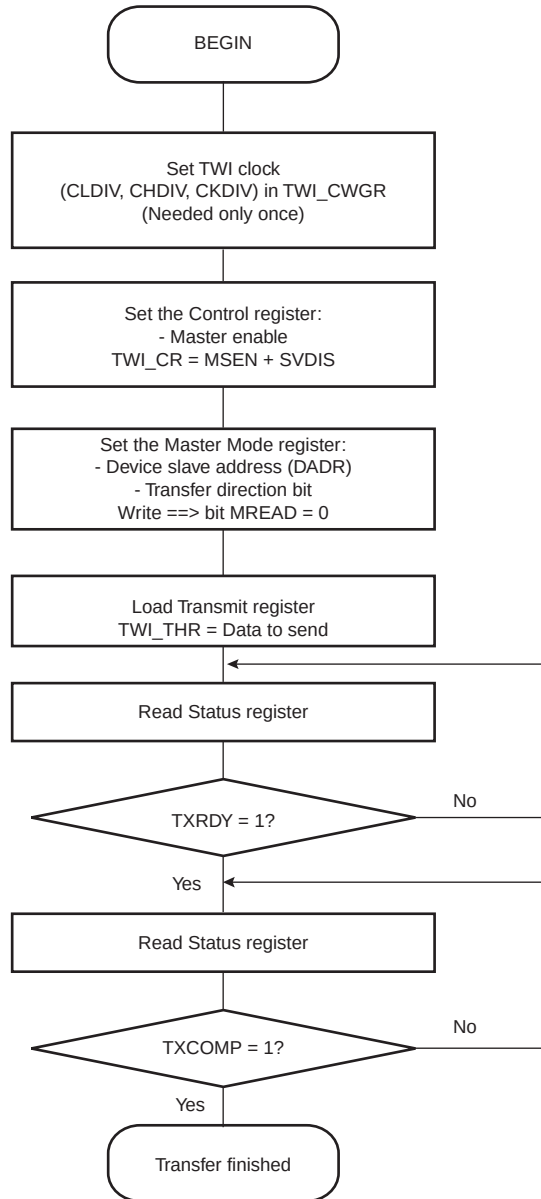
FIGURE 33-23: TWI WRITE OPERATION WITH SINGLE DATA BYTE WITHOUT INTERNAL ADDRESS
