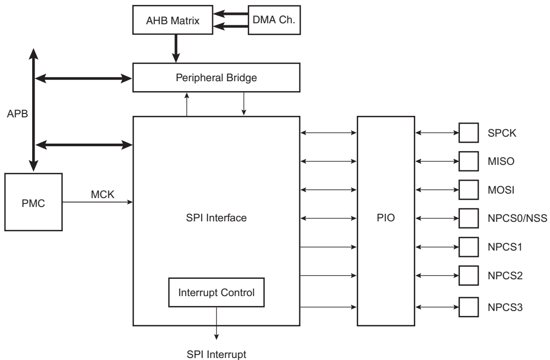
FIGURE 32-2: BLOCK DIAGRAM
