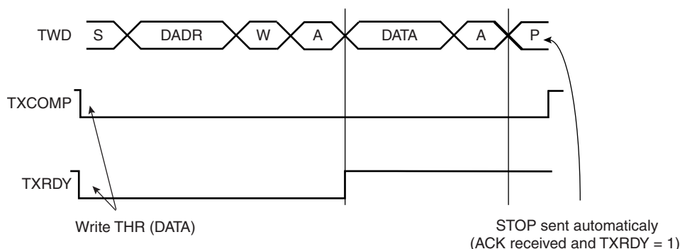
FIGURE 33-10: MASTER WRITE WITH ONE DATA BYTE
