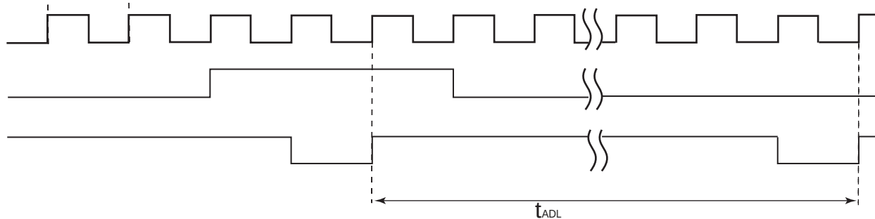
FIGURE 25-33: WRITE ENABLE TIMING FOR NAND FLASH DEVICE DATA INPUT MODE.
