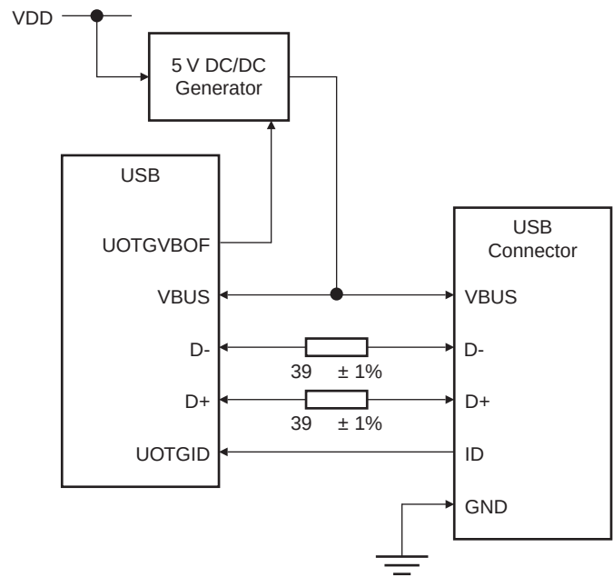
FIGURE 39-7: HOST AND OTG APPLICATION BLOCK DIAGRAM
