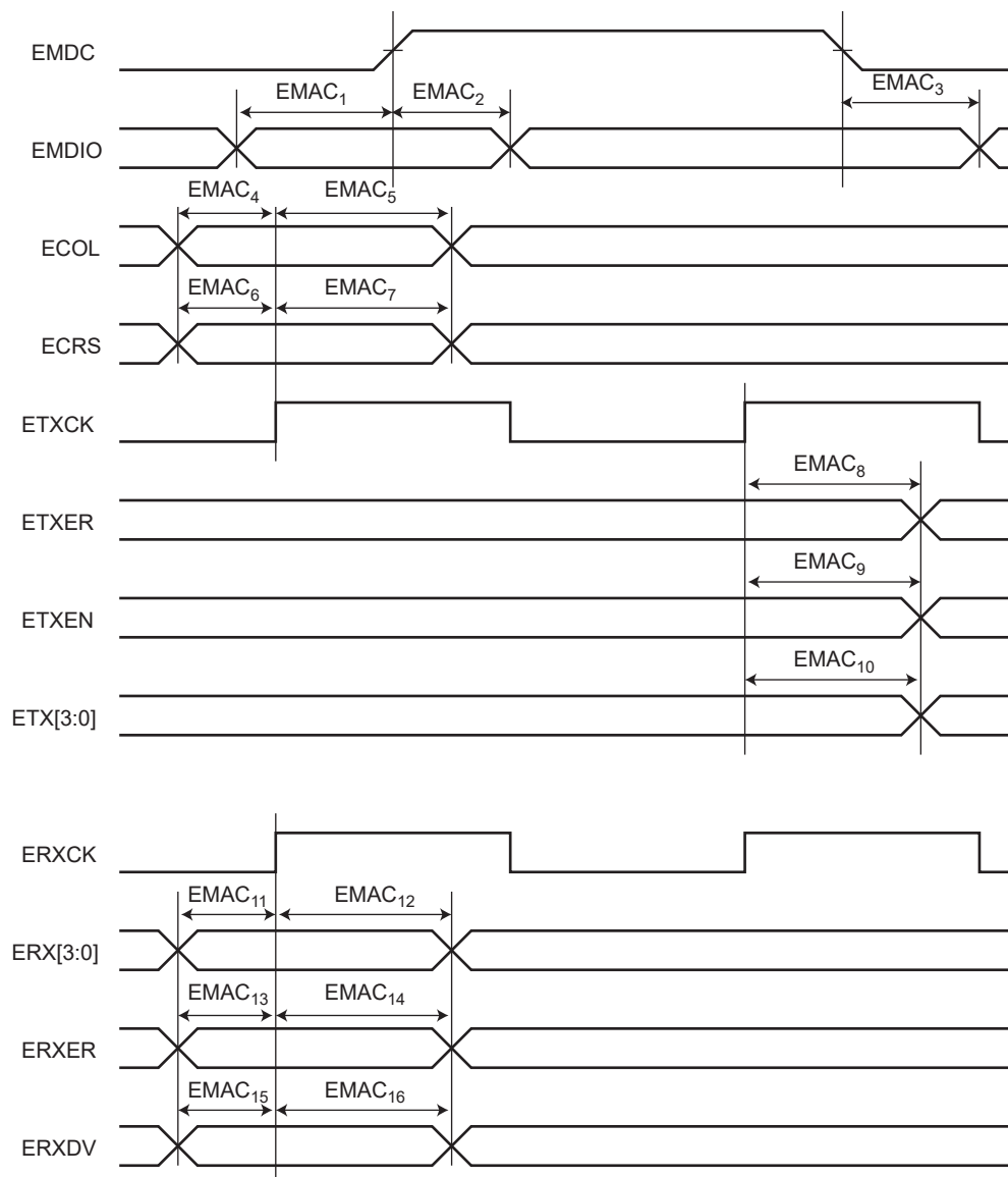
FIGURE 45-36: EMAC MII MODE
