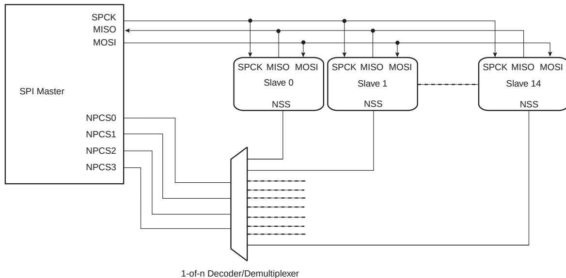
FIGURE 32-11: CHIP SELECT DECODING APPLICATION BLOCK DIAGRAM: SINGLE
