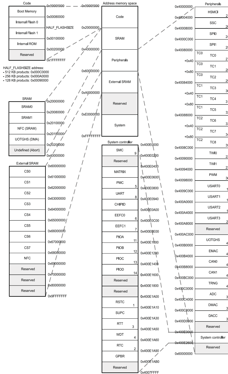
FIGURE 8-1: SAM3X8ERT PRODUCT MAPPING
