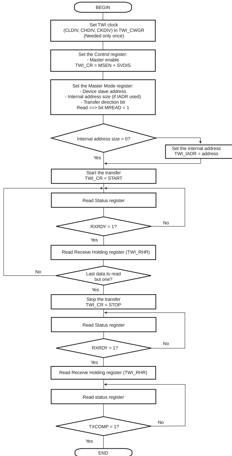
FIGURE 33-28: TWI READ OPERATION WITH MULTIPLE DATA BYTES WITH OR WITHOUT INTERNAL ADDRESS
