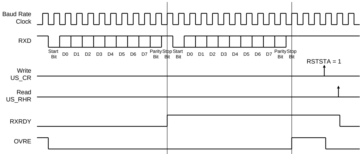
FIGURE 35-29: RECEIVER STATUS
