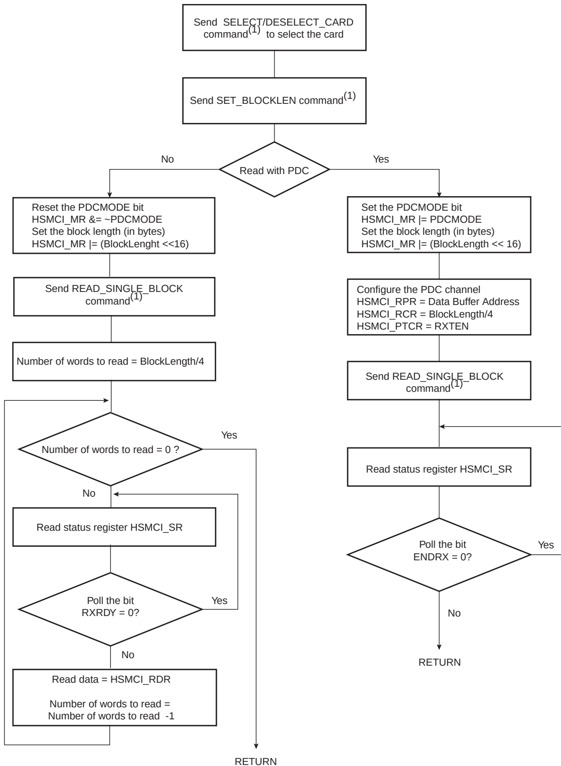
FIGURE 37-19: READ FUNCTIONAL FLOW DIAGRAM
