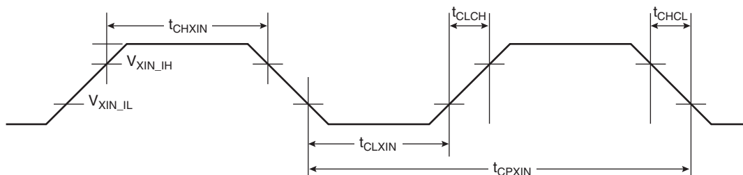
FIGURE 45-13: XIN CLOCK TIMING
