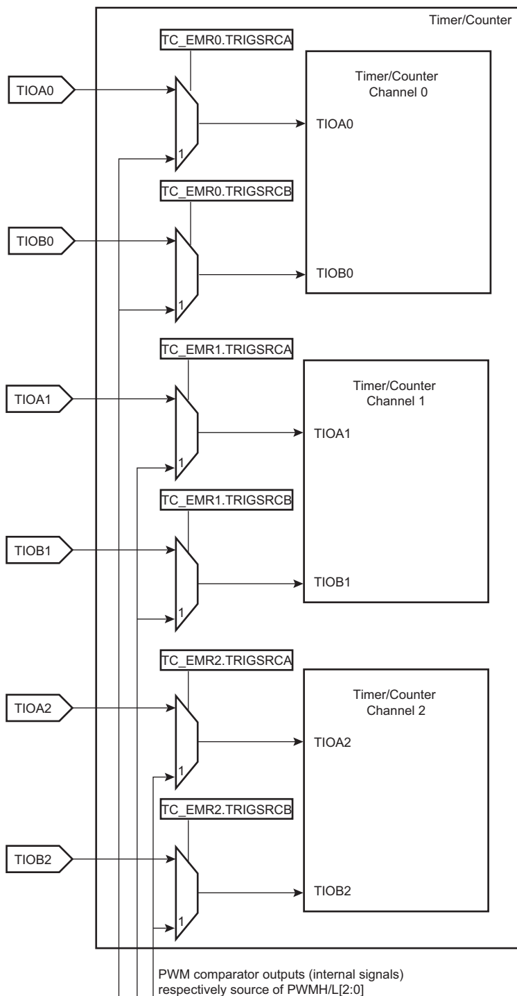
FIGURE 36-18: SYNCHRONIZATION WITH PWM
