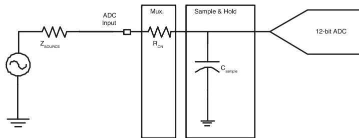
FIGURE 45-16: SIMPLIFIED ACQUISITION PATH
