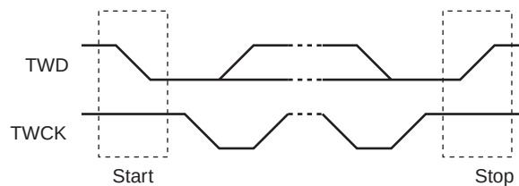
FIGURE 33-4: START AND STOP CONDITIONS
