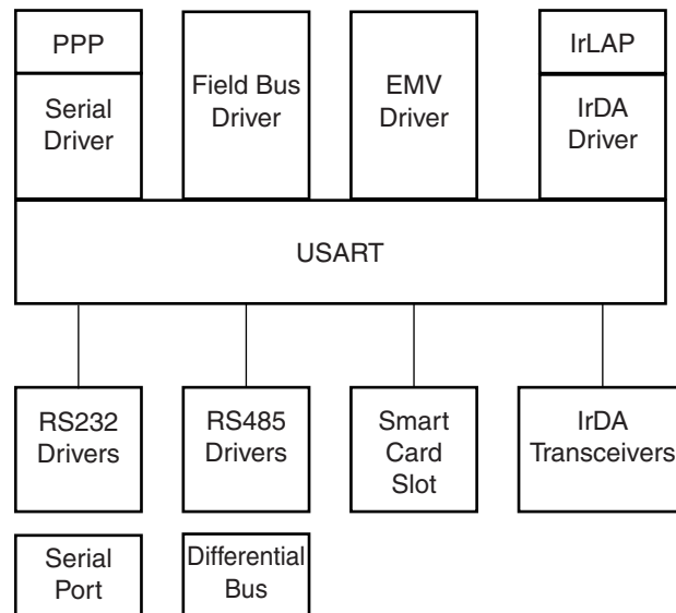
FIGURE 35-10: APPLICATION BLOCK DIAGRAM
