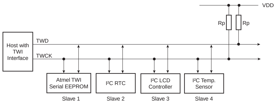
FIGURE 33-6: MASTER MODE TYPICAL APPLICATION BLOCK DIAGRAM
