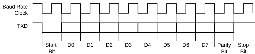
FIGURE 35-14: CHARACTER TRANSMIT
