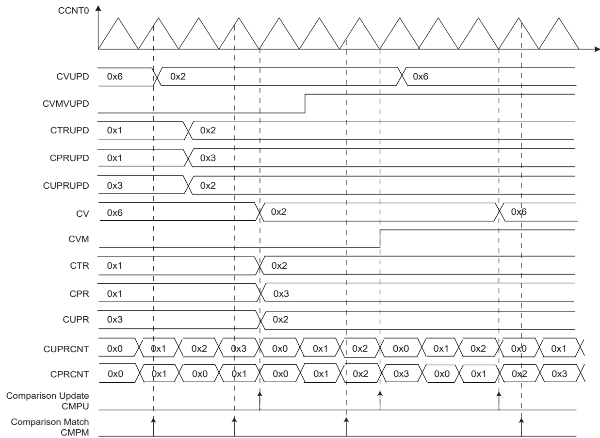
FIGURE 38-19: COMPARISON WAVEFORM
