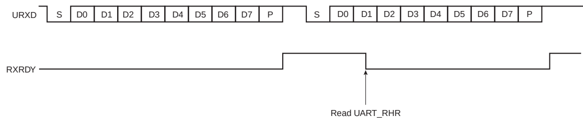
FIGURE 34-6: RECEIVER READY
