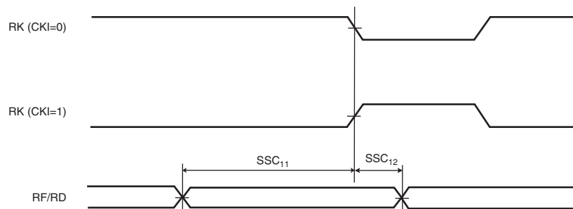
FIGURE 45-28: SSC RECEIVER, RK AS OUTPUT AND RF AS INPUT
