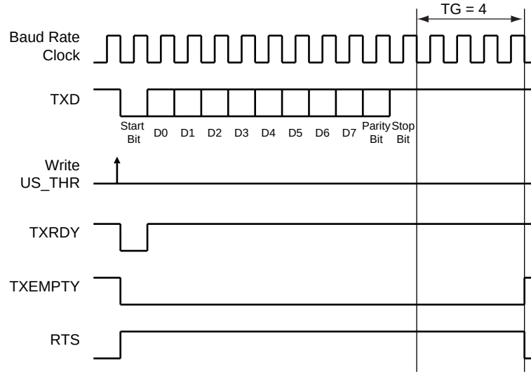
FIGURE 35-45: EXAMPLE OF RTS DRIVE WITH TIMEGUARD
