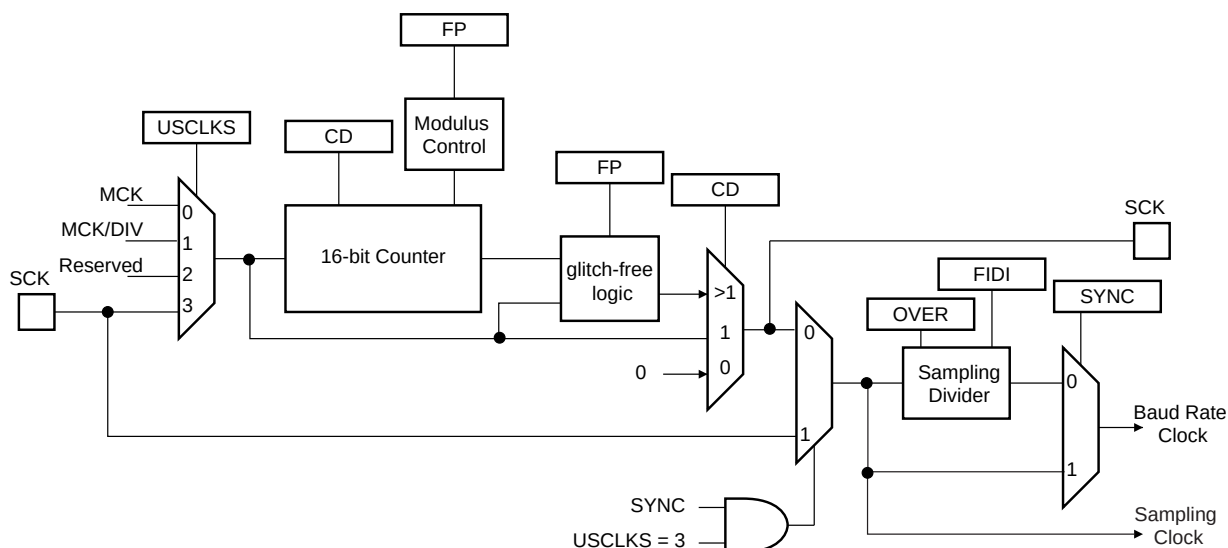
FIGURE 35-12: FRACTIONAL BAUD RATE GENERATOR
