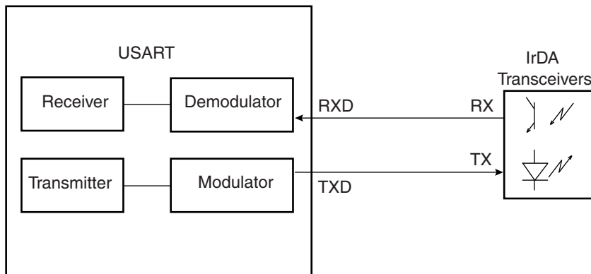
FIGURE 35-41: CONNECTION TO IRDA TRANSCEIVERS
