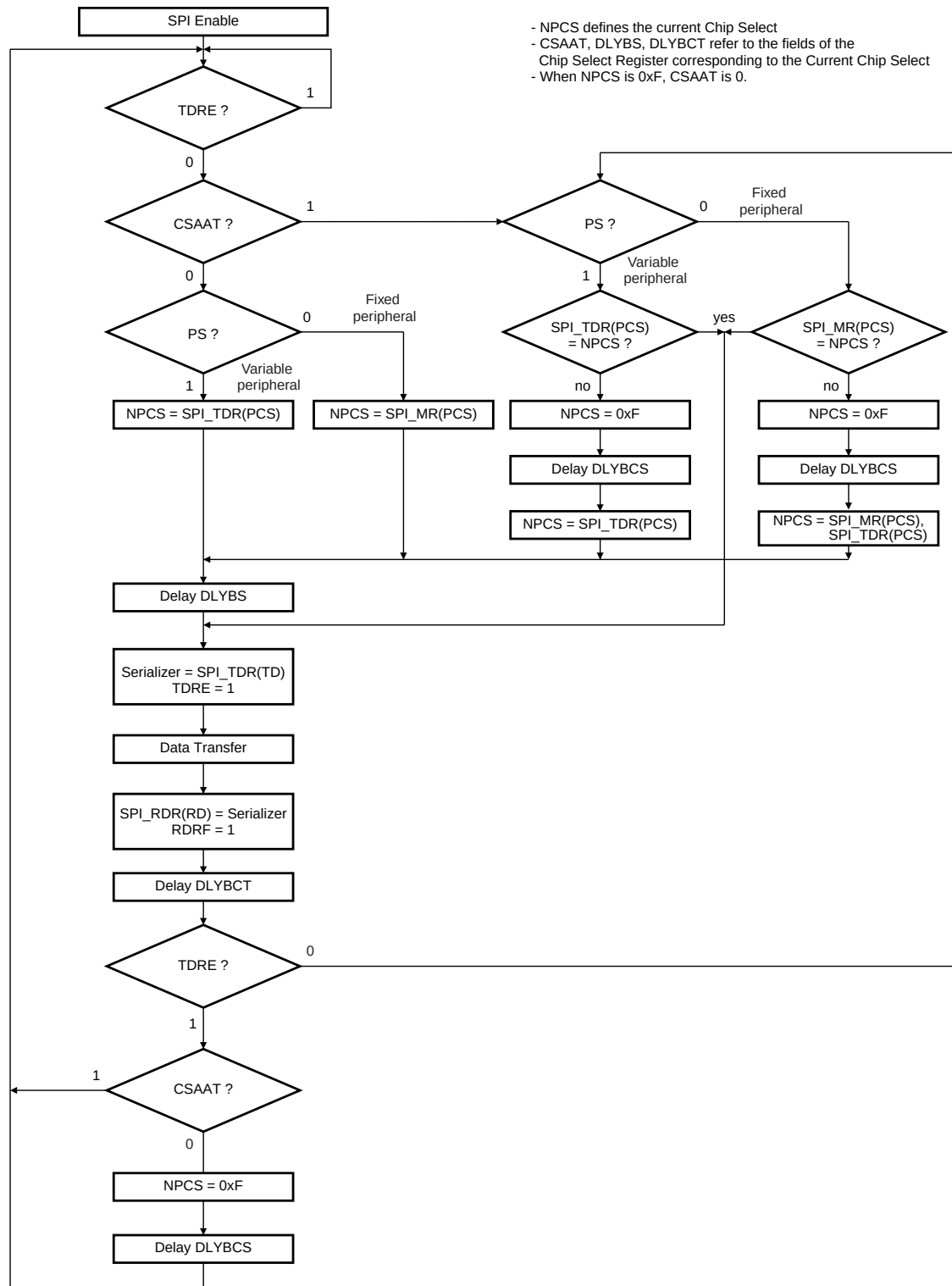
FIGURE 32-7: MASTER MODE FLOW DIAGRAM
