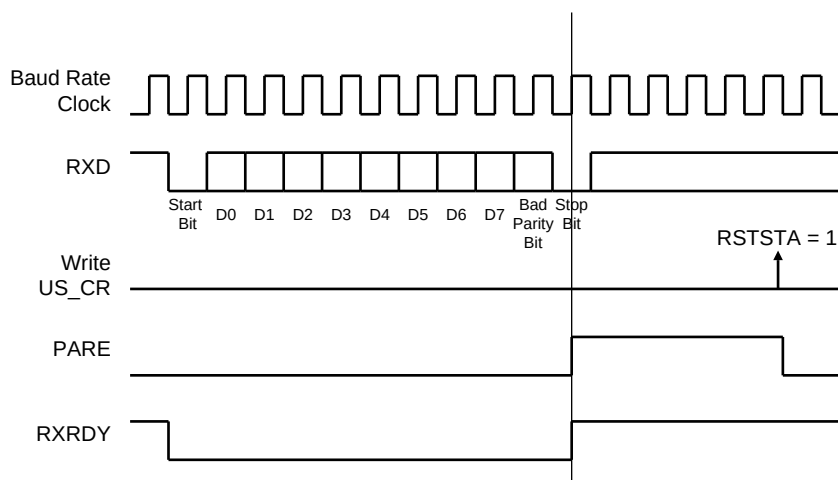
FIGURE 35-30: PARITY ERROR
