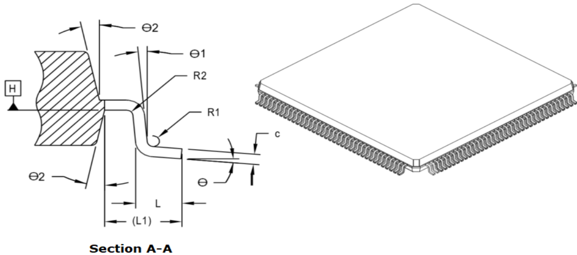
FIGURE 46-2: 144-LEAD PLASTIC QUAD FLATPACK (2SB) - DIMENSION LIMIT
