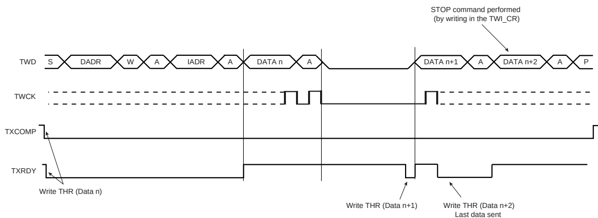
FIGURE 33-9: MASTER WRITE WITH ONE BYTE INTERNAL ADDRESS AND MULTIPLE DATA BYTES
