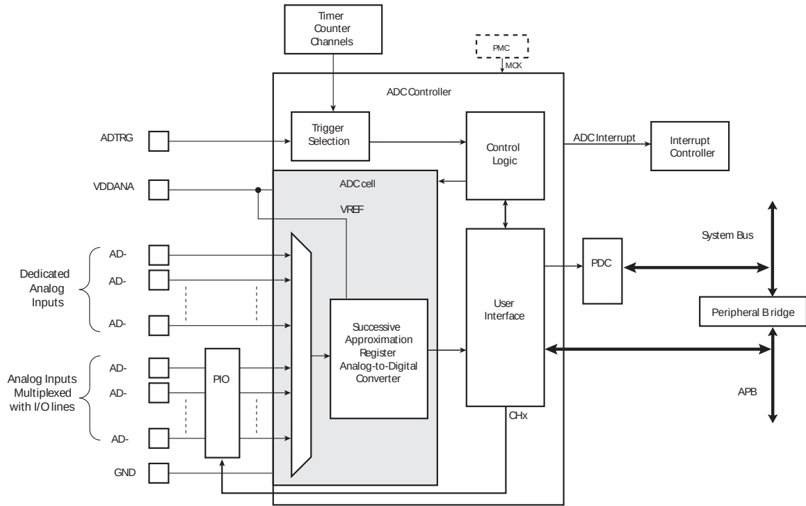
FIGURE 43-3: ANALOG-TO-DIGITAL CONVERTER BLOCK DIAGRAM
