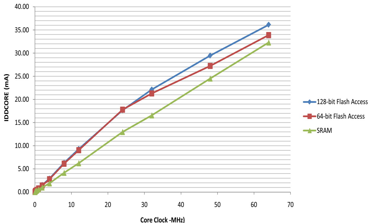
FIGURE 45-9: ACTIVE POWER CONSUMPTION WITH VDDCORE @ 1.8V RUNNING FROM FLASH MEMORY OR SRAM
