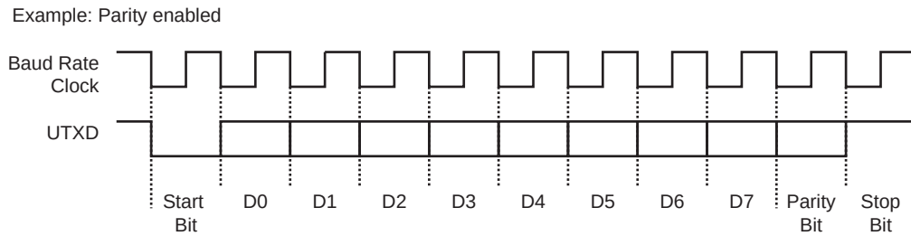
FIGURE 34-10: CHARACTER TRANSMISSION
