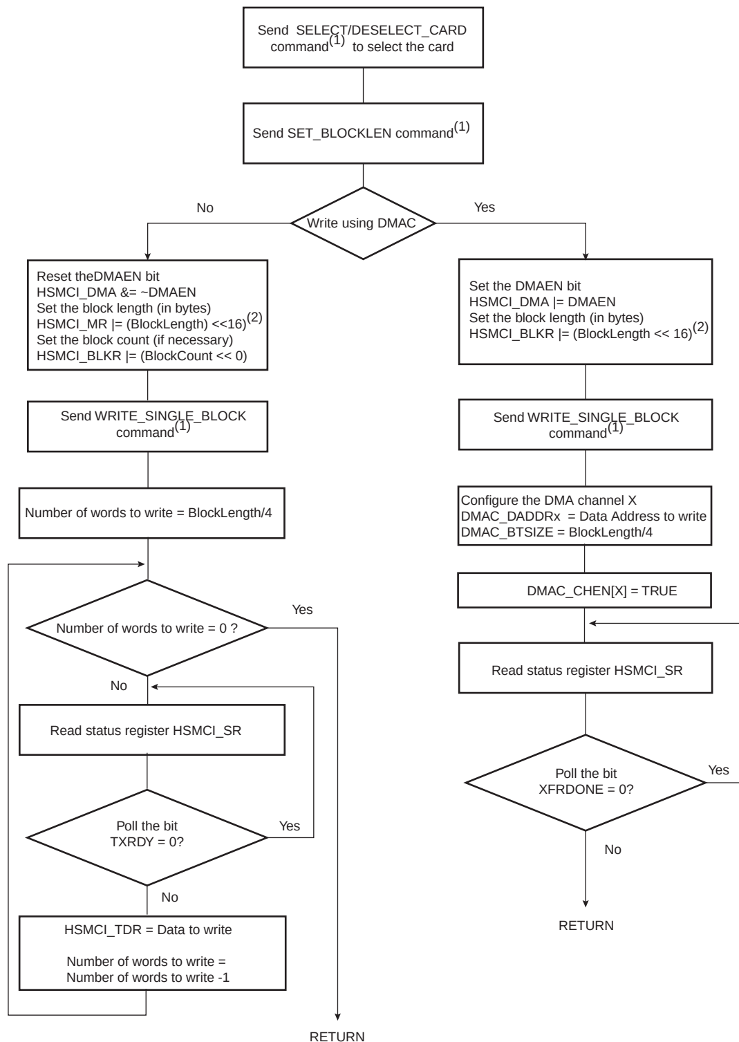
FIGURE 37-23: WRITE FUNCTIONAL FLOW DIAGRAM
