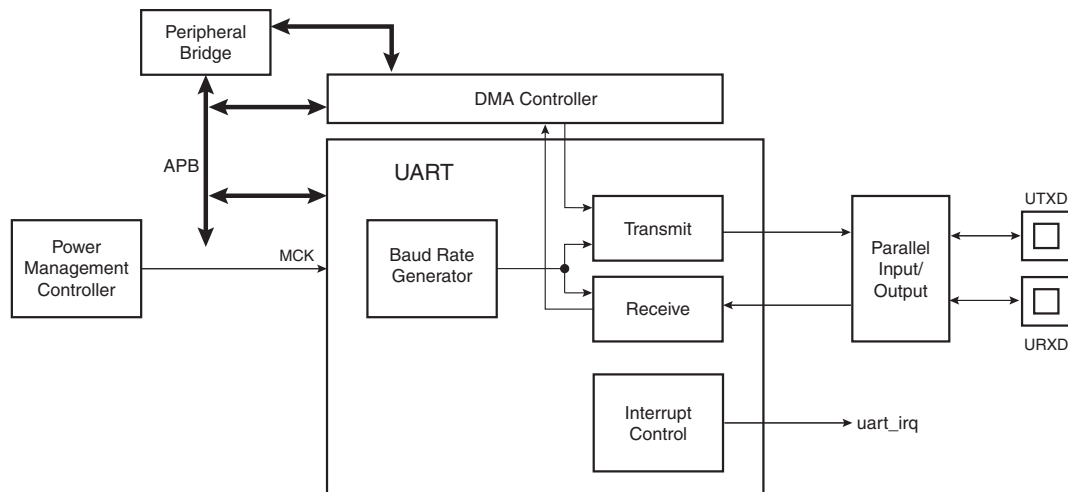
FIGURE 34-1: UART FUNCTIONAL BLOCK DIAGRAM
