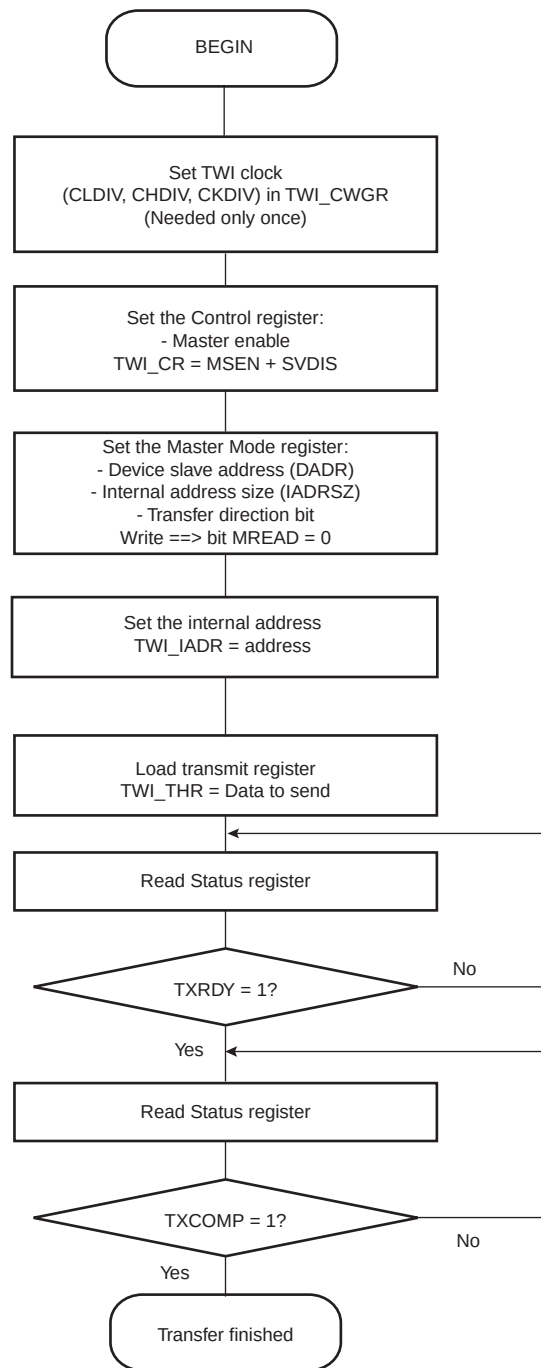
FIGURE 33-24: TWI WRITE OPERATION WITH SINGLE DATA BYTE AND INTERNAL ADDRESS
