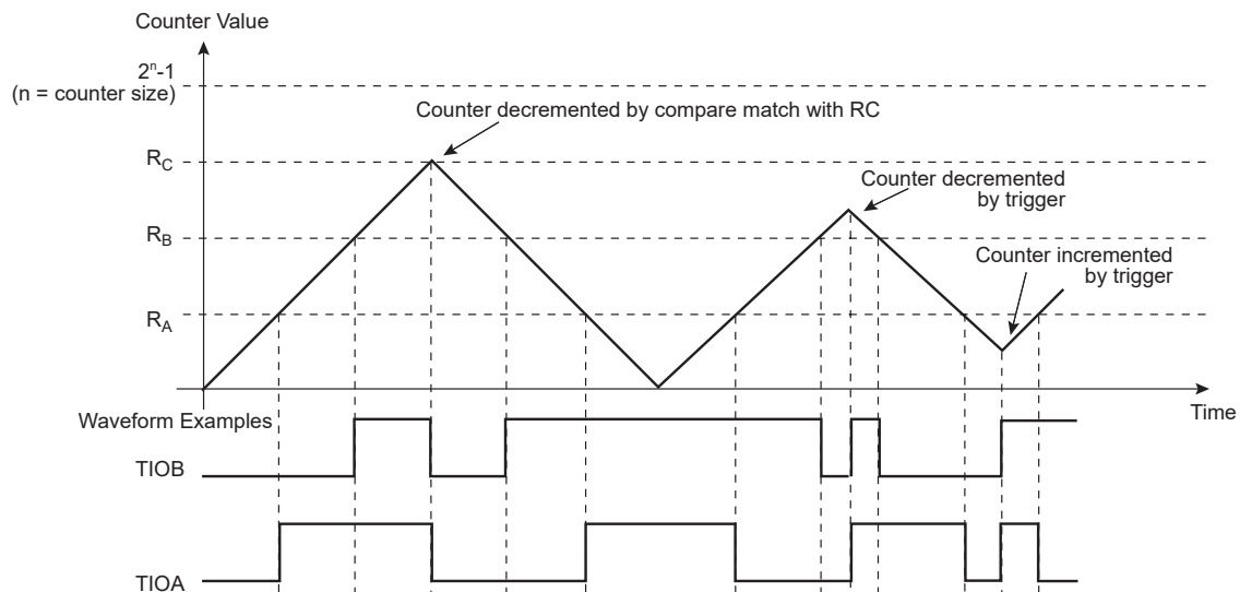
FIGURE 36-17: WAVSEL = 11 WITH TRIGGER
