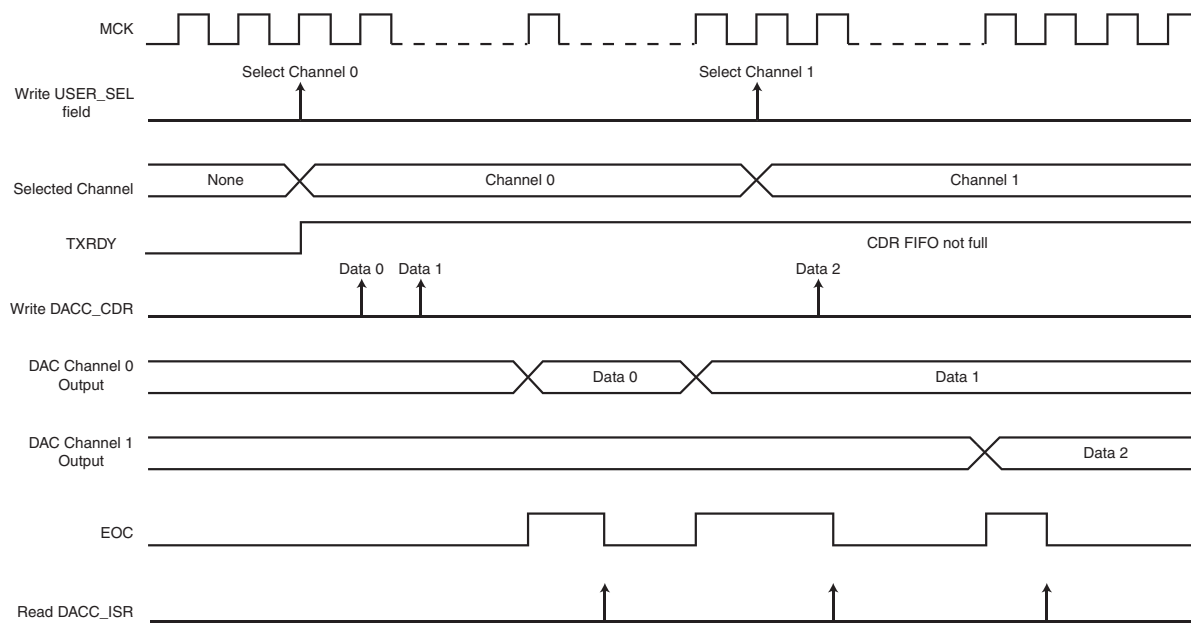
FIGURE 44-3: CONVERSION SEQUENCE
