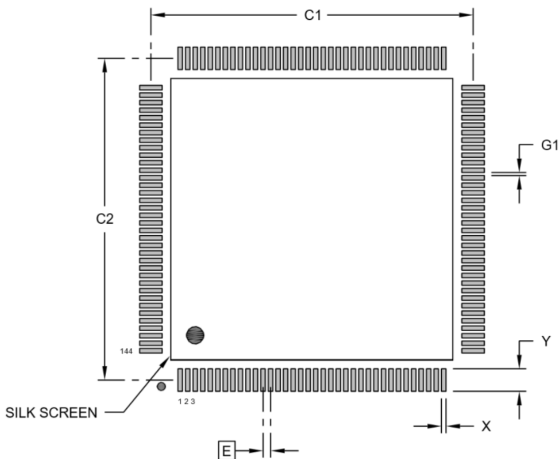
FIGURE 46-3: 144-LEAD PLASTIC QUAD FLATPACK (2SB) - SILK SCREEN
