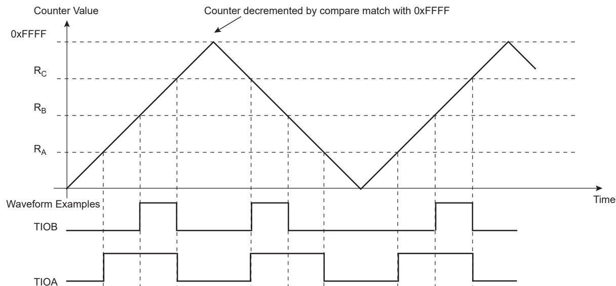
FIGURE 36-14: WAVSEL = 01 WITHOUT TRIGGER
