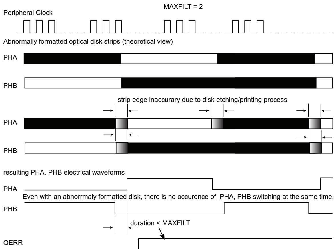
FIGURE 36-23: QUADRATURE ERROR DETECTION
