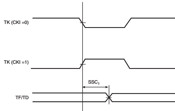
FIGURE 45-22: SSC TRANSMITTER, TK AS INPUT AND TF AS OUTPUT
