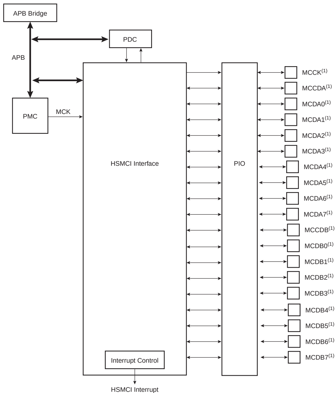
FIGURE 37-7: BLOCK DIAGRAM
