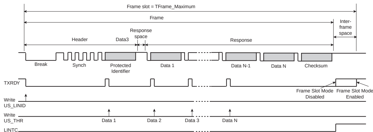
FIGURE 35-53: FRAME SLOT MODE
