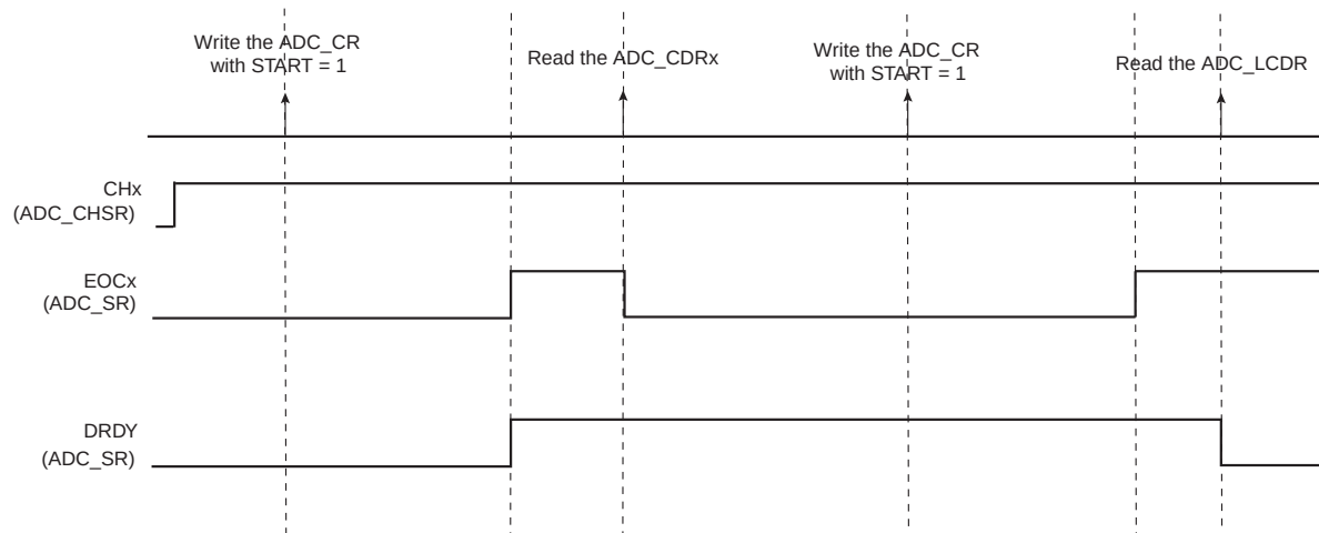
FIGURE 43-11: EOCX AND DRDY FLAG BEHAVIOR
