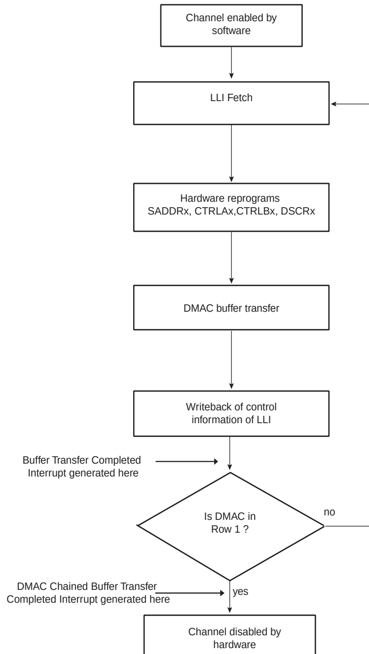
FIGURE 23-9: DMAC TRANSFER FLOW FOR LINKED LIST SOURCE ADDRESS AND CONTIGUOUS DESTINATION ADDRESS
