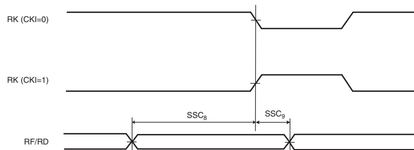
FIGURE 45-25: SSC RECEIVER RK AND RF AS INPUT
