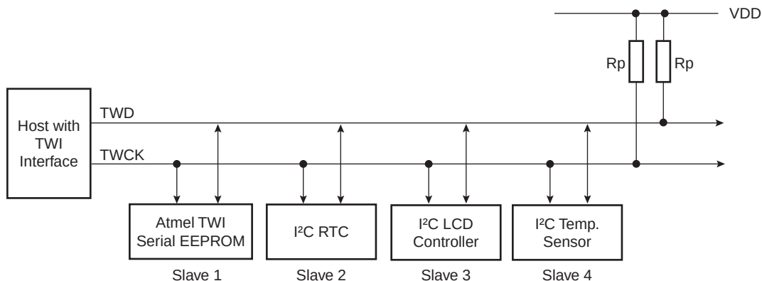
FIGURE 33-3: APPLICATION BLOCK DIAGRAM
