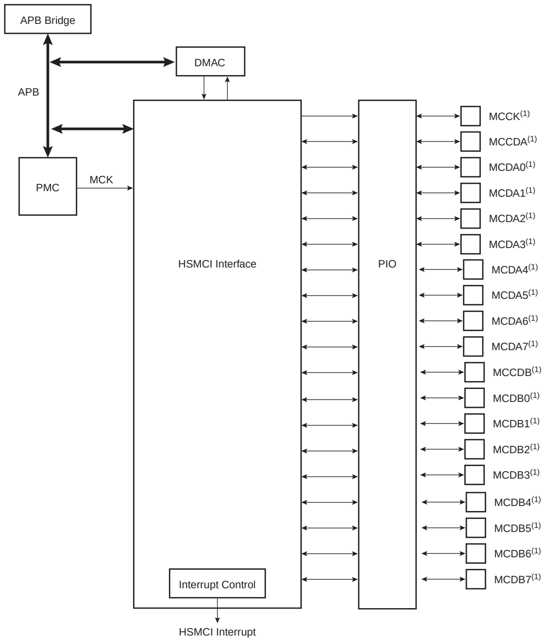
FIGURE 37-5: BLOCK DIAGRAM
