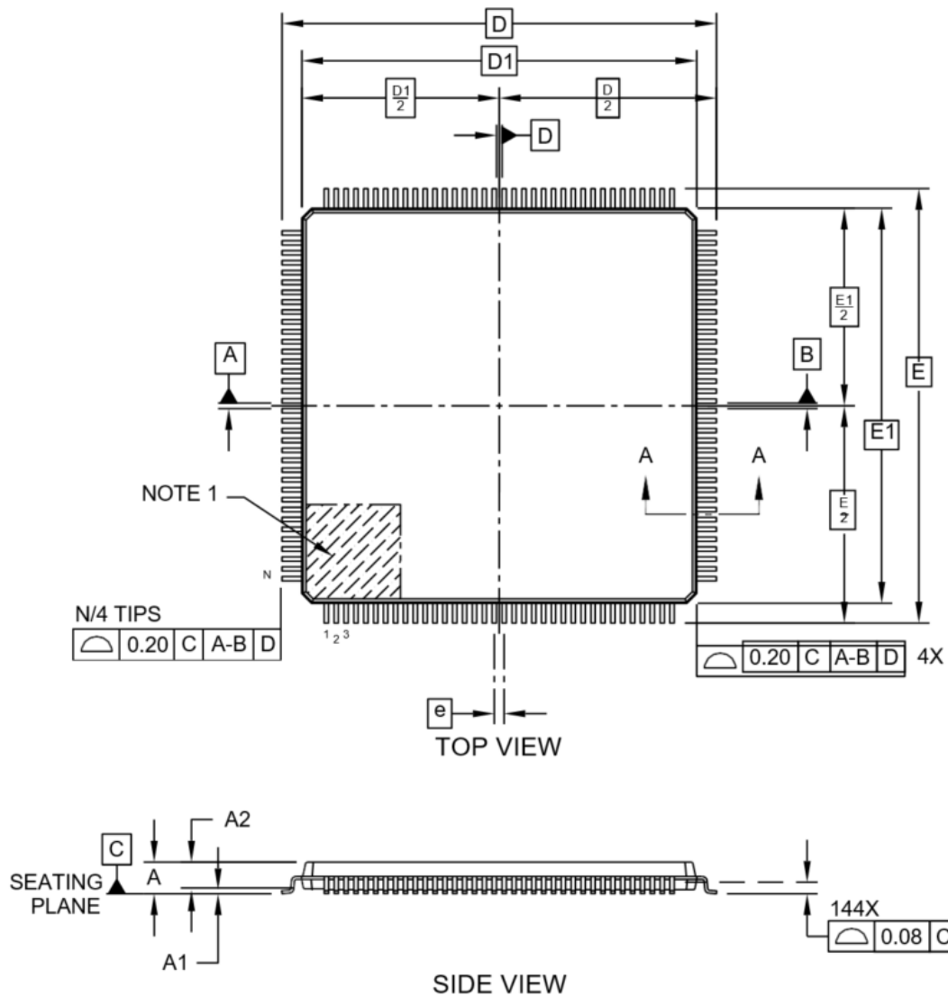
FIGURE 46-1: 144-LEAD LQFP PACKAGE DRAWING-TOP- SIDE-VIEW
