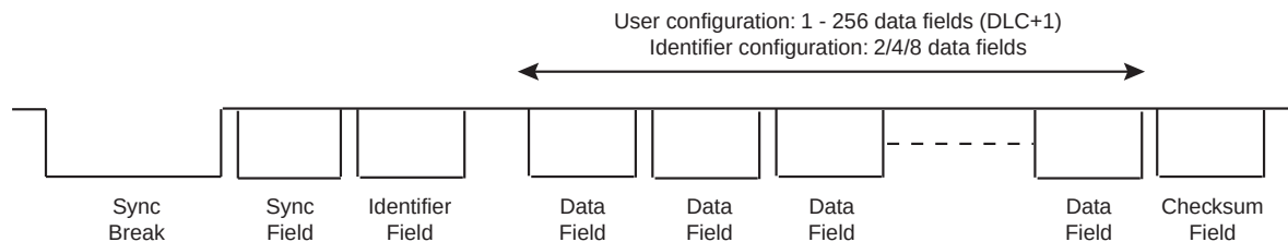
FIGURE 35-52: RESPONSE DATA LENGTH
