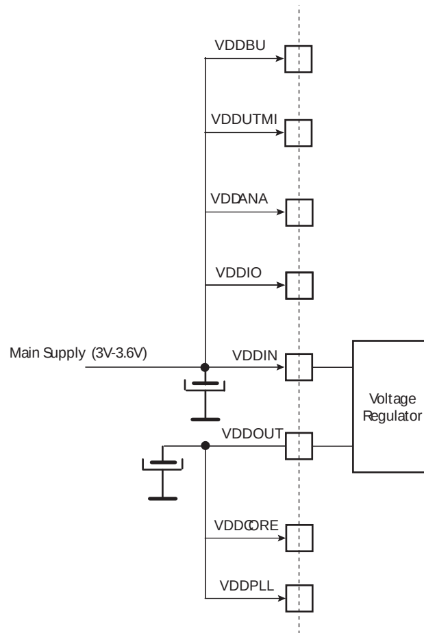
FIGURE 17-3: NO SEPARATED BACKUP SUPPLY POWERING SCHEME
