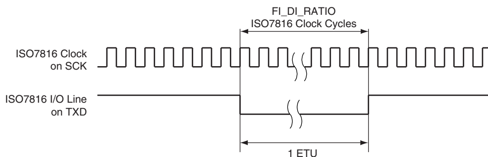
FIGURE 35-13: ELEMENTARY TIME UNIT (ETU)
