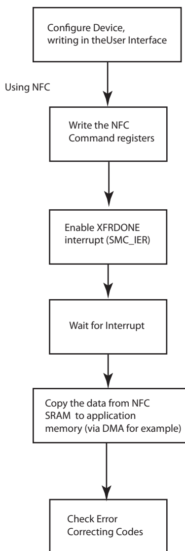
FIGURE 25-37: PAGE READ FLOW CHART
