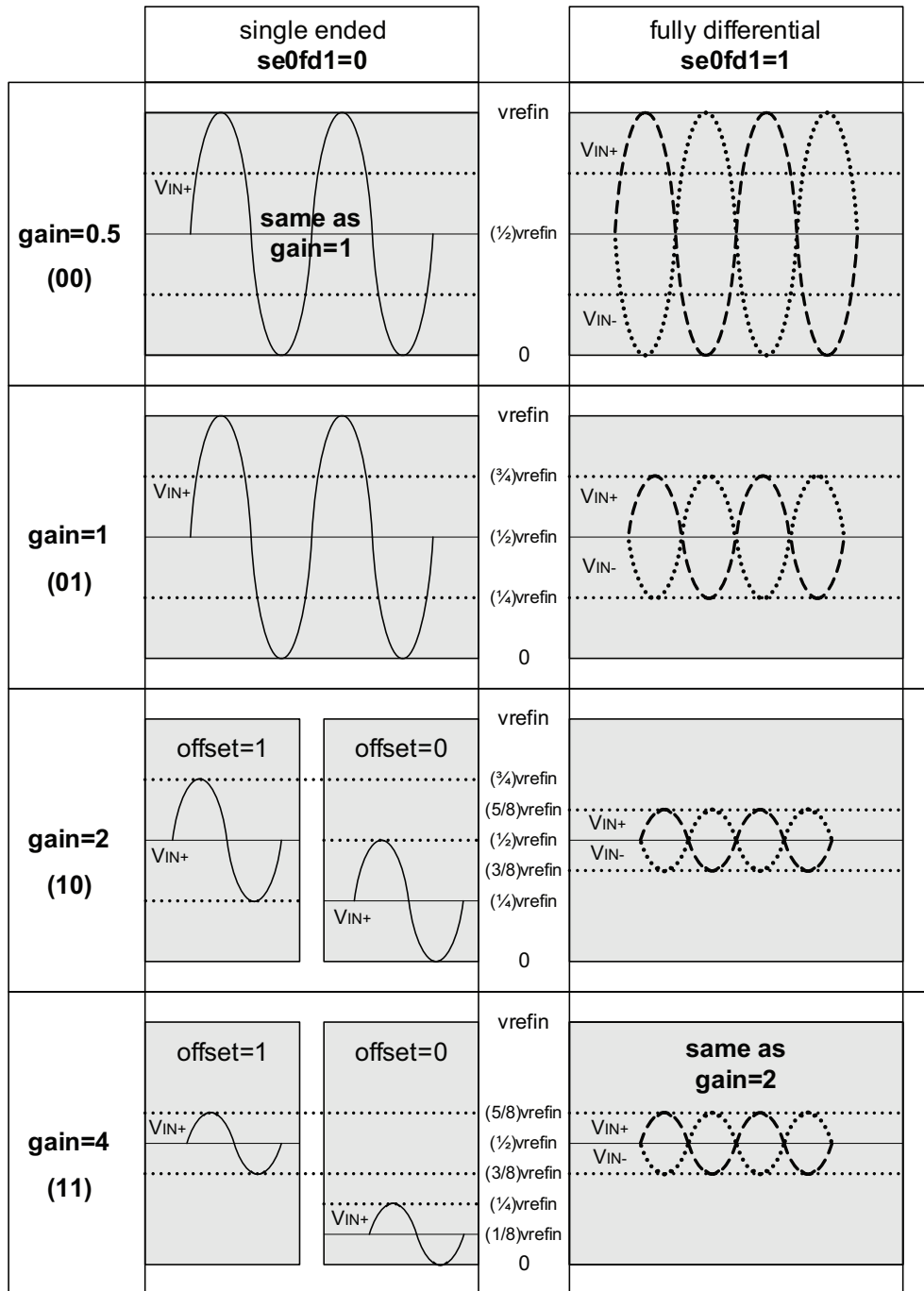
FIGURE 43-13: ANALOG FULL SCALE RANGES IN SINGLE ENDED/DIFFERENTIAL APPLICATIONS VERSUS GAIN AND OFFSET
