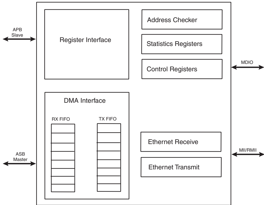
FIGURE 41-2: EMAC BLOCK DIAGRAM
