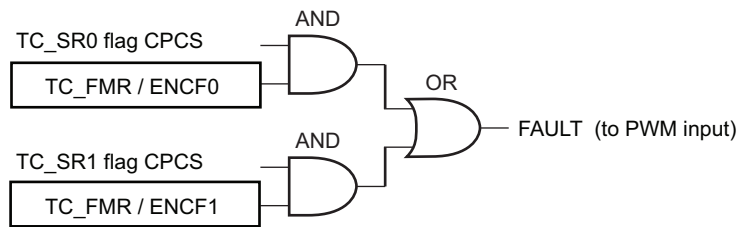
FIGURE 36-26: FAULT OUTPUT GENERATION
