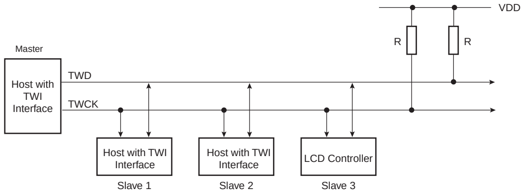
FIGURE 33-33: SLAVE MODE TYPICAL APPLICATION BLOCK DIAGRAM
