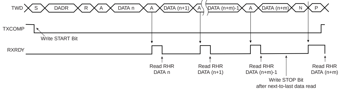
FIGURE 33-14: MASTER READ WITH MULTIPLE DATA BYTES
