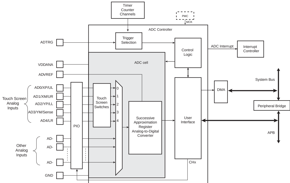
FIGURE 43-5: ANALOG-TO-DIGITAL CONVERTER BLOCK DIAGRAM WITH TOUCHSCREEN MODE
