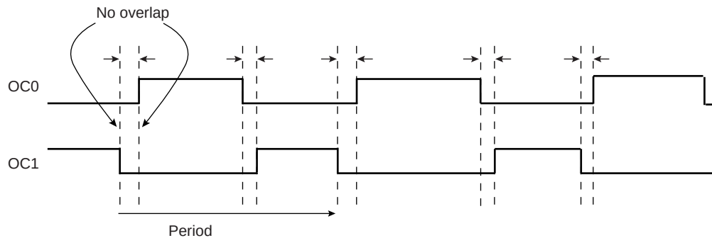
FIGURE 38-8: NON OVERLAPPED CENTER ALIGNED WAVEFORMS
