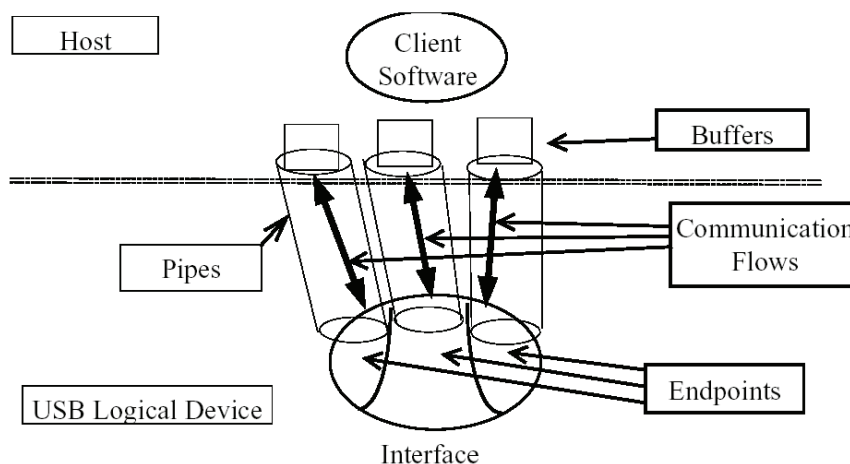
FIGURE 39-27: USB COMMUNICATION FLOW
