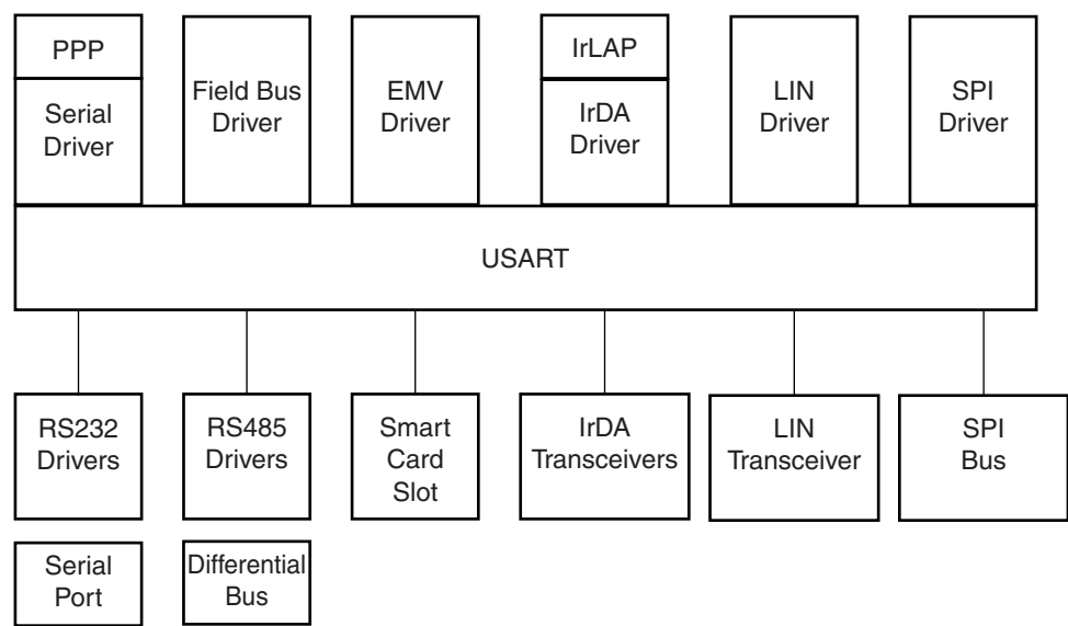
FIGURE 35-8: APPLICATION BLOCK DIAGRAM
