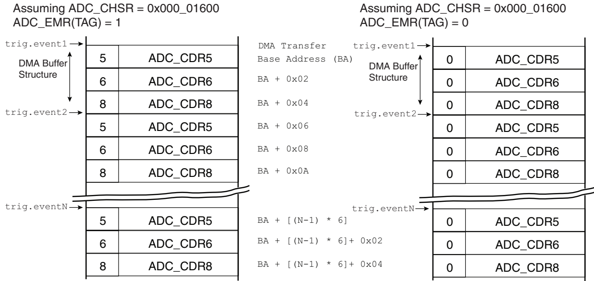
FIGURE 43-14: BUFFER STRUCTURE WHEN TSMODE = 0
