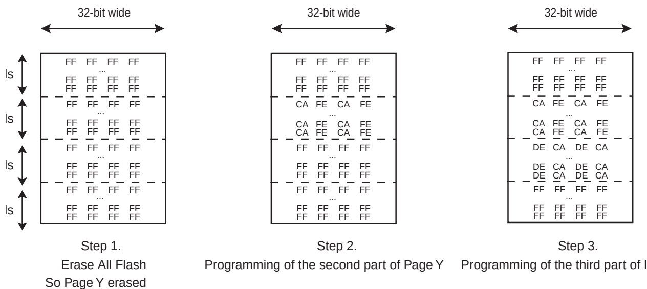
FIGURE 19-6: EXAMPLE OF PARTIAL PAGE PROGRAMMING
