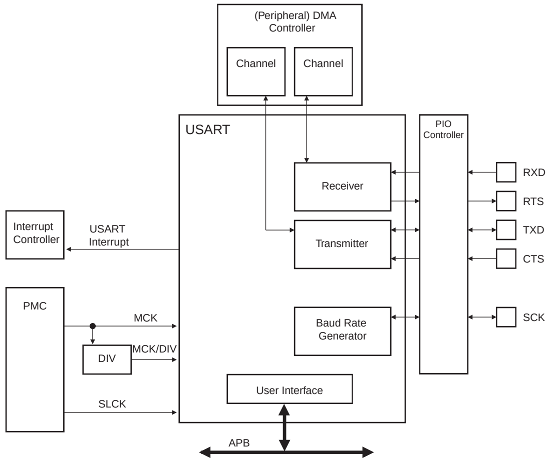
FIGURE 35-2: USART BLOCK DIAGRAM
