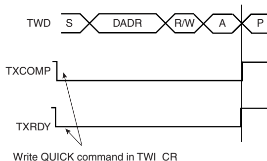
FIGURE 33-19: SMBUS QUICK COMMAND
