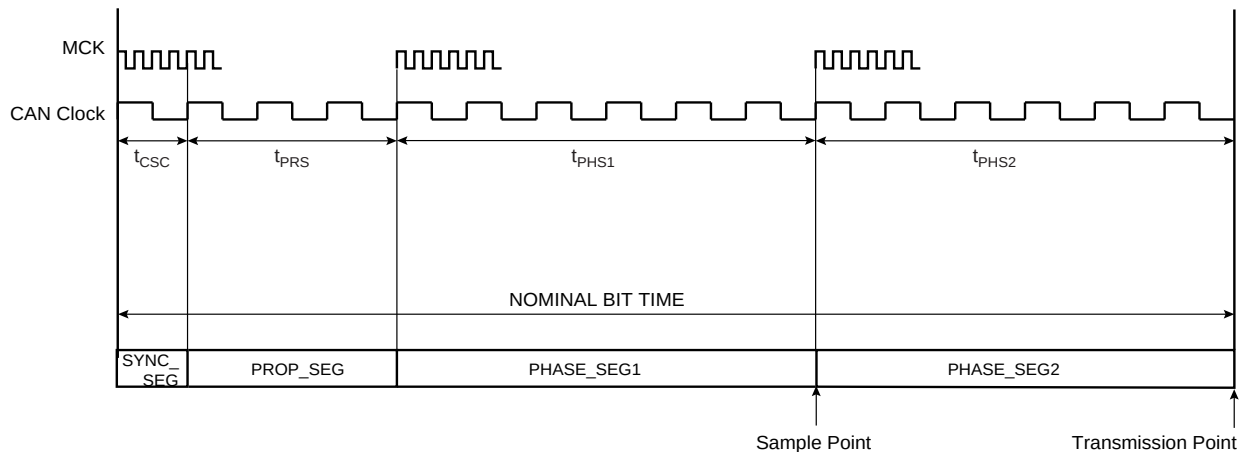
FIGURE 40-5: CAN BIT TIMING
