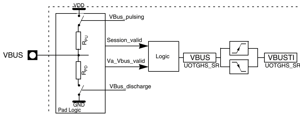
FIGURE 39-16: PLUG-IN DETECTION INPUT BLOCK DIAGRAM
