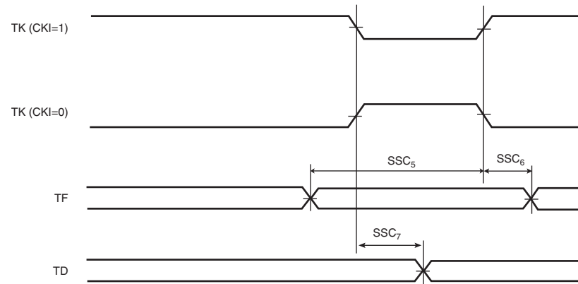
FIGURE 45-24: SSC TRANSMITTER, TK AND TF AS INPUT
