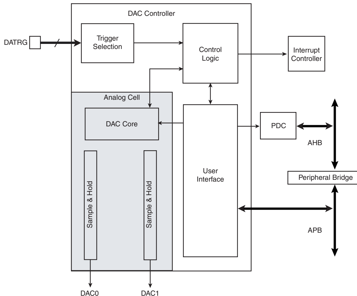
FIGURE 44-2: DIGITAL-TO-ANALOG CONVERTER CONTROLLER BLOCK DIAGRAM
