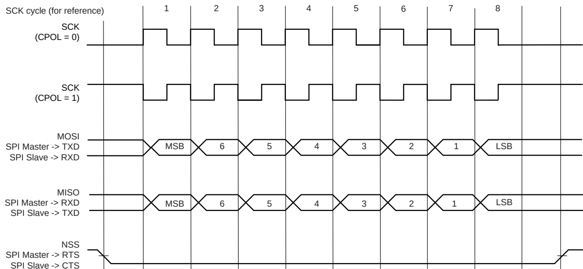
FIGURE 35-47: SPI TRANSFER FORMAT (CPHA=0, 8 BITS PER TRANSFER)
