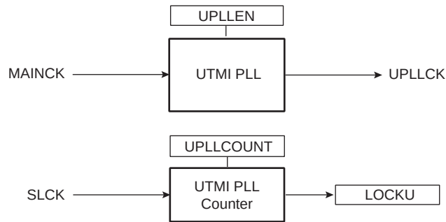
FIGURE 27-5: UTMI PLL BLOCK DIAGRAM
