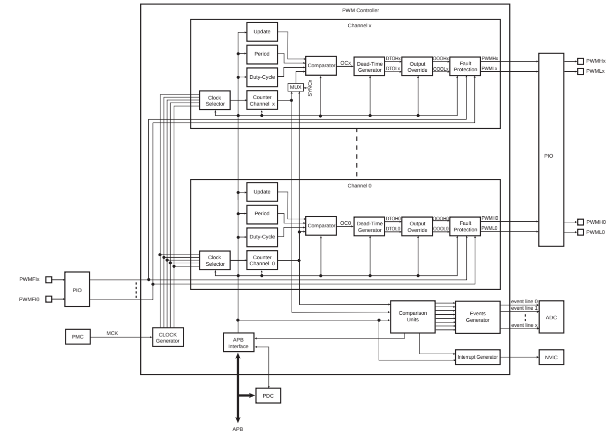
FIGURE 38-3: PULSE WIDTH MODULATION CONTROLLER BLOCK DIAGRAM
