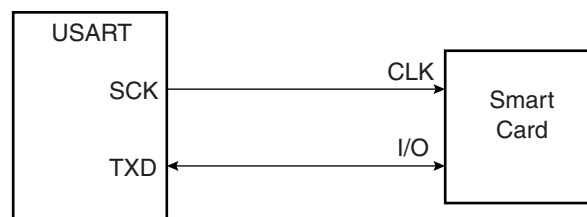
FIGURE 35-38: CONNECTION OF A SMART CARD TO THE USART
