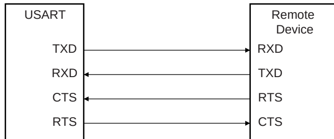
FIGURE 35-35: CONNECTION WITH A REMOTE DEVICE FOR HARDWARE HANDSHAKING
