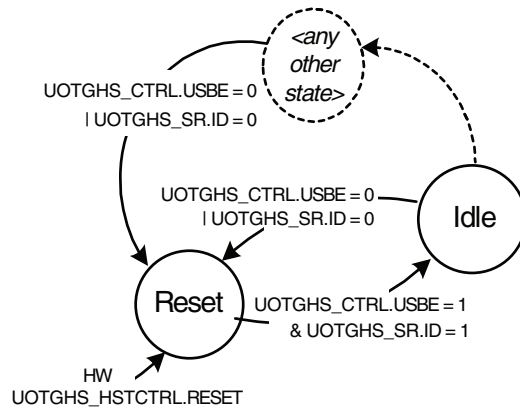
FIGURE 39-18: DEVICE MODE STATES
