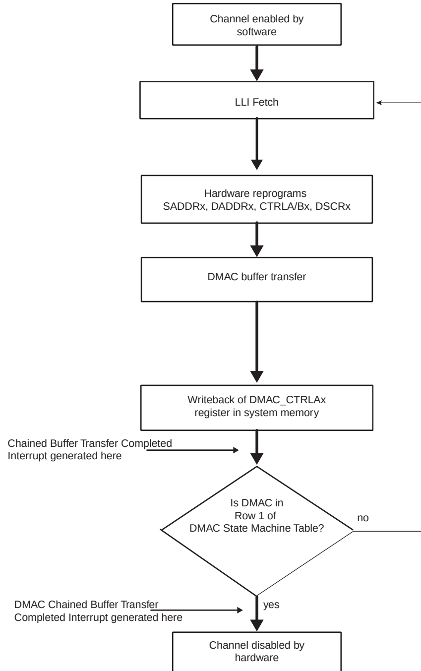
FIGURE 23-7: DMAC TRANSFER FLOW FOR SOURCE AND DESTINATION LINKED LIST ADDRESS
