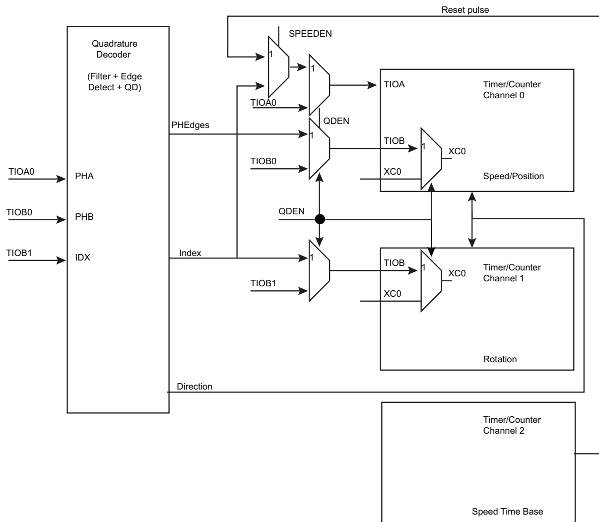
FIGURE 36-19: PREDEFINED CONNECTION OF THE QUADRATURE DECODER WITH TIMER COUNTERS
