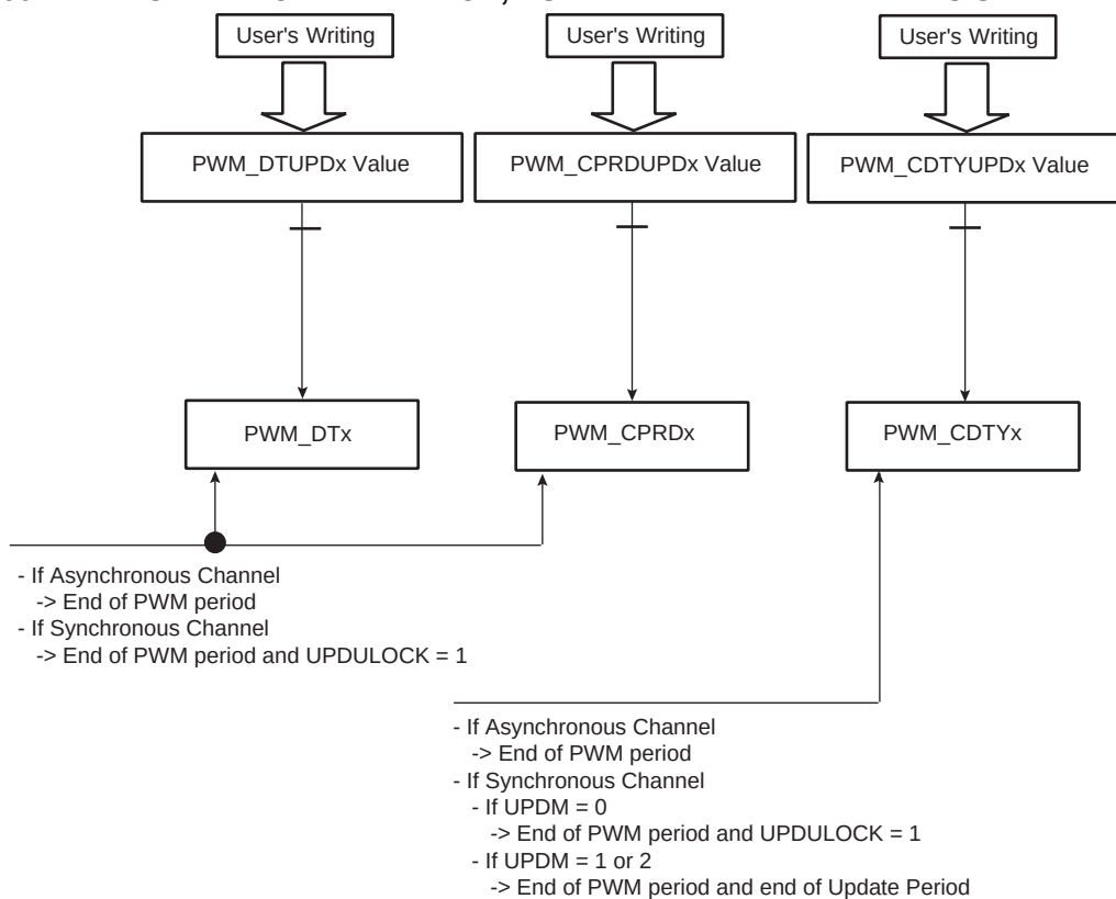
FIGURE 38-21: SYNCHRONIZED PERIOD, DUTY-CYCLE AND DEAD-TIMES UPDATE
