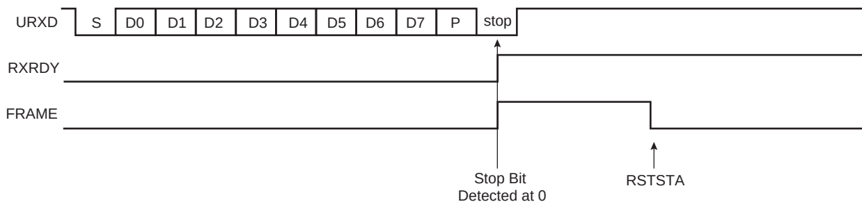
FIGURE 34-9: RECEIVER FRAMING ERROR
