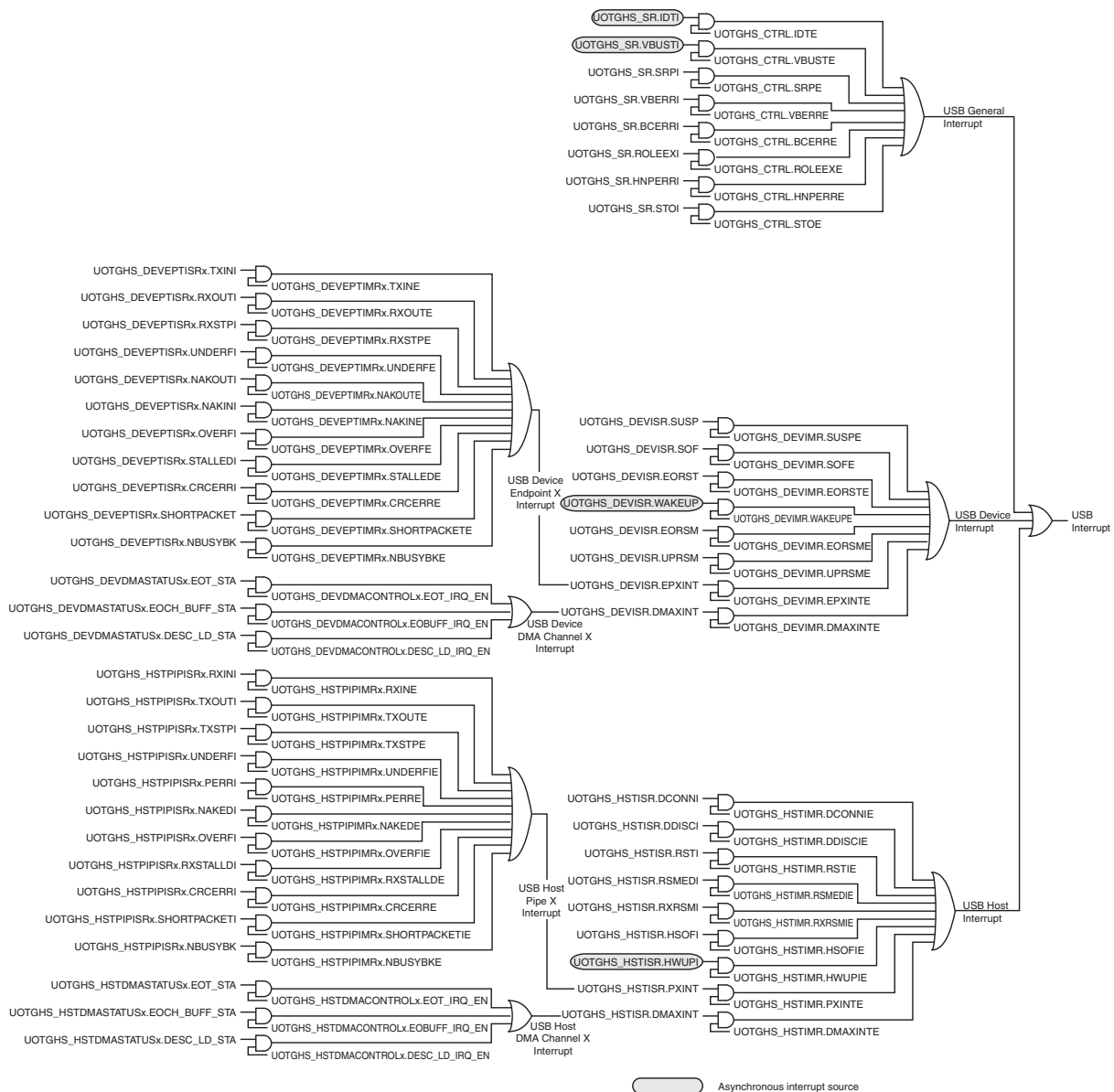
FIGURE 39-10: INTERRUPT SYSTEM
