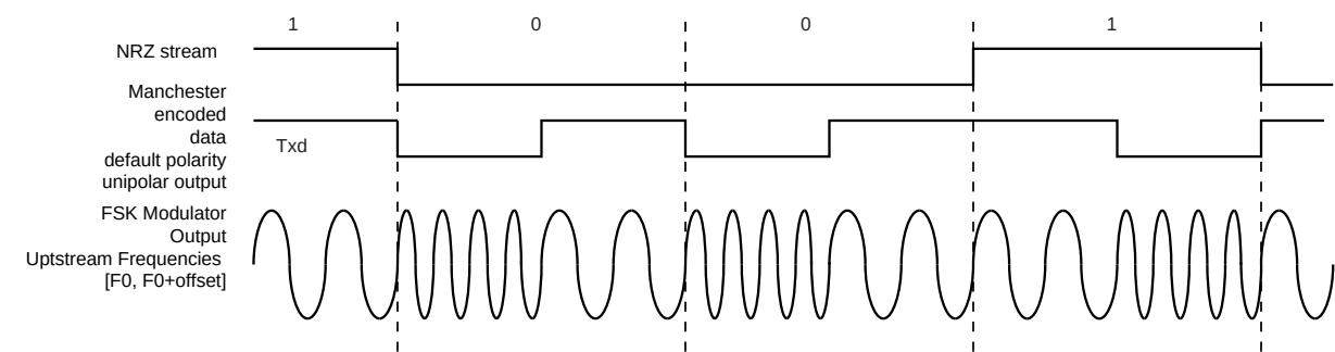
FIGURE 35-27: FSK MODULATOR OUTPUT
