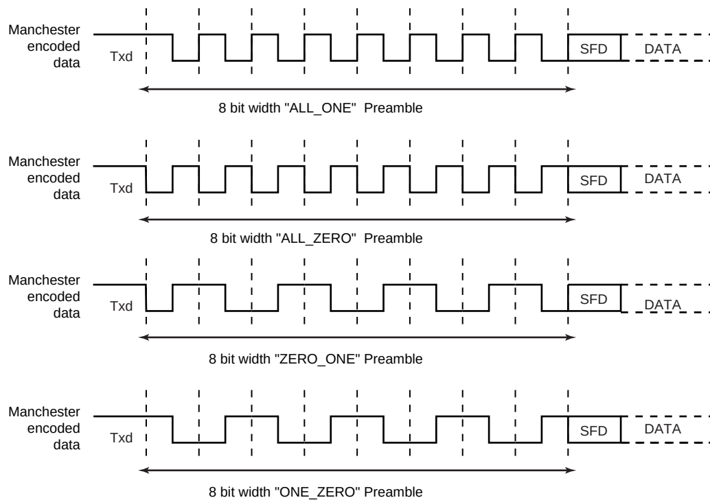
FIGURE 35-17: PREAMBLE PATTERNS, DEFAULT POLARITY ASSUMED
