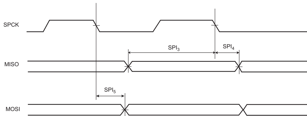
FIGURE 45-18: SPI MASTER MODE WITH (CPOL = 0 AND NCPHA = 1) OR (CPOL = 1 AND NCPHA = 0)
