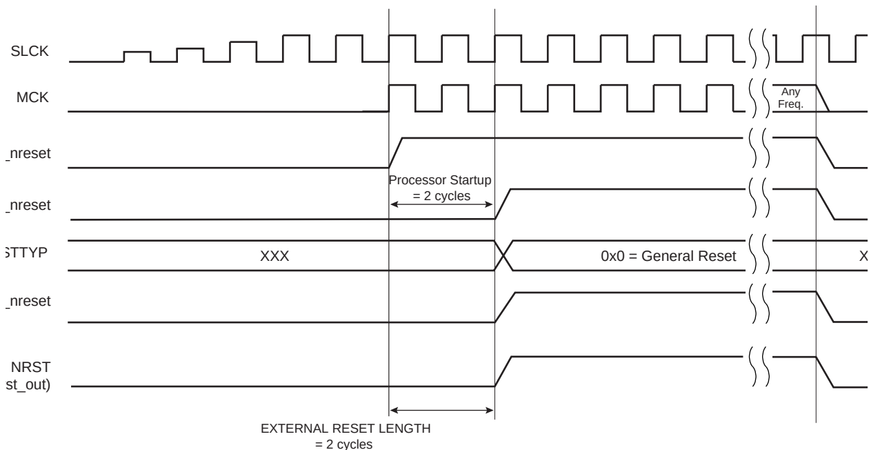
FIGURE 13-3: GENERAL RESET STATE
