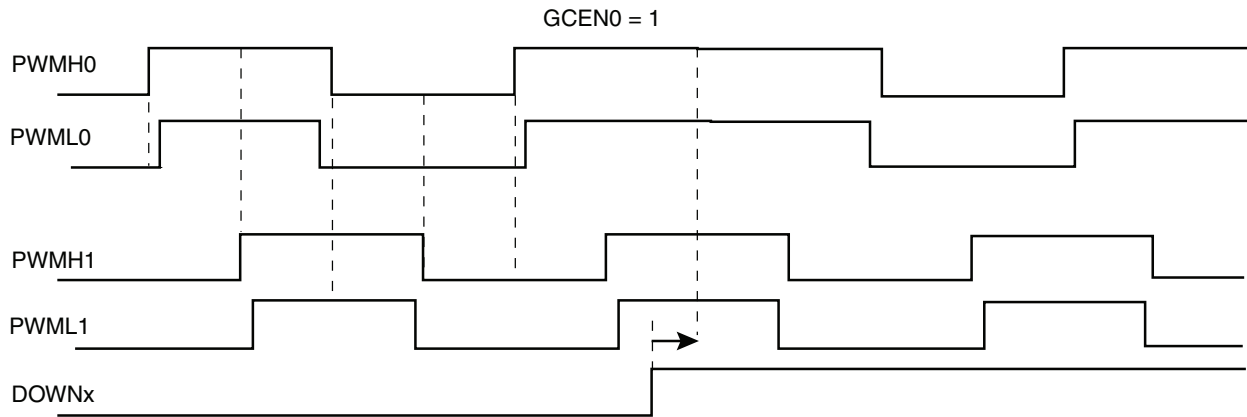
FIGURE 38-10: 2-BIT GRAY UP/DOWN COUNTER
