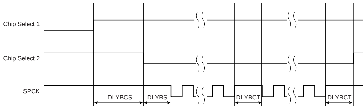
FIGURE 32-10: PROGRAMMABLE DELAYS
