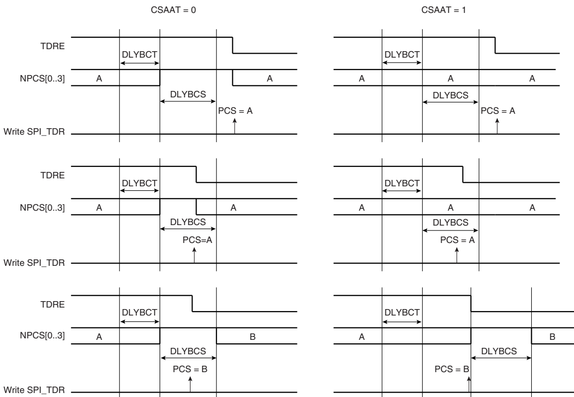
FIGURE 32-13: PERIPHERAL DESELECTION
