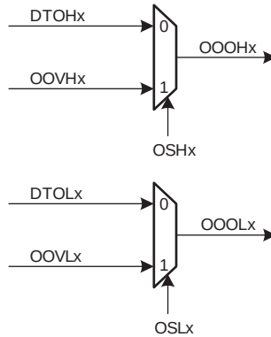
FIGURE 38-12: OVERRIDE OUTPUT SELECTION
