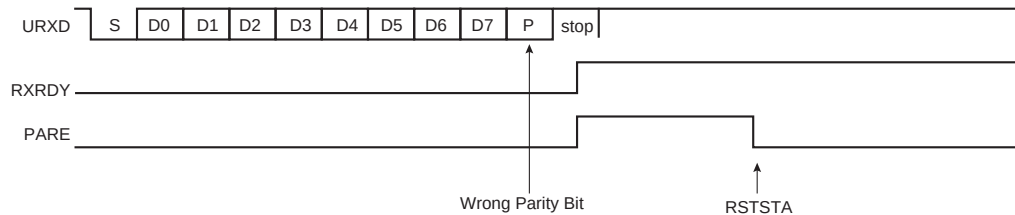
FIGURE 34-8: PARITY ERROR
