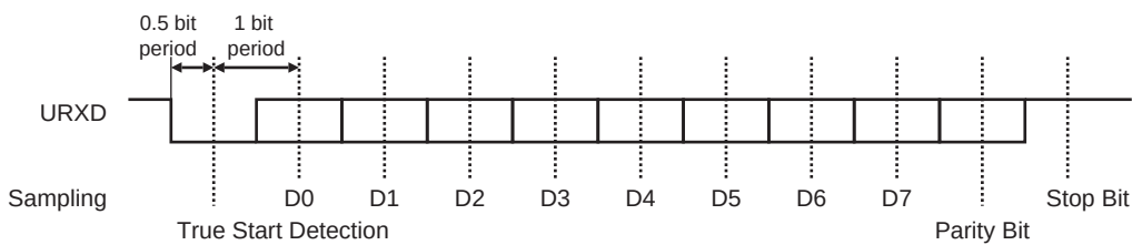
FIGURE 34-5: CHARACTER RECEPTION
