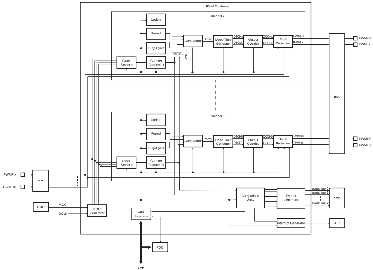
FIGURE 38-1: PULSE WIDTH MODULATION CONTROLLER BLOCK DIAGRAM
