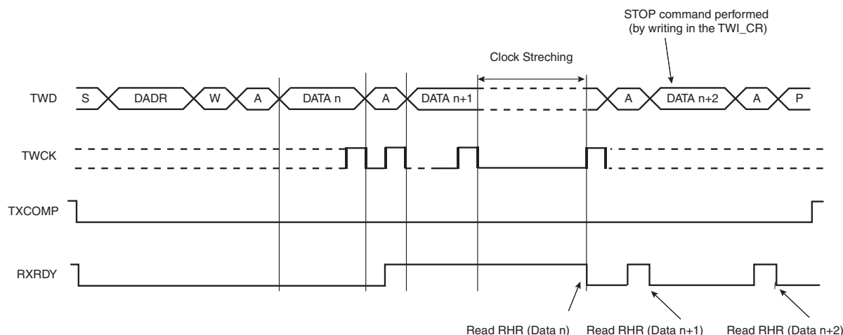
FIGURE 33-15: MASTER READ CLOCK STRETCHING WITH MULTIPLE DATA BYTES
