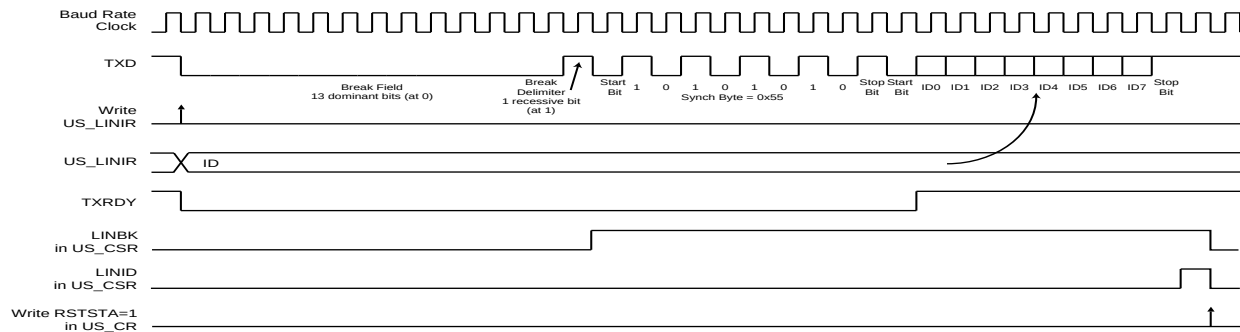
FIGURE 35-48: HEADER TRANSMISSION
