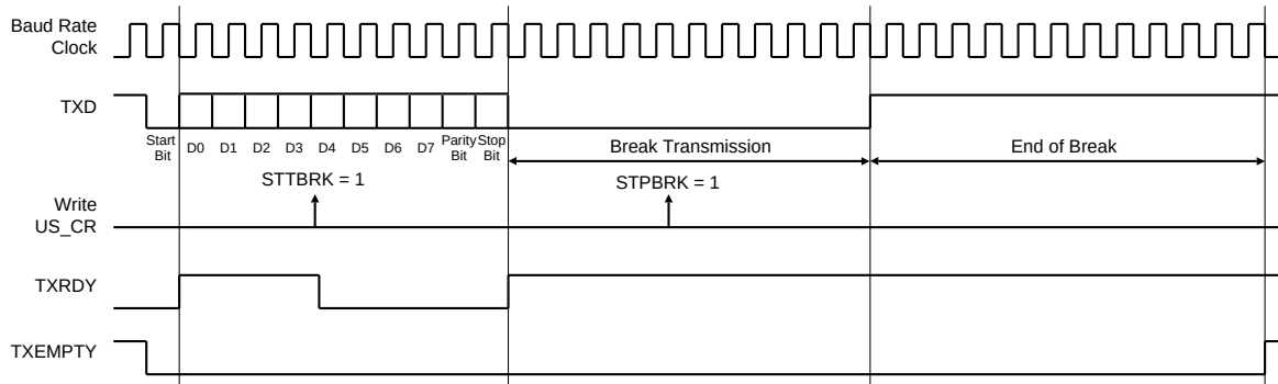
FIGURE 35-34: BREAK TRANSMISSION
