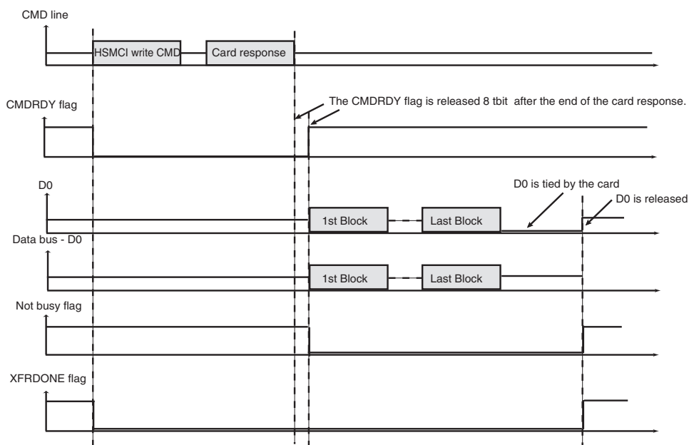
FIGURE 37-26: XFRDONE DURING A WRITE ACCESS
