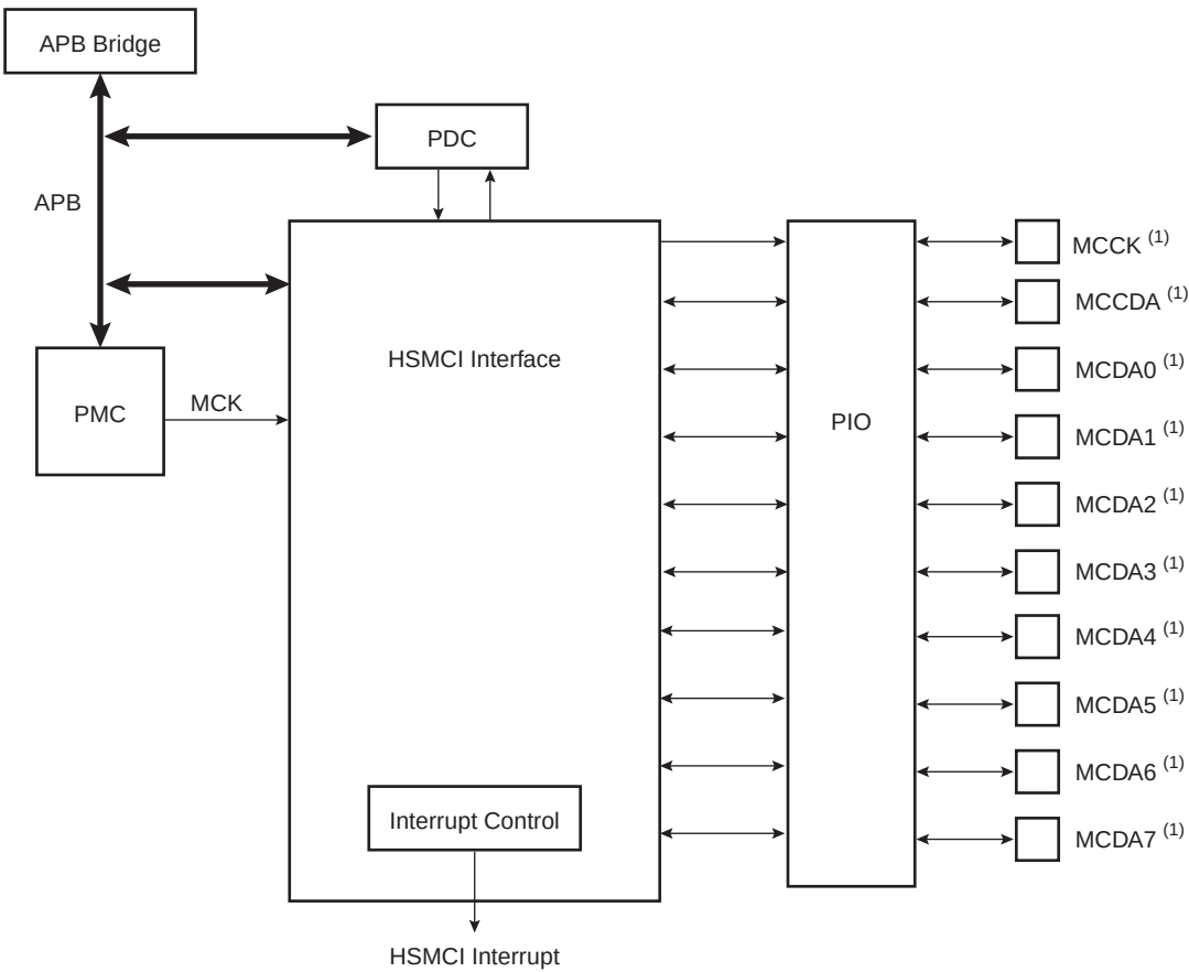
FIGURE 37-3: BLOCK DIAGRAM
