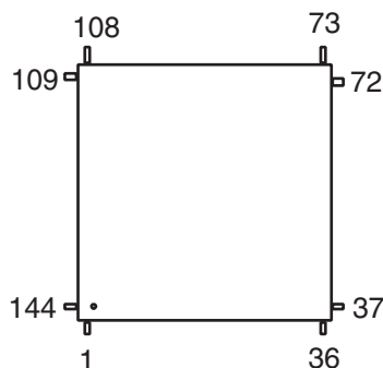
FIGURE 5-1: ORIENTATION OF THE 144-LEAD LQFP/CQFP PACKAGES
