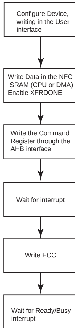
FIGURE 25-38: PROGRAM PAGE FLOW CHART
