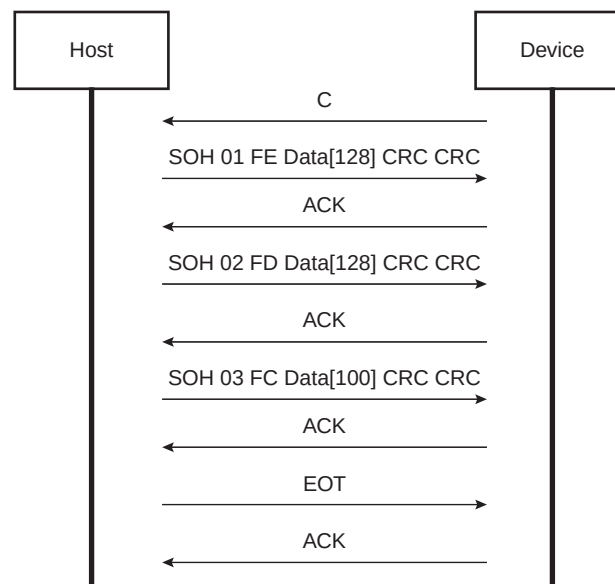
FIGURE 21-1: XMODEM TRANSFER EXAMPLE
