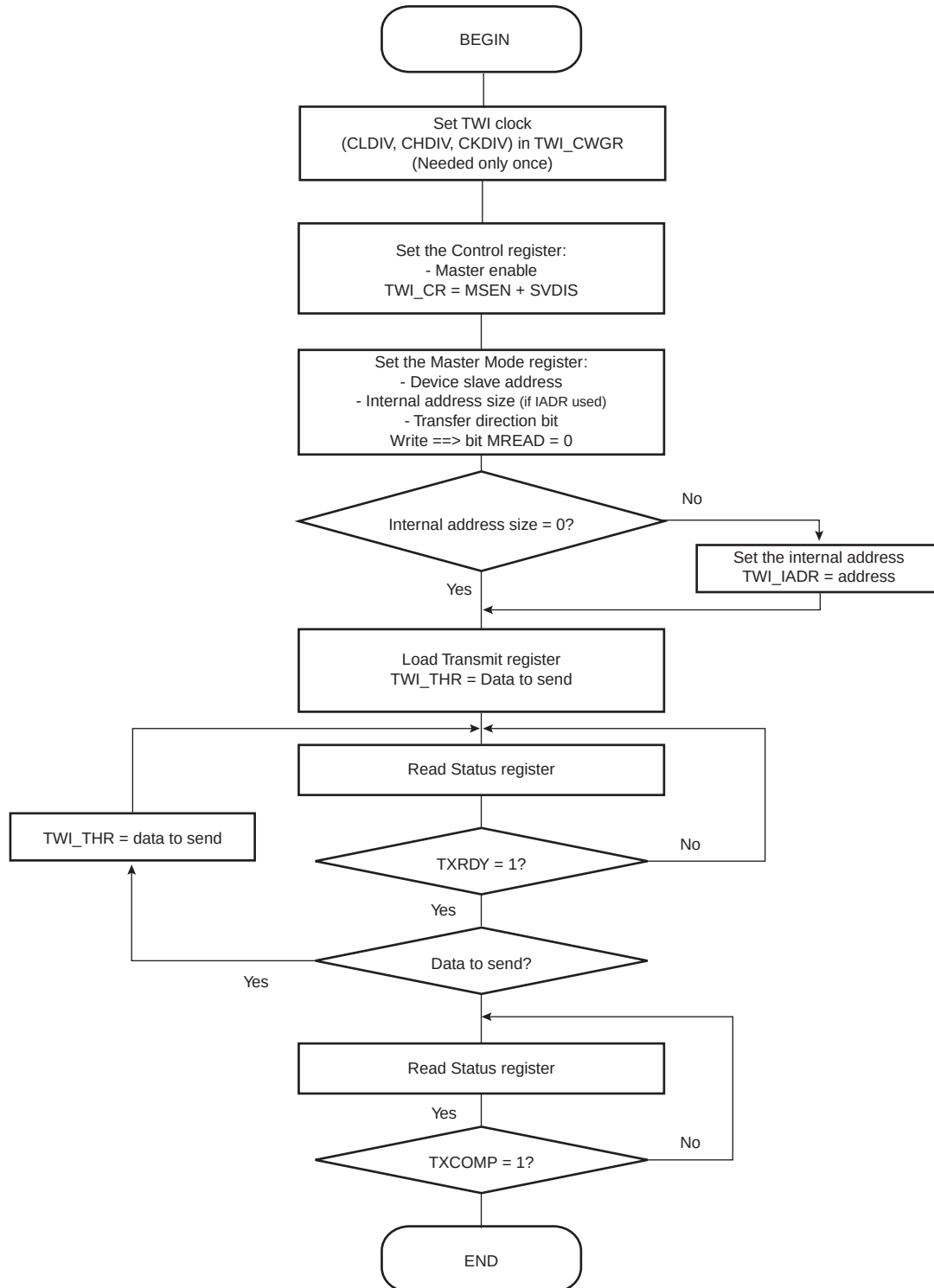
FIGURE 33-25: TWI WRITE OPERATION WITH MULTIPLE DATA BYTES WITH OR WITHOUT INTERNAL ADDRESS
