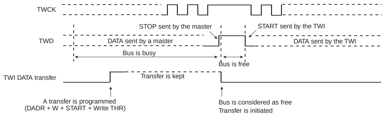
FIGURE 33-29: PROGRAMMER SENDS DATA WHILE THE BUS IS BUSY
