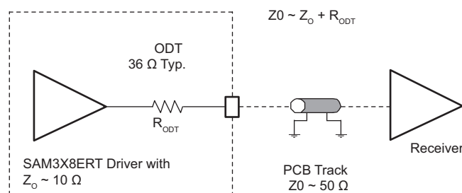
FIGURE 7-1: ON-DIE TERMINATION
