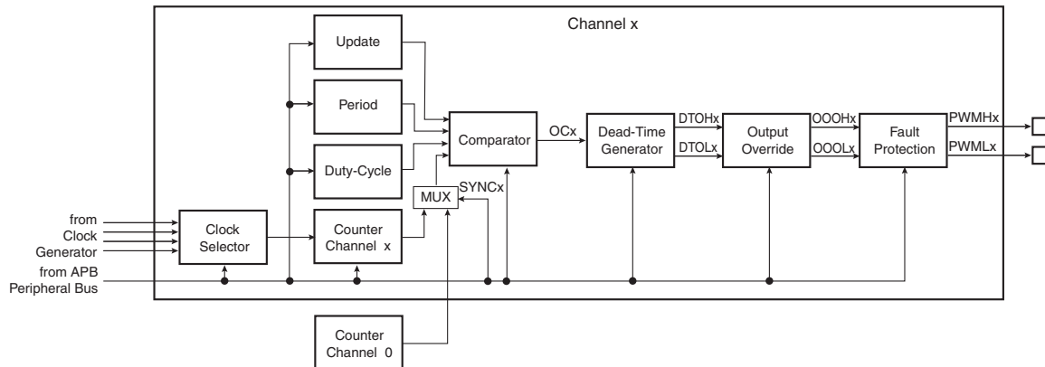
FIGURE 38-6: FUNCTIONAL VIEW OF THE CHANNEL BLOCK DIAGRAM
