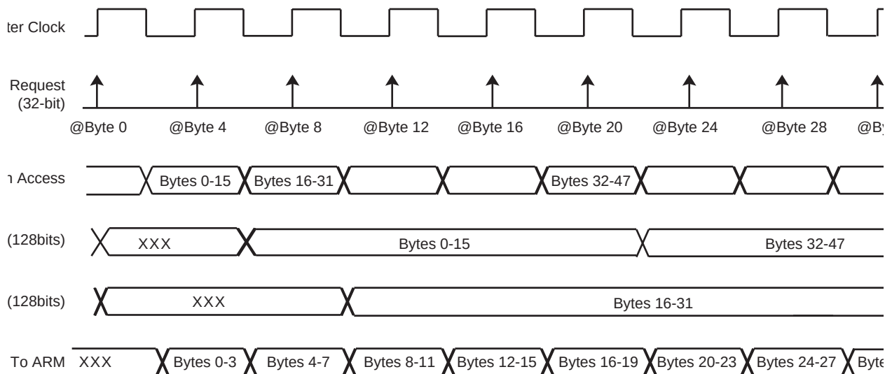
FIGURE 19-2: CODE READ OPTIMIZATION FOR FWS = 0
