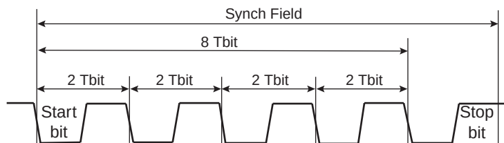
FIGURE 35-50: SYNCH FIELD
