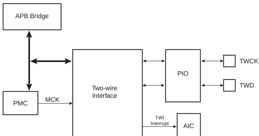
FIGURE 33-1: BLOCK DIAGRAM
