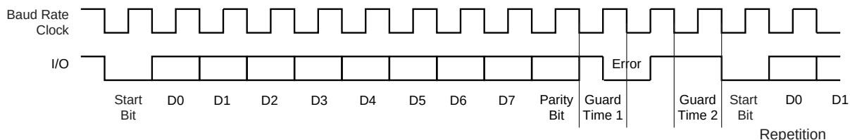
FIGURE 35-40: T = 0 PROTOCOL WITH PARITY ERROR
