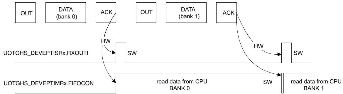
FIGURE 39-26: EXAMPLE OF AN OUT ENDPOINT WITH TWO DATA BANKS
