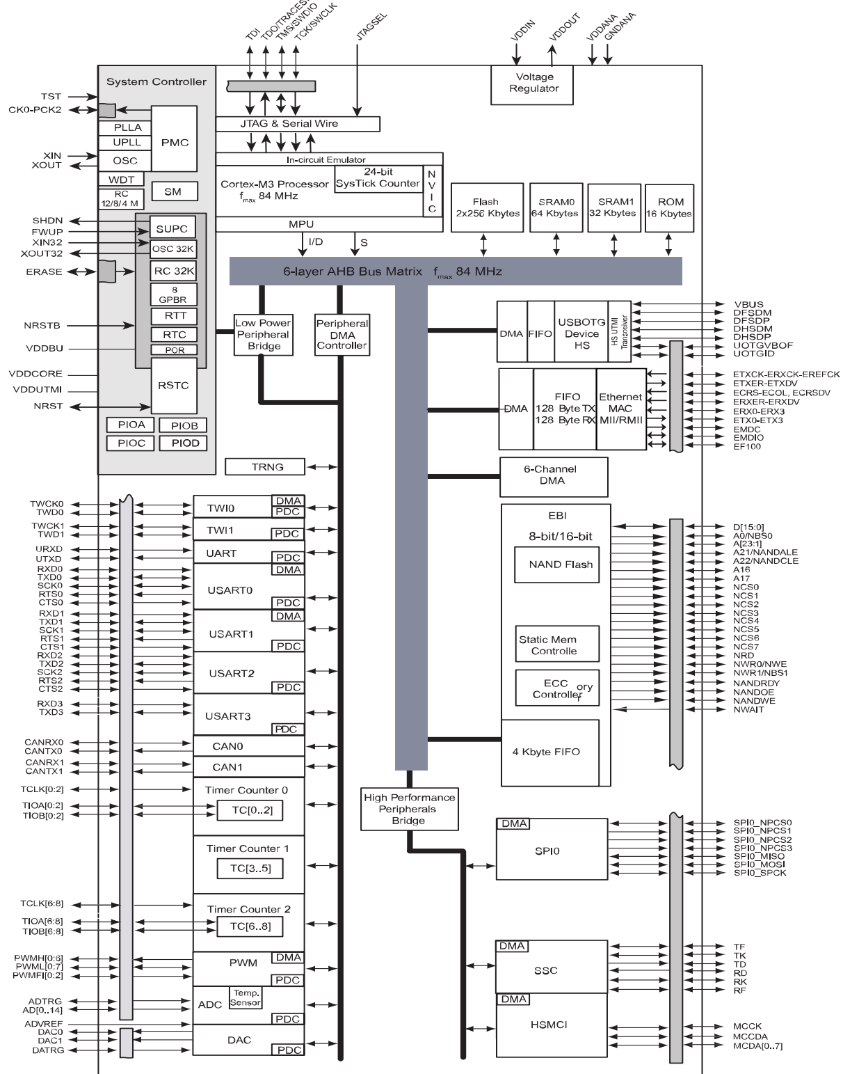
FIGURE 2-1: SAM3X8ERT BLOCK DIAGRAM
