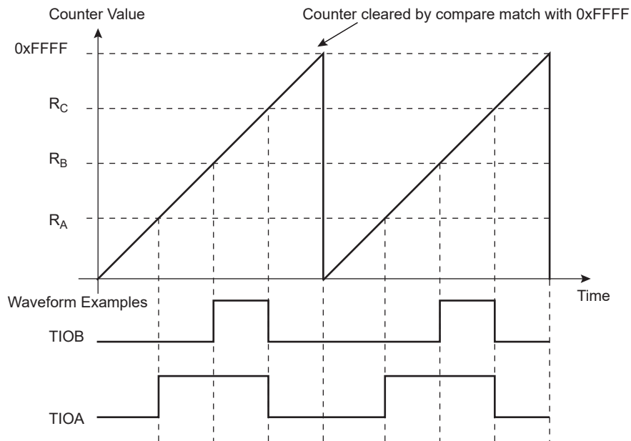
FIGURE 36-10: WAVSEL = 00 WITHOUT TRIGGER
