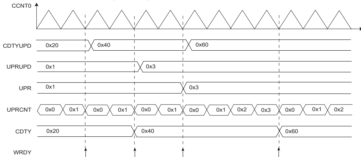
FIGURE 38-15: METHOD 2 (UPDM=1)
