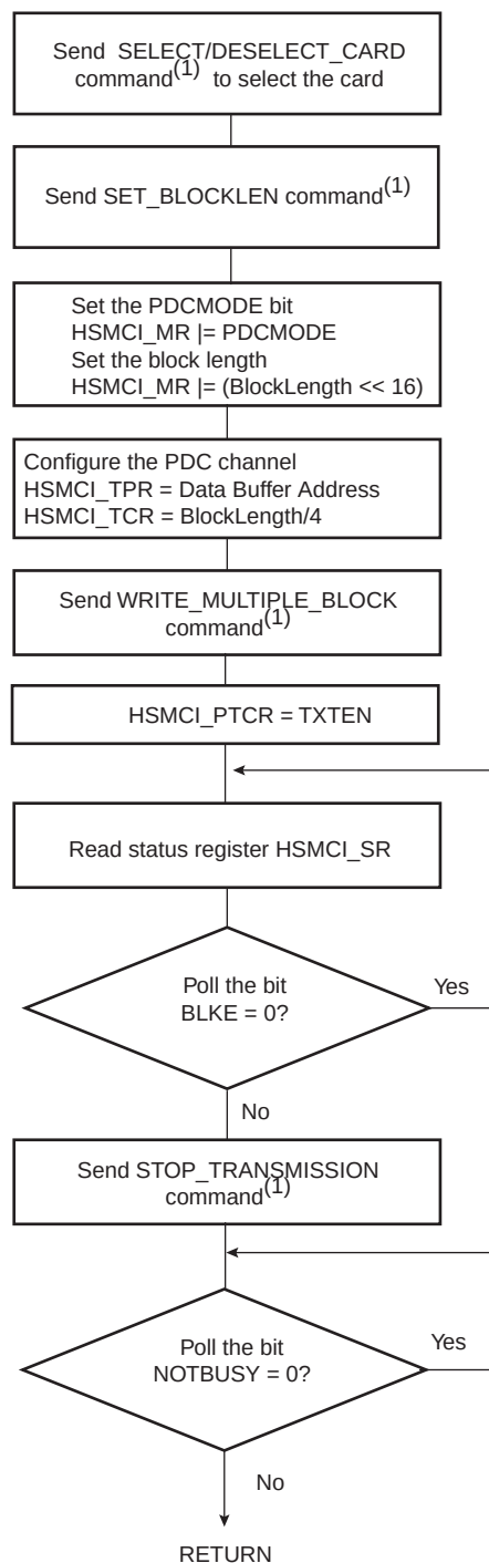
FIGURE 37-22: MULTIPLE WRITE FUNCTIONAL FLOW DIAGRAM
