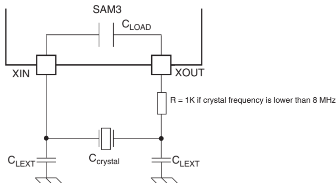
FIGURE 45-12: 3 TO 20 MHZ CRYSTAL OSCILLATOR SCHEMATIC
