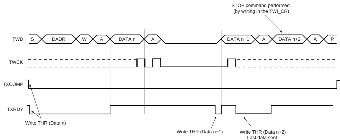
FIGURE 33-8: MASTER WRITE WITH MULTIPLE DATA BYTES
