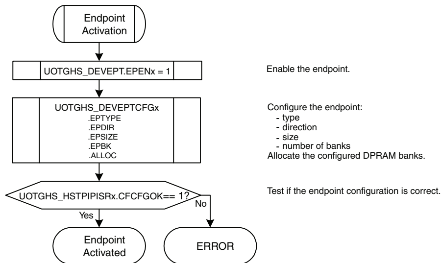
FIGURE 39-19: ENDPOINT ACTIVATION ALGORITHM
