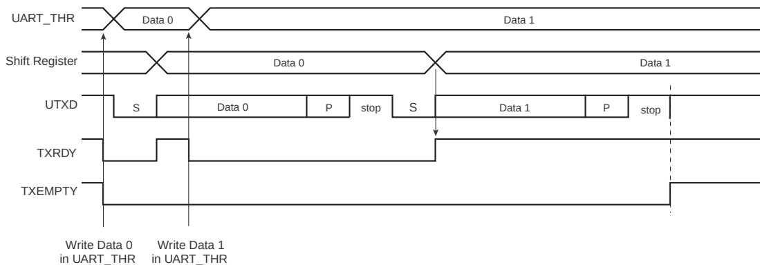
FIGURE 34-11: TRANSMITTER CONTROL
