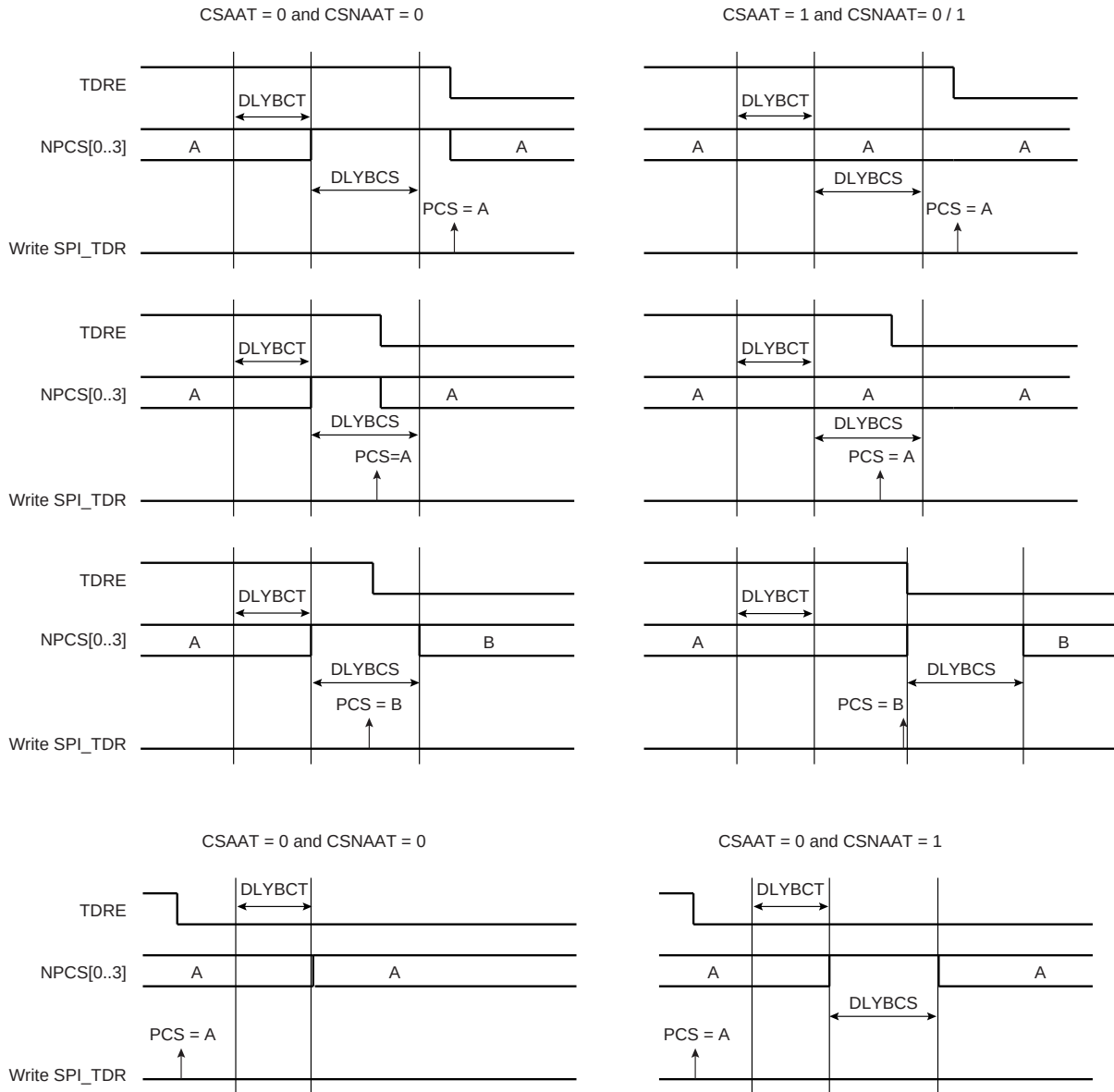
FIGURE 32-12: PERIPHERAL DESELECTION
