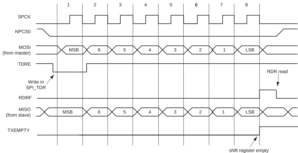
FIGURE 32-8: STATUS REGISTER FLAGS BEHAVIOR
