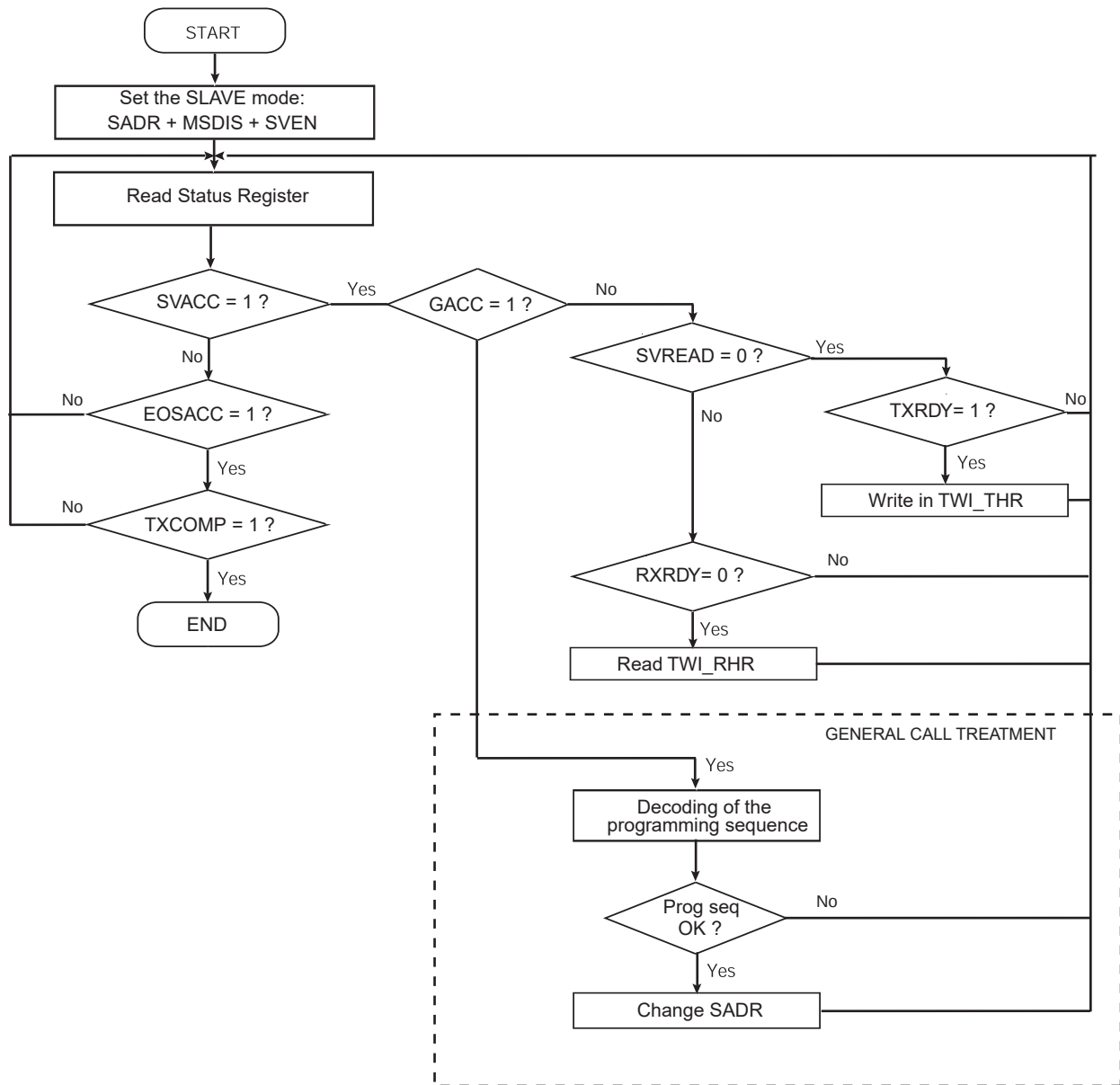
FIGURE 33-41: READ WRITE FLOWCHART IN SLAVE MODE
