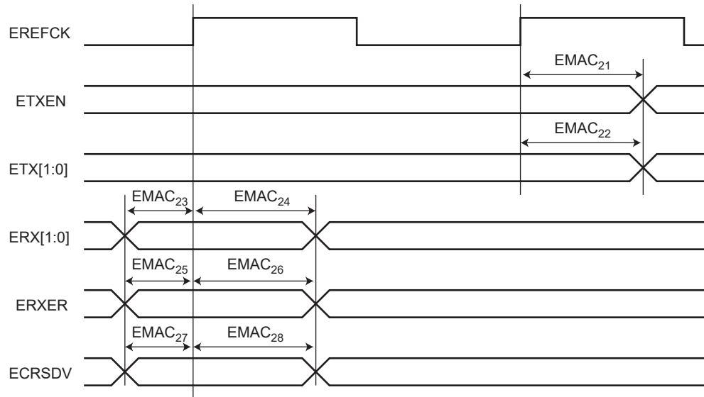
FIGURE 45-37: EMAC RMII TIMINGS
