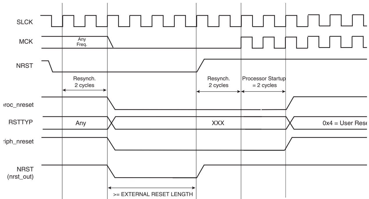
FIGURE 13-4: USER RESET STATE
