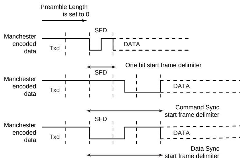
FIGURE 35-18: START FRAME DELIMITER
