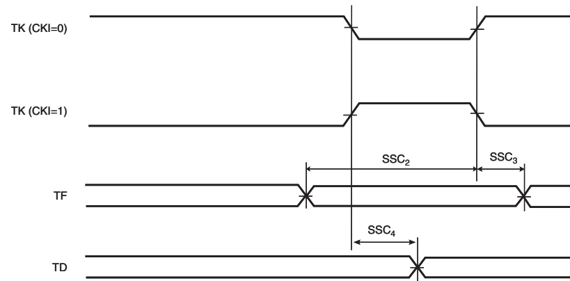
FIGURE 45-23: SSC TRANSMITTER, TK AS OUTPUT AND TF AS INPUT
