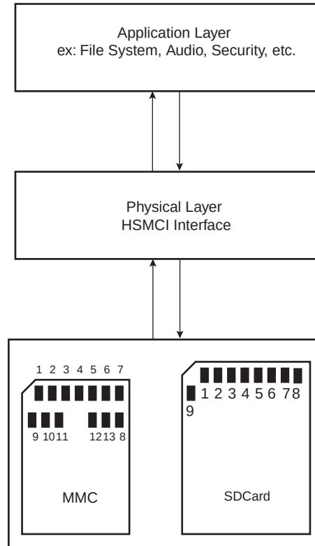
FIGURE 37-12: APPLICATION BLOCK DIAGRAM
