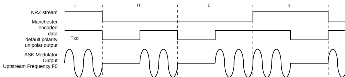
FIGURE 35-26: ASK MODULATOR OUTPUT
