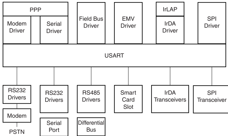
FIGURE 35-5: APPLICATION BLOCK DIAGRAM
