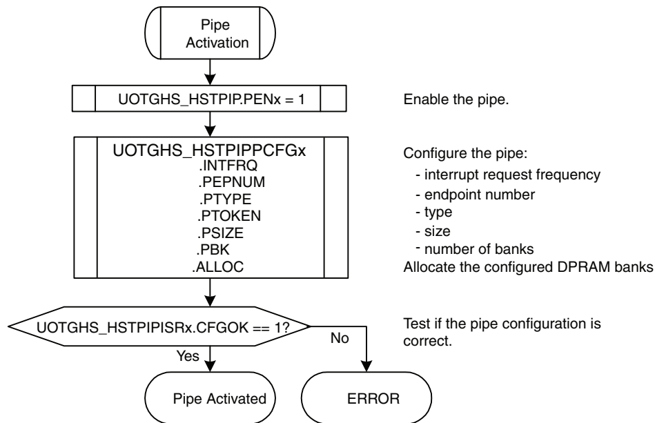
FIGURE 39-29: PIPE ACTIVATION ALGORITHM
