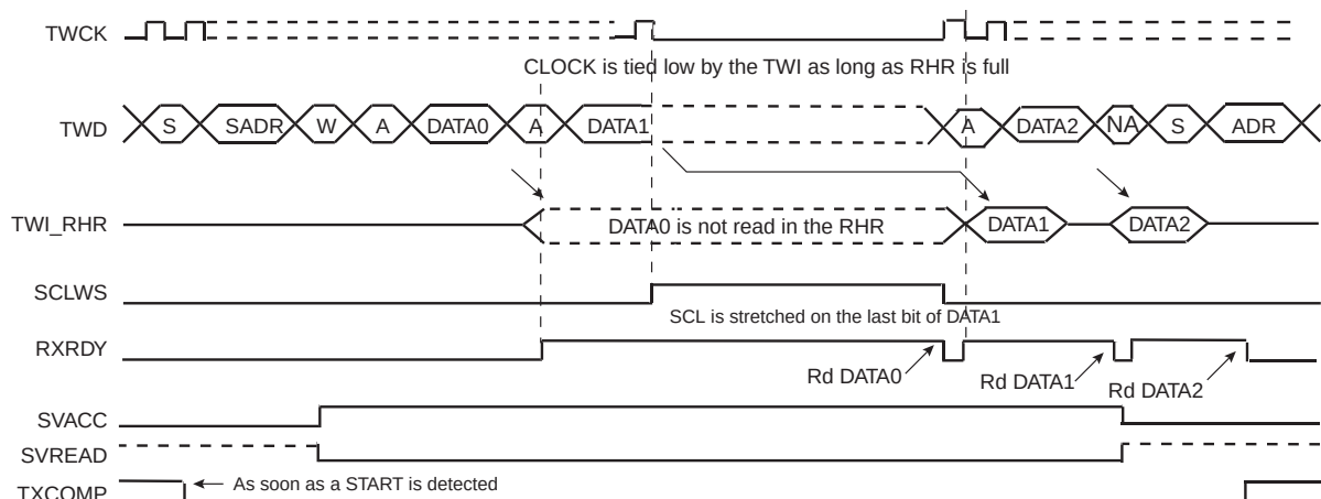
FIGURE 33-38: CLOCK SYNCHRONIZATION IN WRITE MODE
