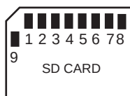
FIGURE 37-15: SD MEMORY CARD BUS TOPOLOGY
