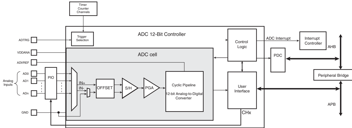
FIGURE 43-7: ANALOG-TO-DIGITAL CONVERTER BLOCK DIAGRAM
