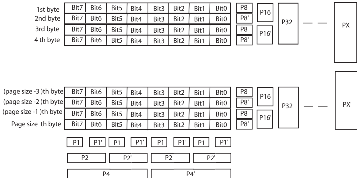
FIGURE 25-39: PARITY GENERATION FOR 512/1024/2048/4096 8-BIT WORDS
