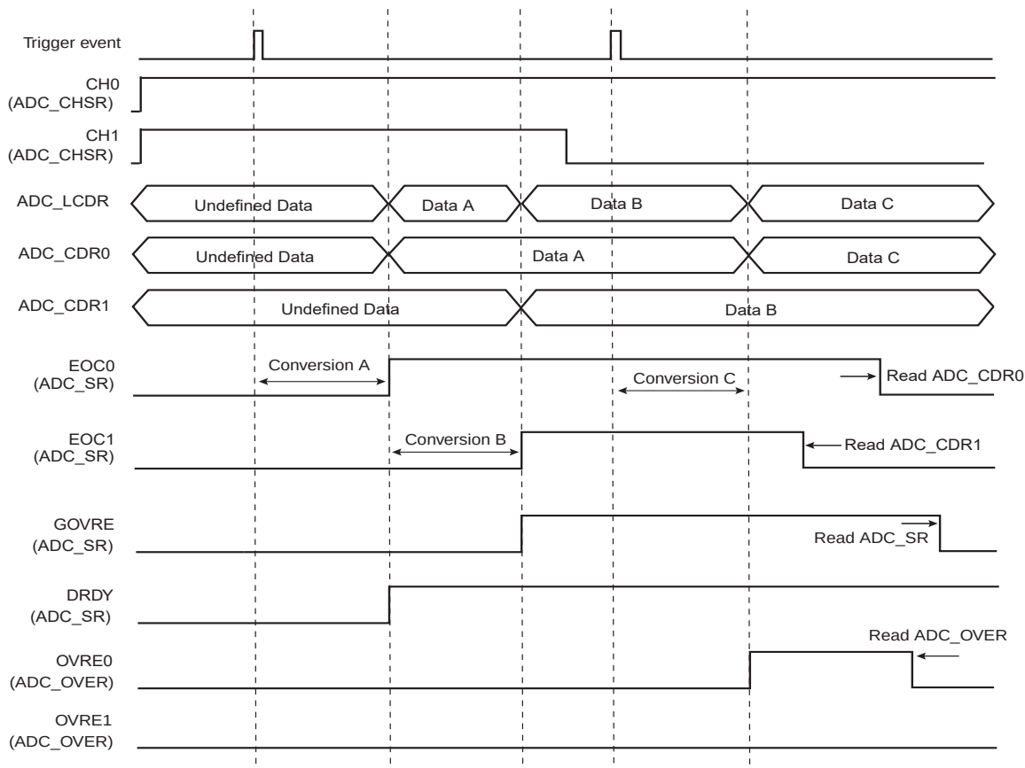
FIGURE 43-12: GOVRE AND OVREX FLAG BEHAVIOR
