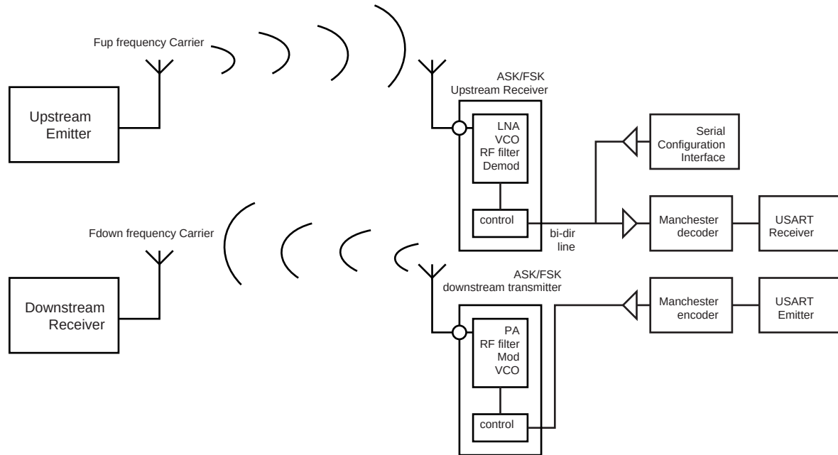
FIGURE 35-25: MANCHESTER ENCODED CHARACTERS RF TRANSMISSION
