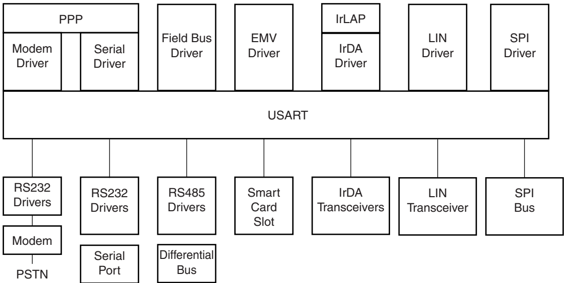
FIGURE 35-3: APPLICATION BLOCK DIAGRAM
