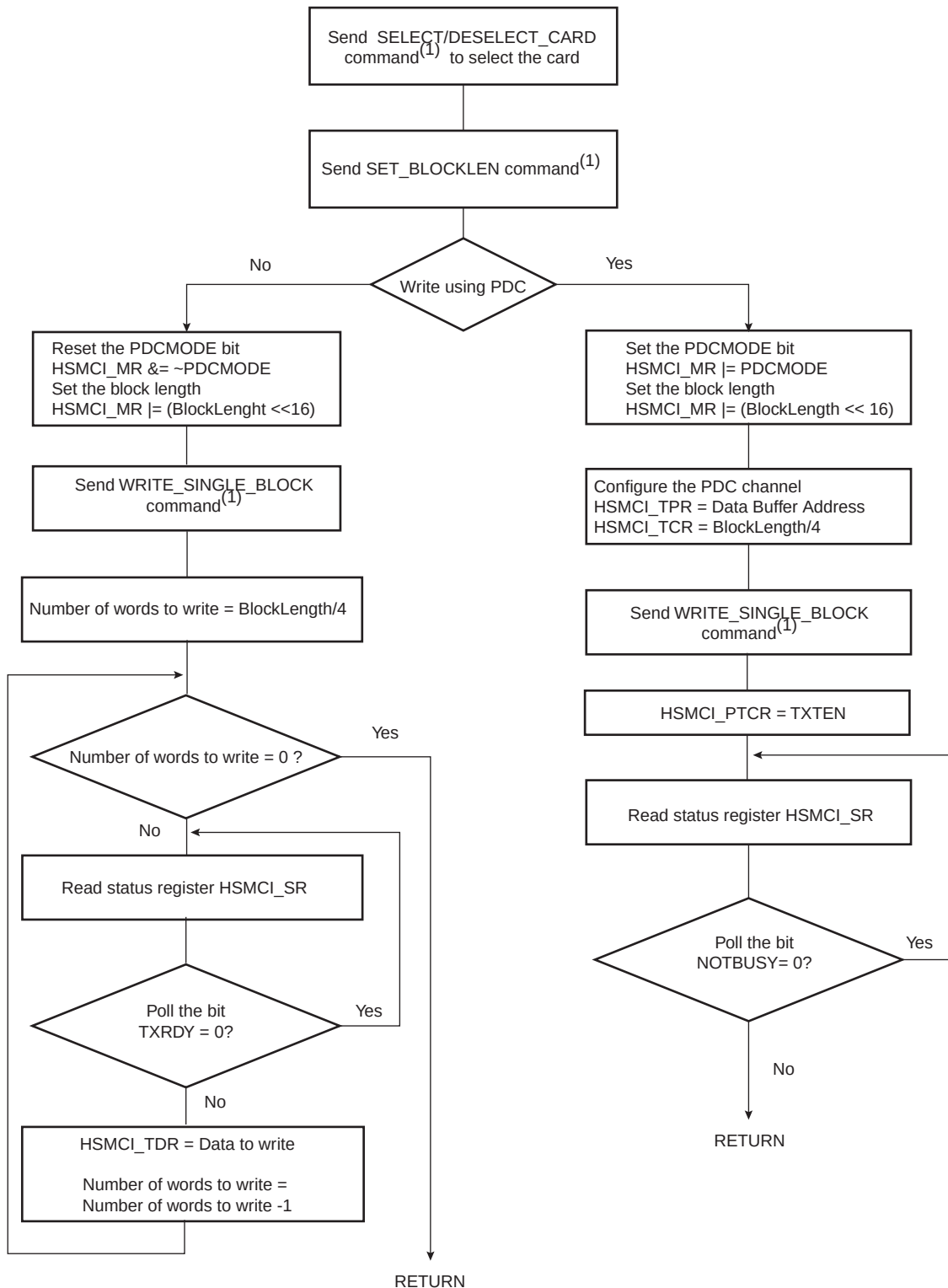
FIGURE 37-21: WRITE FUNCTIONAL FLOW DIAGRAM
