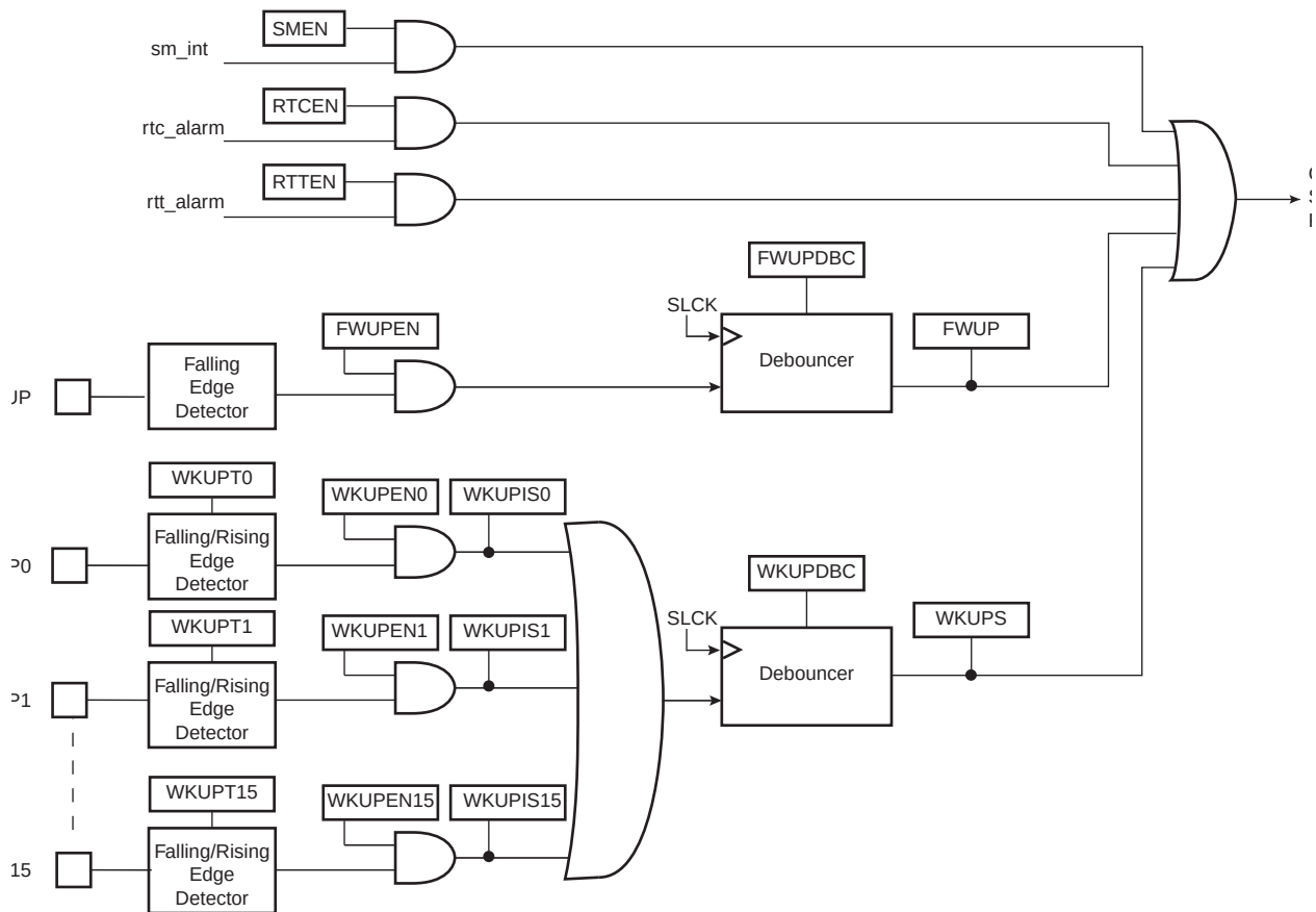
FIGURE 17-7: WAKE UP SOURCE
