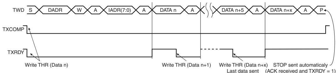
FIGURE 33-12: MASTER WRITE WITH ONE BYTE INTERNAL ADDRESS AND MULTIPLE DATA BYTES
