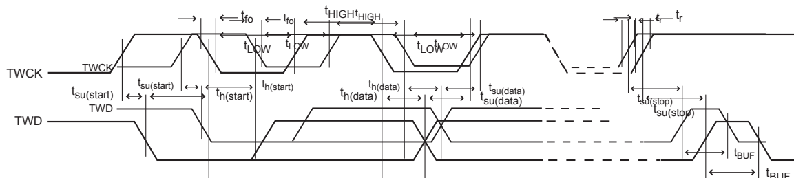
FIGURE 45-38: TWO-WIRE SERIAL BUS TIMING
