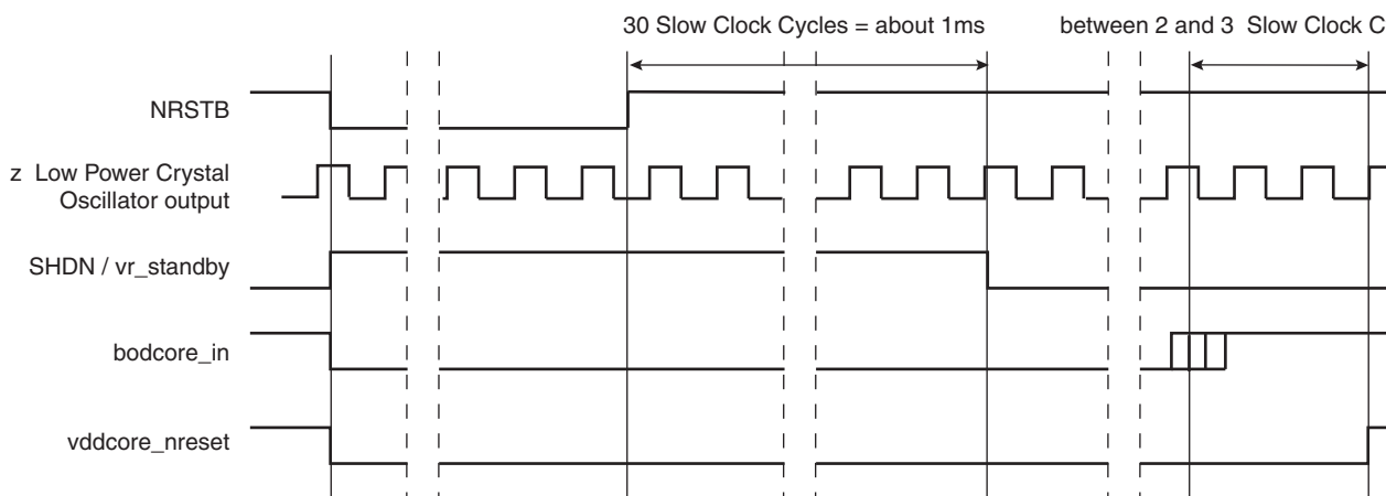
FIGURE 17-6: NRSTB RESET
