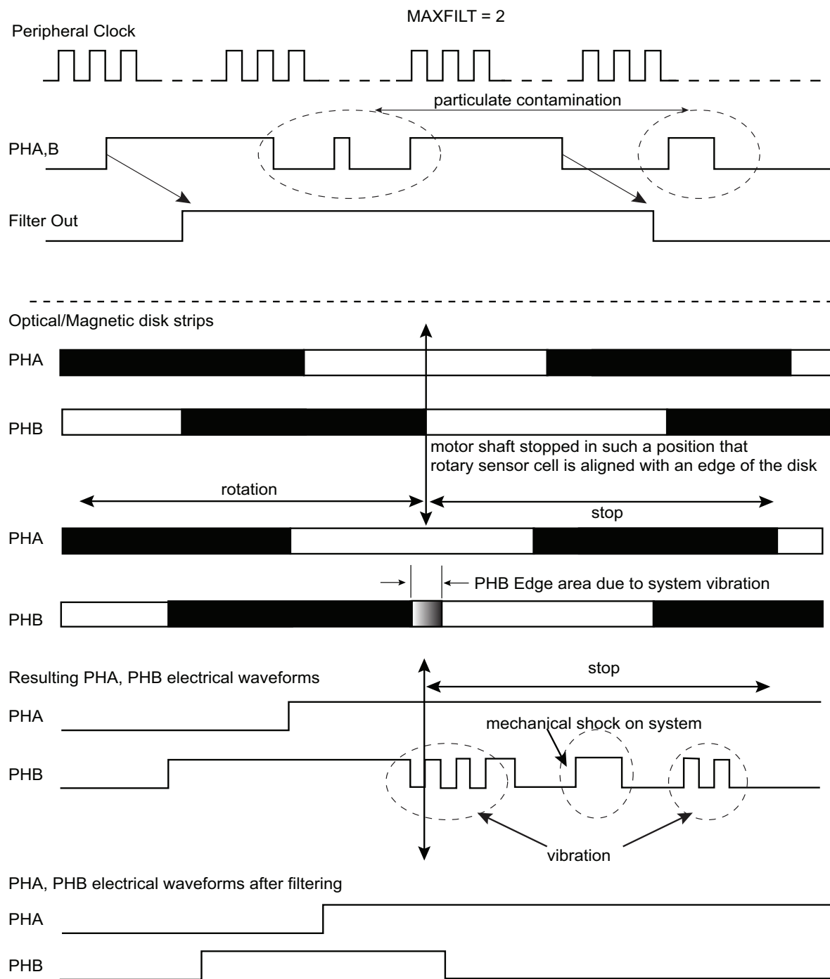
FIGURE 36-21: FILTERING EXAMPLES
