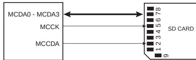
FIGURE 37-16: SD CARD BUS CONNECTIONS WITH ONE SLOT
