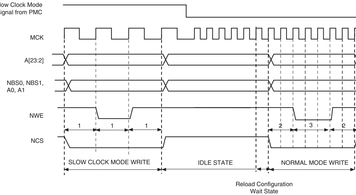
FIGURE 25-30: RECOMMENDED PROCEDURE TO SWITCH FROM SLOW CLOCK MODE TO NORMAL MODE OR FROM NORMAL MODE TO SLOW CLOCK MODE
