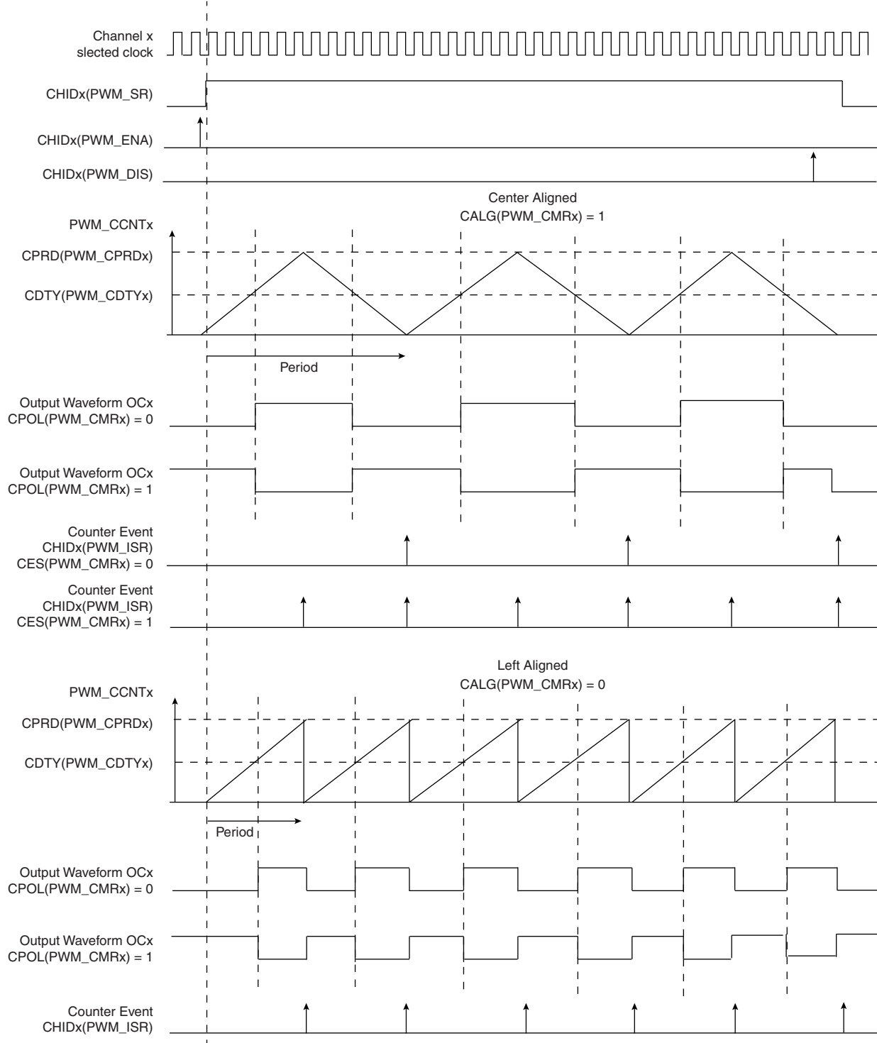
FIGURE 38-9: WAVEFORM PROPERTIES
