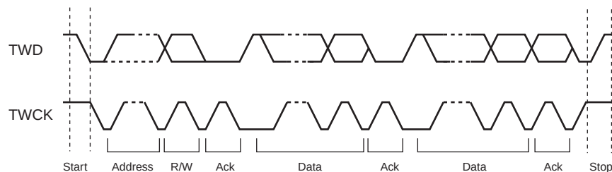
FIGURE 33-5: TRANSFER FORMAT
