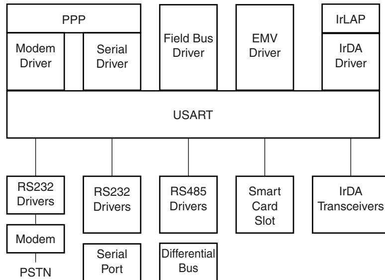
FIGURE 35-6: APPLICATION BLOCK DIAGRAM
