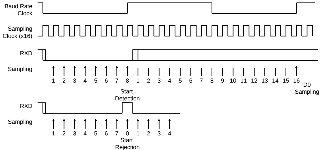
FIGURE 35-21: ASYNCHRONOUS CHARACTER RECEPTION
