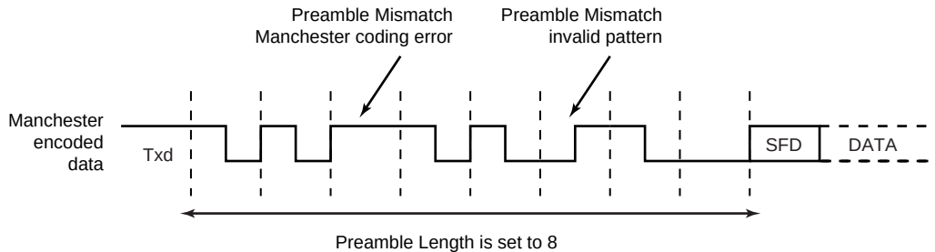
FIGURE 35-23: PREAMBLE PATTERN MISMATCH
