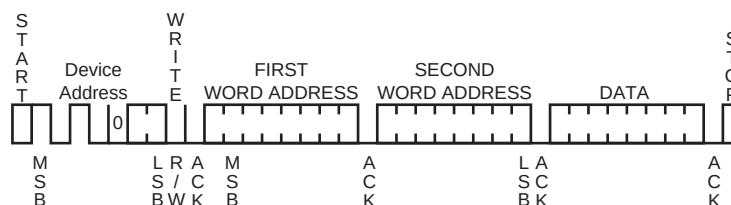
FIGURE 33-18: INTERNAL ADDRESS USAGE
