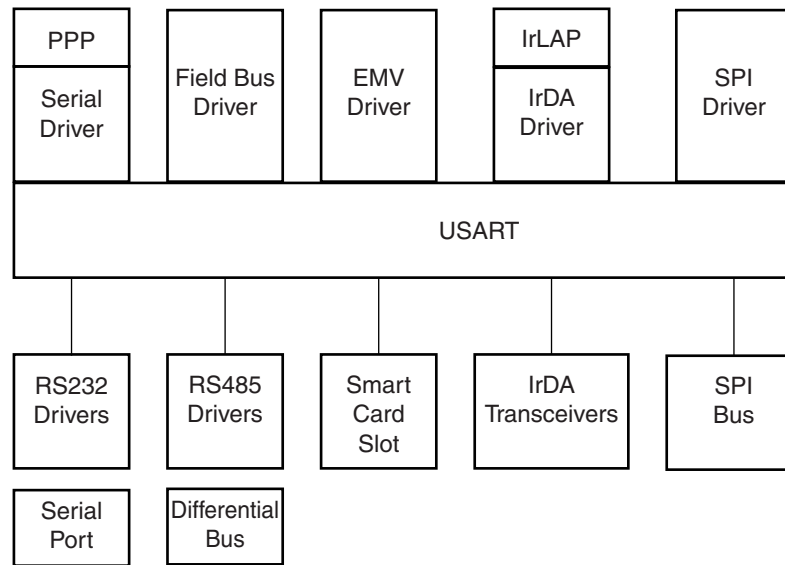
FIGURE 35-9: APPLICATION BLOCK DIAGRAM
