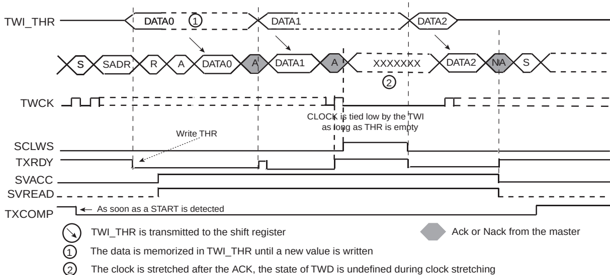
FIGURE 33-37: CLOCK SYNCHRONIZATION IN READ MODE
