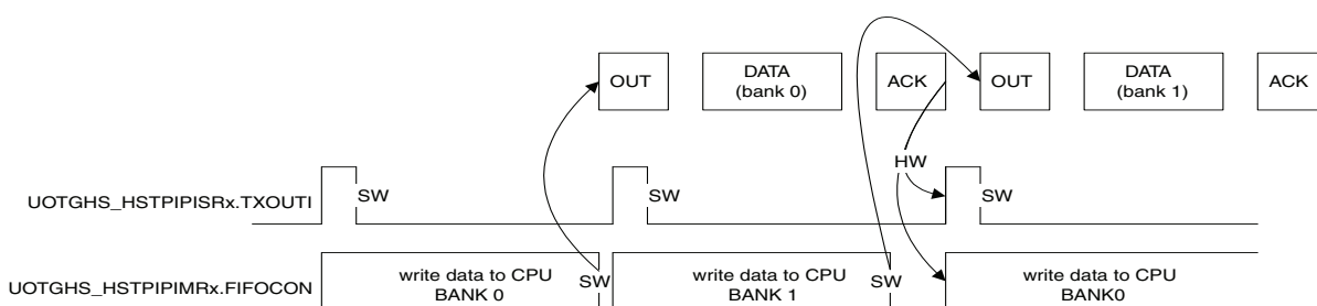
FIGURE 39-34: EXAMPLE OF AN OUT PIPE WITH TWO DATA BANKS AND A BANK SWITCHING DELAY
