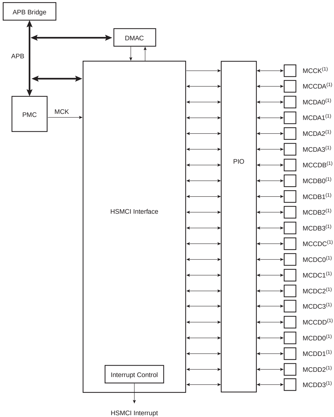
FIGURE 37-10: BLOCK DIAGRAM
