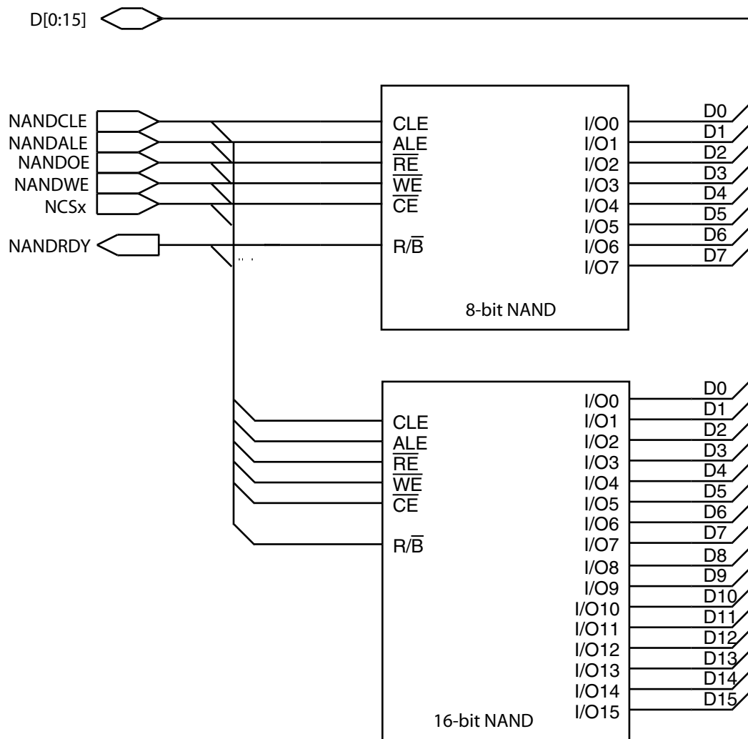
FIGURE 24-2: 8-BIT AND 16-BIT NAND FLASH HARDWARE CONFIGURATION
