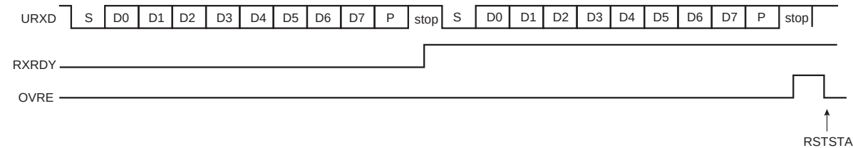
FIGURE 34-7: RECEIVER OVERRUN
