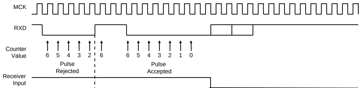
FIGURE 35-43: IRDA DEMODULATOR OPERATIONS
