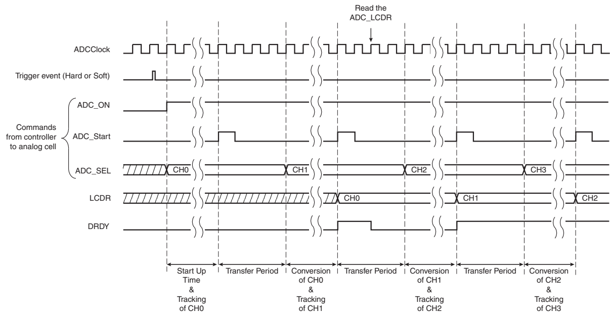
FIGURE 43-9: SEQUENCE OF ADC CONVERSIONS WHEN TRACKING TIME < CONVERSION TIME
