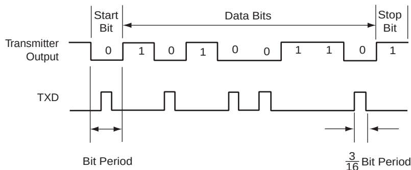
FIGURE 35-42: IRDA MODULATION
