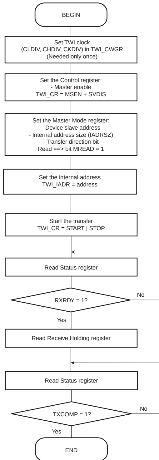
FIGURE 33-27: TWI READ OPERATION WITH SINGLE DATA BYTE AND INTERNAL ADDRESS
