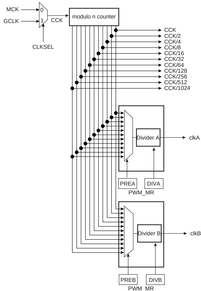
FIGURE 38-4: FUNCTIONAL VIEW OF THE CLOCK GENERATOR BLOCK DIAGRAM
