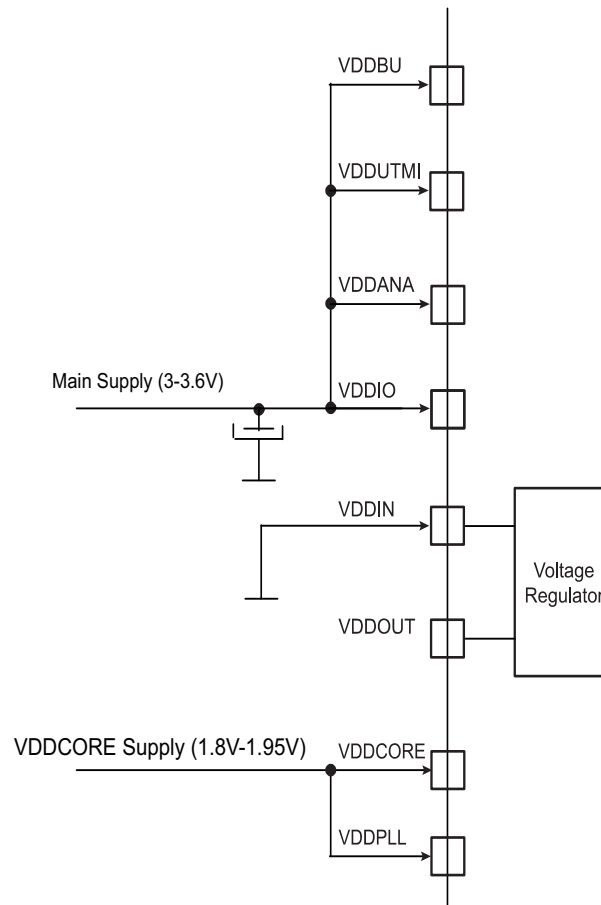
FIGURE 6-3: CORE EXTERNALLY SUPPLIED
