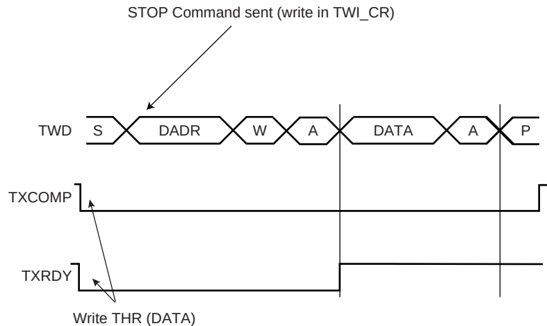
FIGURE 33-7: MASTER WRITE WITH ONE DATA BYTE
