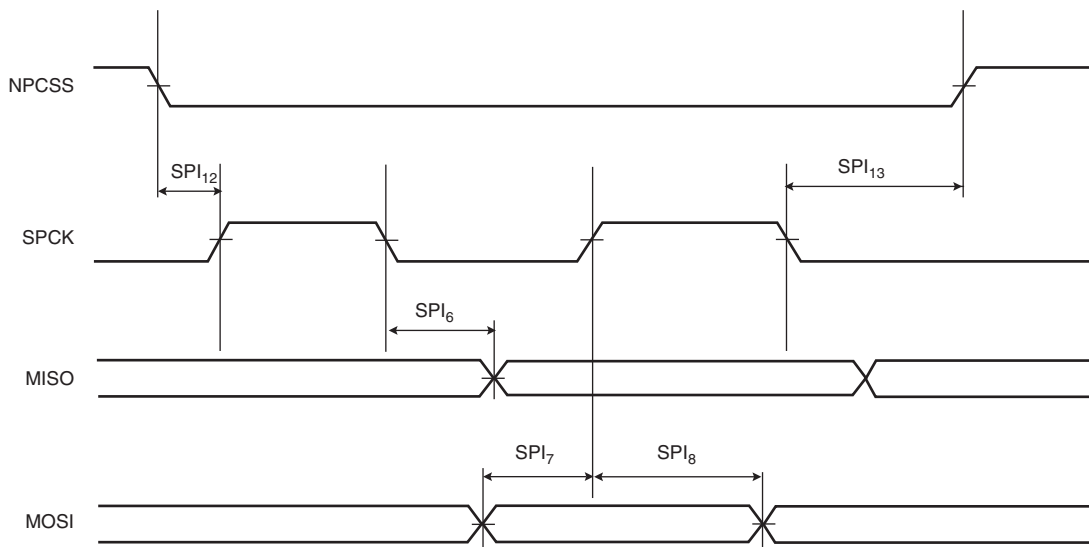
FIGURE 45-19: SPI SLAVE MODE WITH (CPOL = 0 AND NCPHA = 1) OR (CPOL = 1 AND NCPHA = 0)
