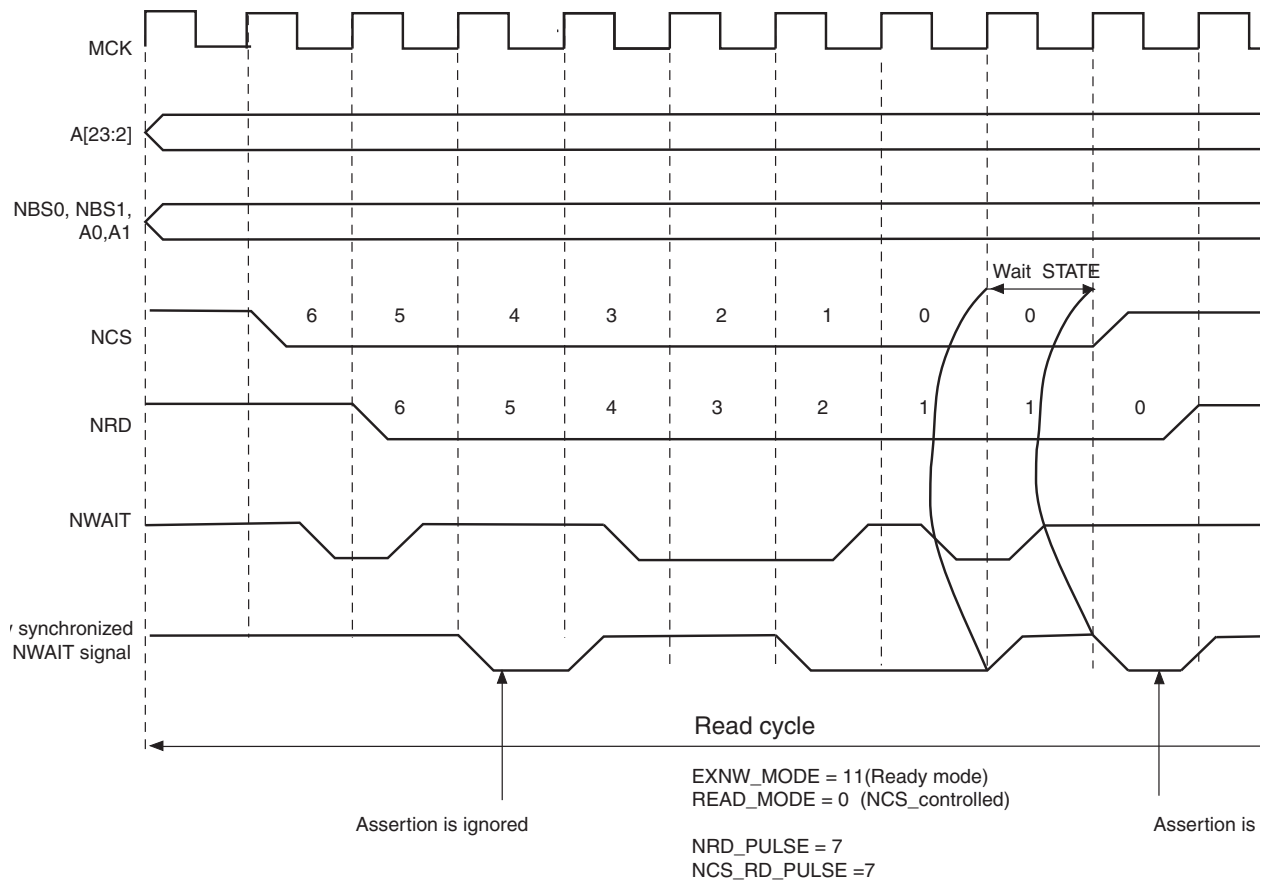
FIGURE 25-26: NWAIT ASSERTION IN READ ACCESS: READY MODE (EXNW_MODE = 11)
