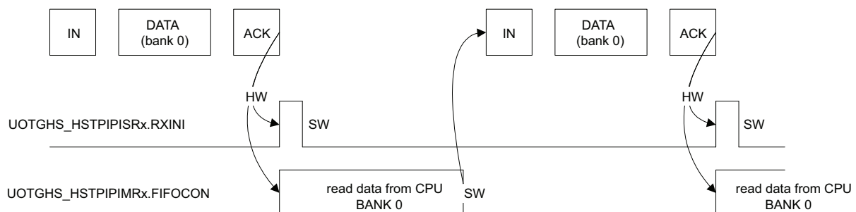
FIGURE 39-30: EXAMPLE OF AN IN PIPE WITH 1 DATA BANK
