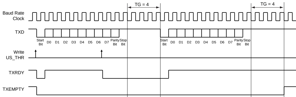
FIGURE 35-31: TIMEGUARD OPERATIONS
