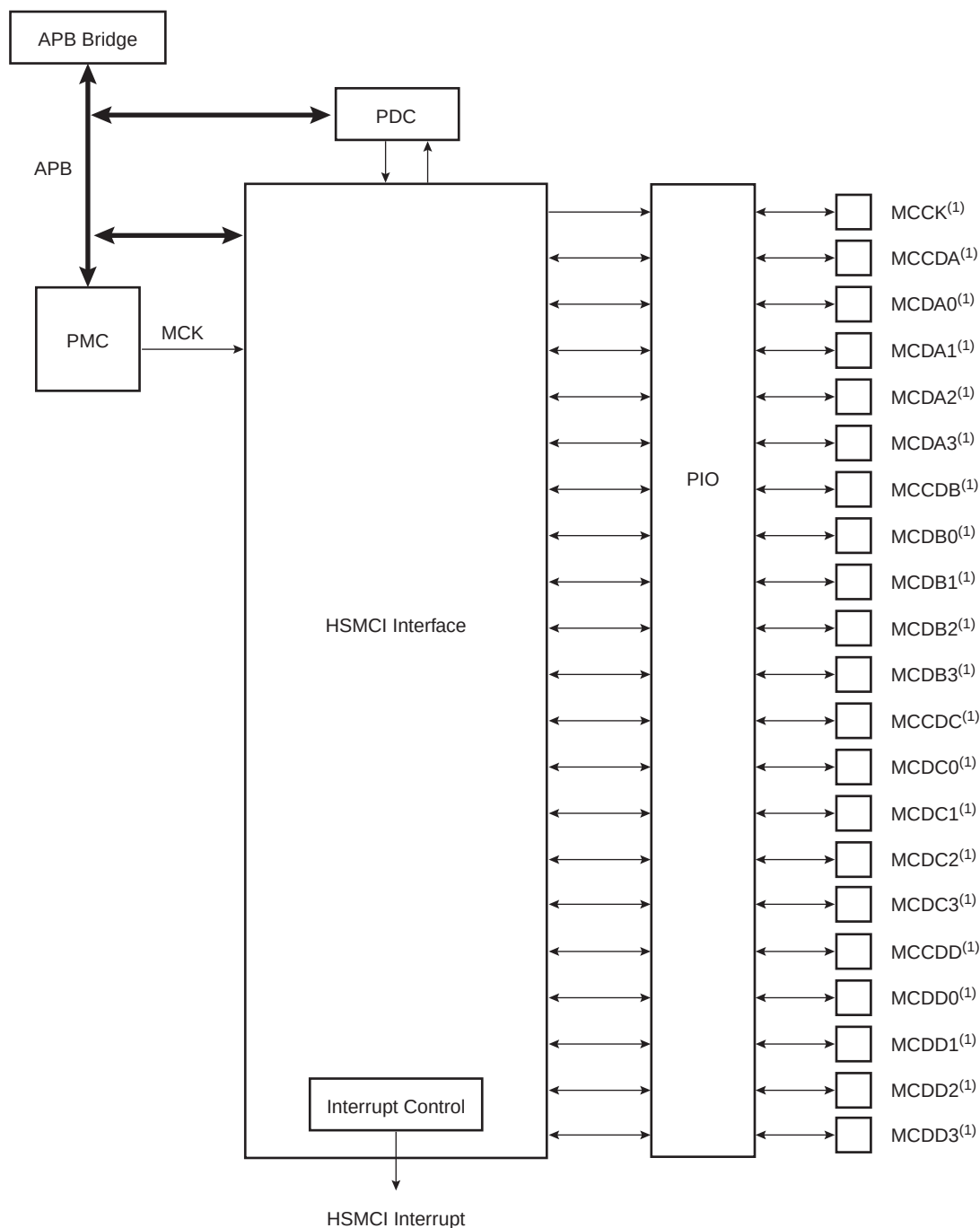
FIGURE 37-11: BLOCK DIAGRAM
