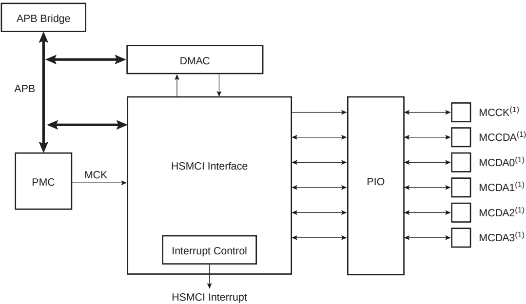
FIGURE 37-2: BLOCK DIAGRAM
