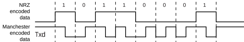
FIGURE 35-16: NRZ TO MANCHESTER ENCODING
