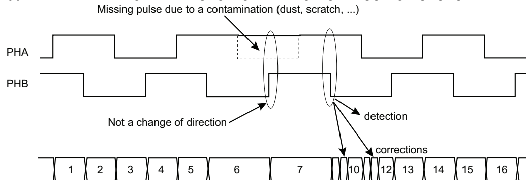
FIGURE 36-24: DETECTION AND AUTO-CORRECTION OF MISSING PULSES
