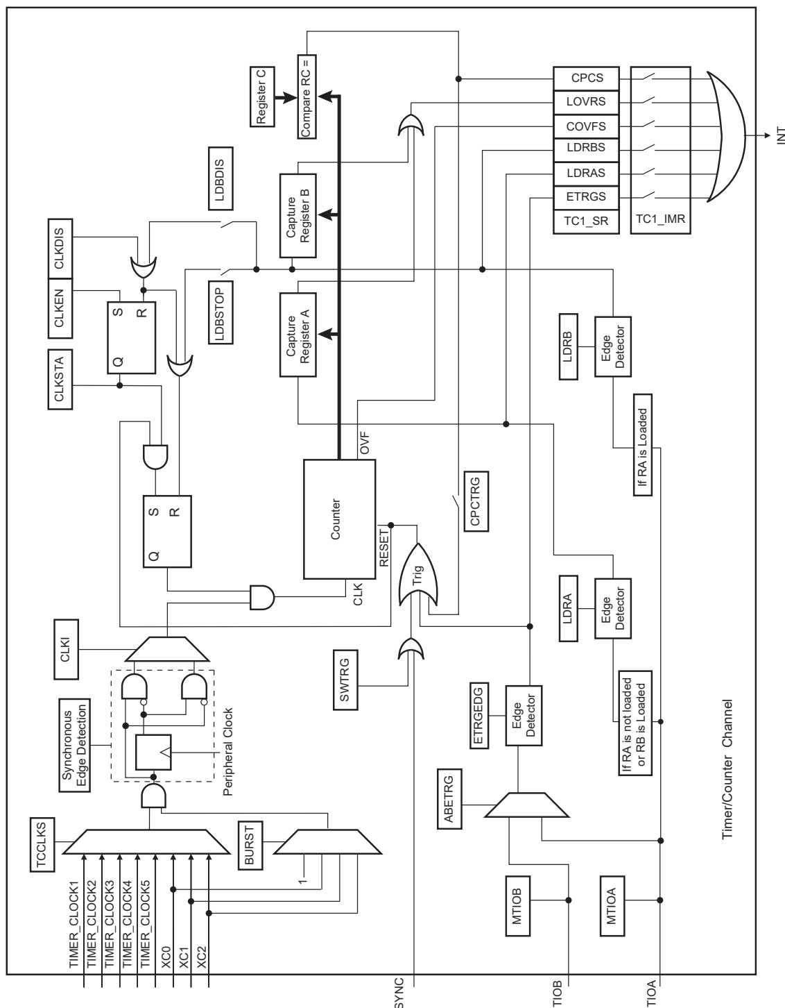
FIGURE 36-7: CAPTURE MODE
