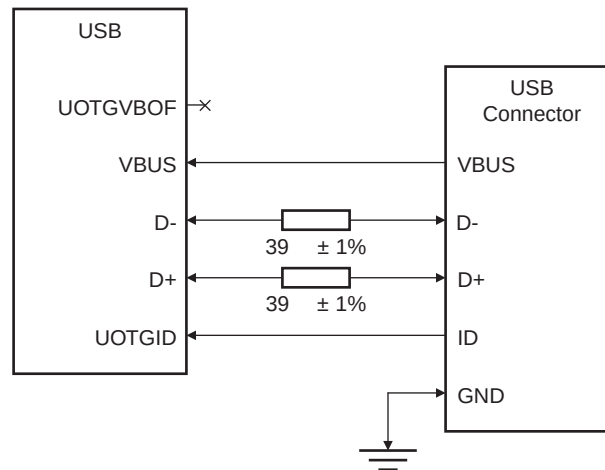
FIGURE 39-5: SELF-POWERED DEVICE APPLICATION BLOCK DIAGRAM
