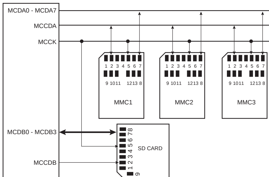
FIGURE 37-18: MIXING HIGH SPEED MULTIMEDIA AND SD MEMORY CARDS WITH TWO SLOTS
