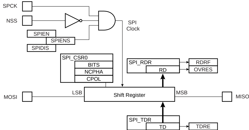
FIGURE 32-14: SLAVE MODE FUNCTIONAL BLOC DIAGRAM
