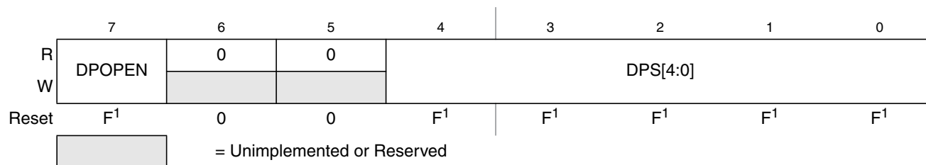
Figure 22-15. EEPROM Protection Register (EPROT)
