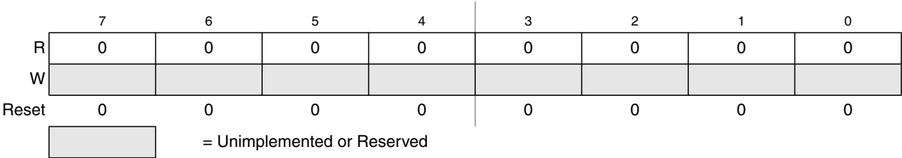
Figure 24-23. Flash Reserved5 Register (FRSV5)
