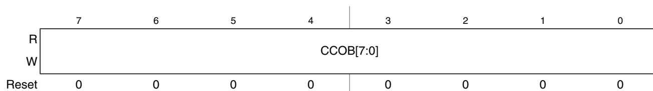
Figure 22-17. Flash Common Command Object Low Register (FCCOBLO)
