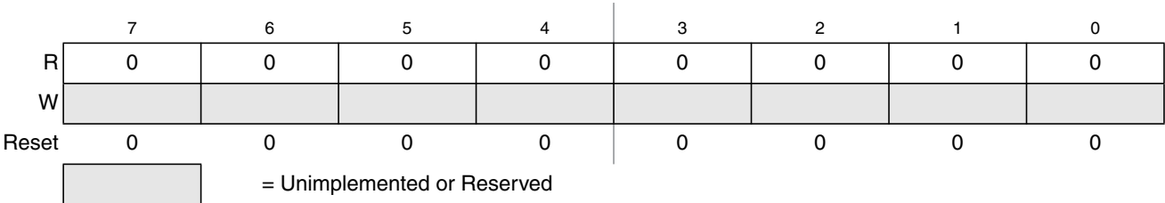
Figure 24-24. Flash Reserved6 Register (FRSV6)
