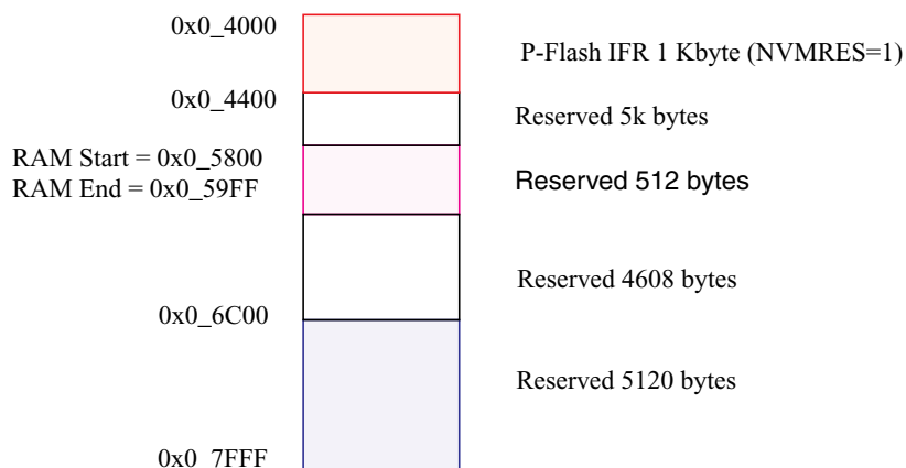
Figure 22-3. Memory Controller Resource Memory Map (NVMRES=1)
