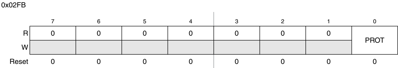
Figure 10-28. S12CPMU Protection Register (CPMUPROT)
