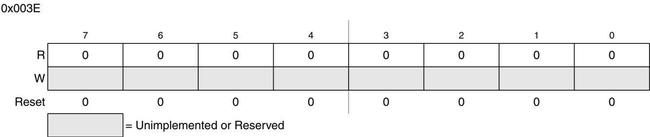
Figure 10-14. Reserved Register (CPMUTEST1)
