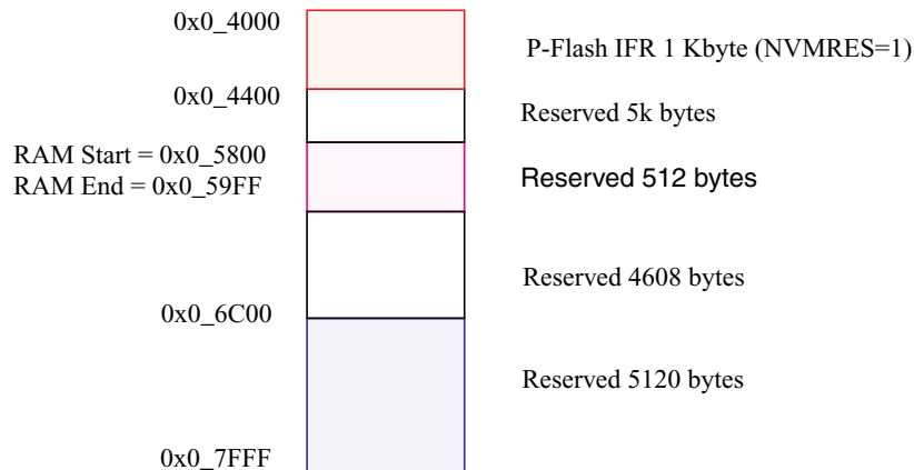
Figure 21-3. Memory Controller Resource Memory Map (NVMRES=1)
