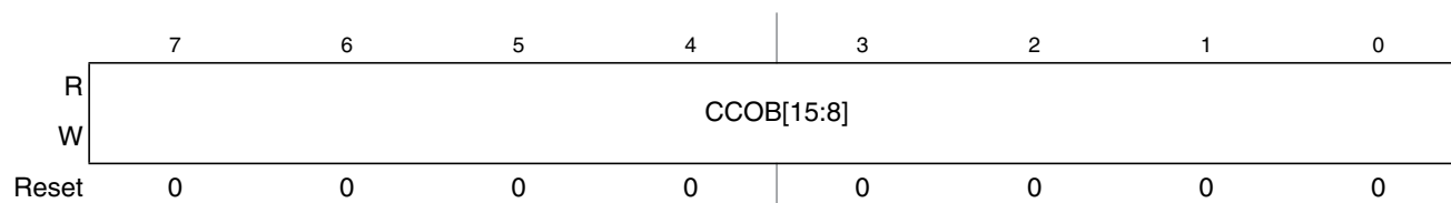
Figure 21-15. Flash Common Command Object High Register (FCCOBHI)
