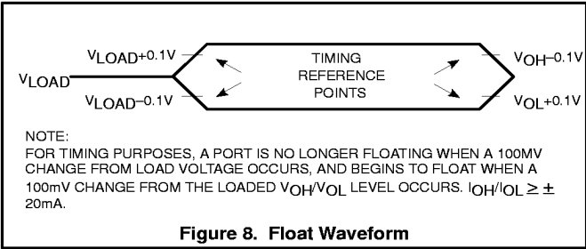
Figure 8. Float Waveform
