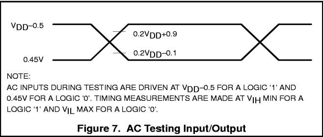
Figure 7. AC Testing Input/Output
