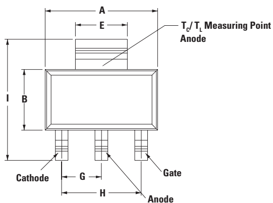
Dimensions – SOT-223
