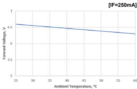
Fig 5. Forward Voltage vs Ambient Temperature
