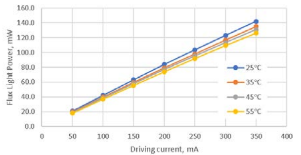
Fig 6. P-IF data vs SMD Temperature
