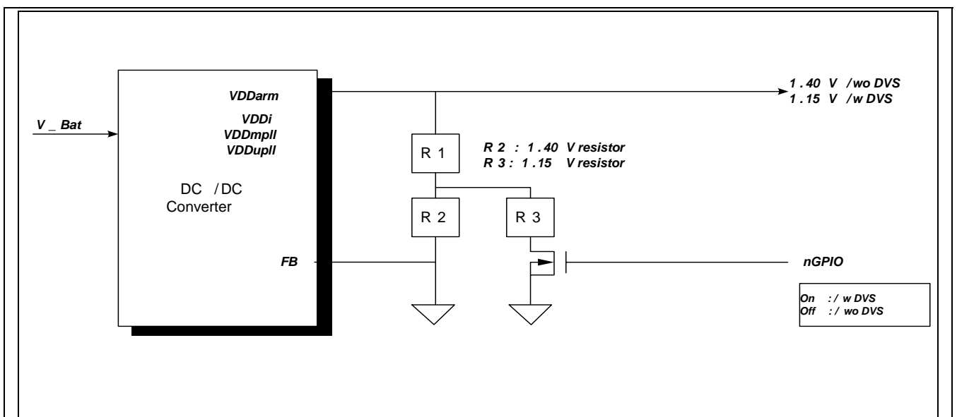
Figure 1-3. Power Scheme Diagram :266MHz
