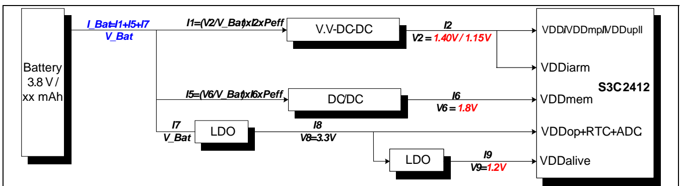
Figure 1-1. Power Scheme Diagram : 266MHz
