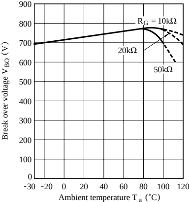
Fig. 6 Break Over Voltage vs. Ambient Temperature
